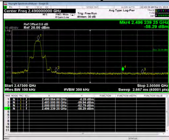
8DPSK,2480MHz,3DH5,Plot 1,Band Edge
