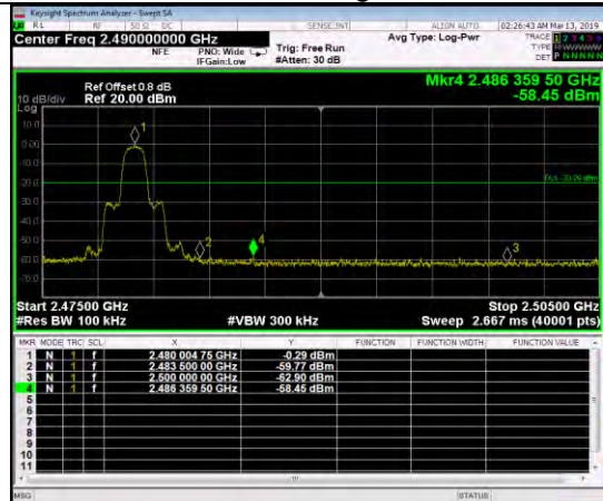
DQPSK,2480MHz,2DH5,Plot 1,Band Edge
