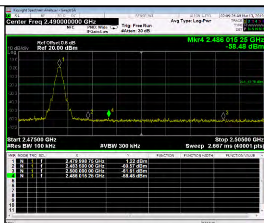
GFSK,2480MHz,DH5,Plot 1,Band Edge
