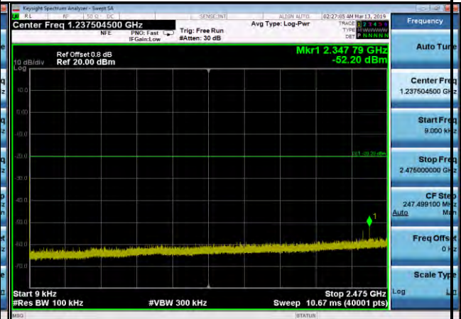
DQPSK,2480MHz,2DH5,Plot 2,0.009MHz~24 75MHz
