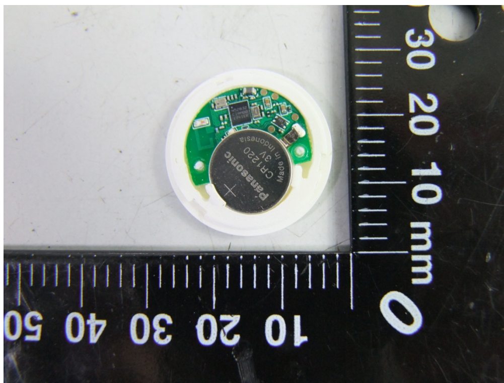
Photo 9 Inside of EUT (RIT-P02-RS)
