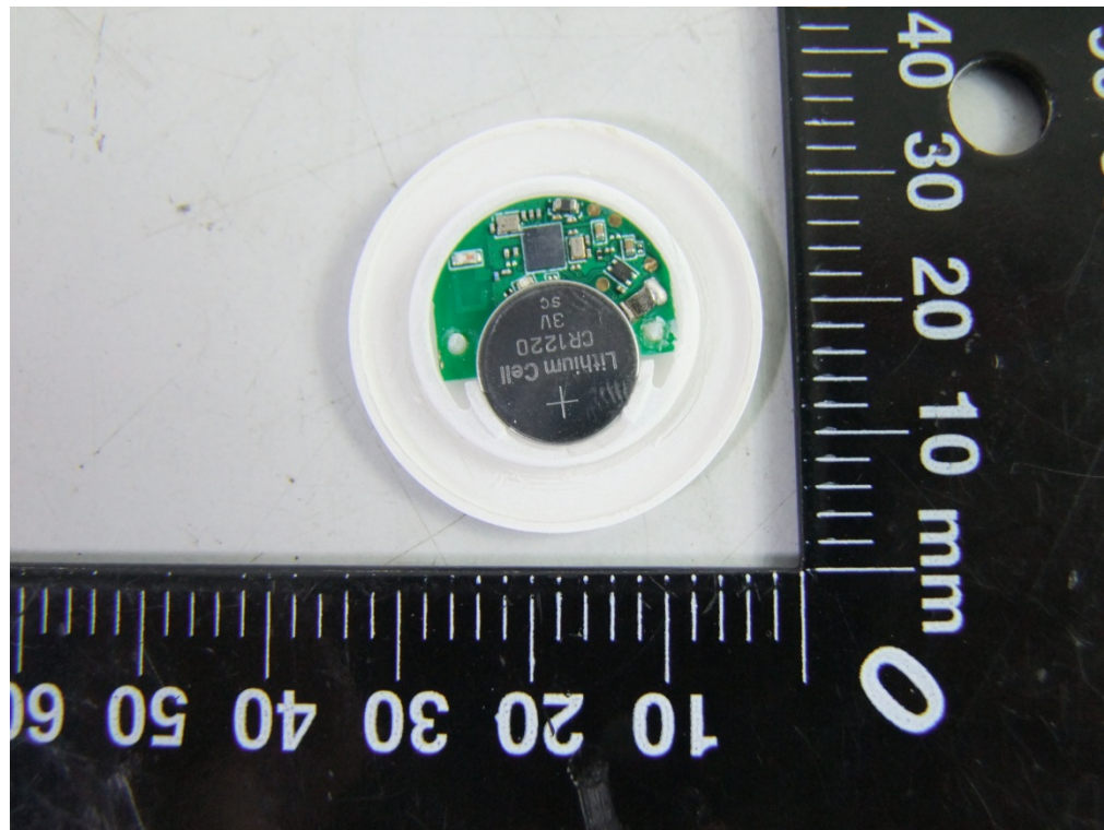
Photo 11 Inside of EUT (RIT-P02-R1)
