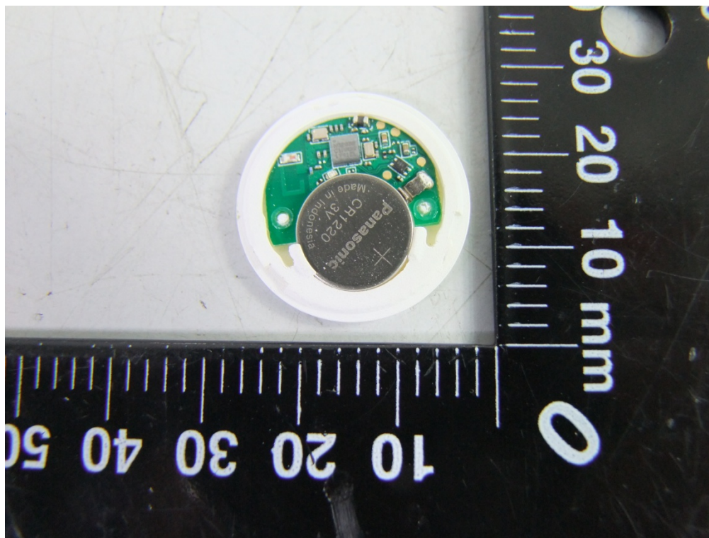
Photo 7 Inside of EUT (RIT-P02-RR)
