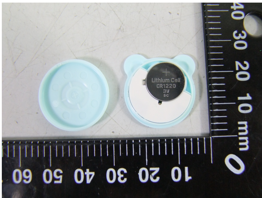
Photo 1 Inside of EUT (RIT-P02-MED)
