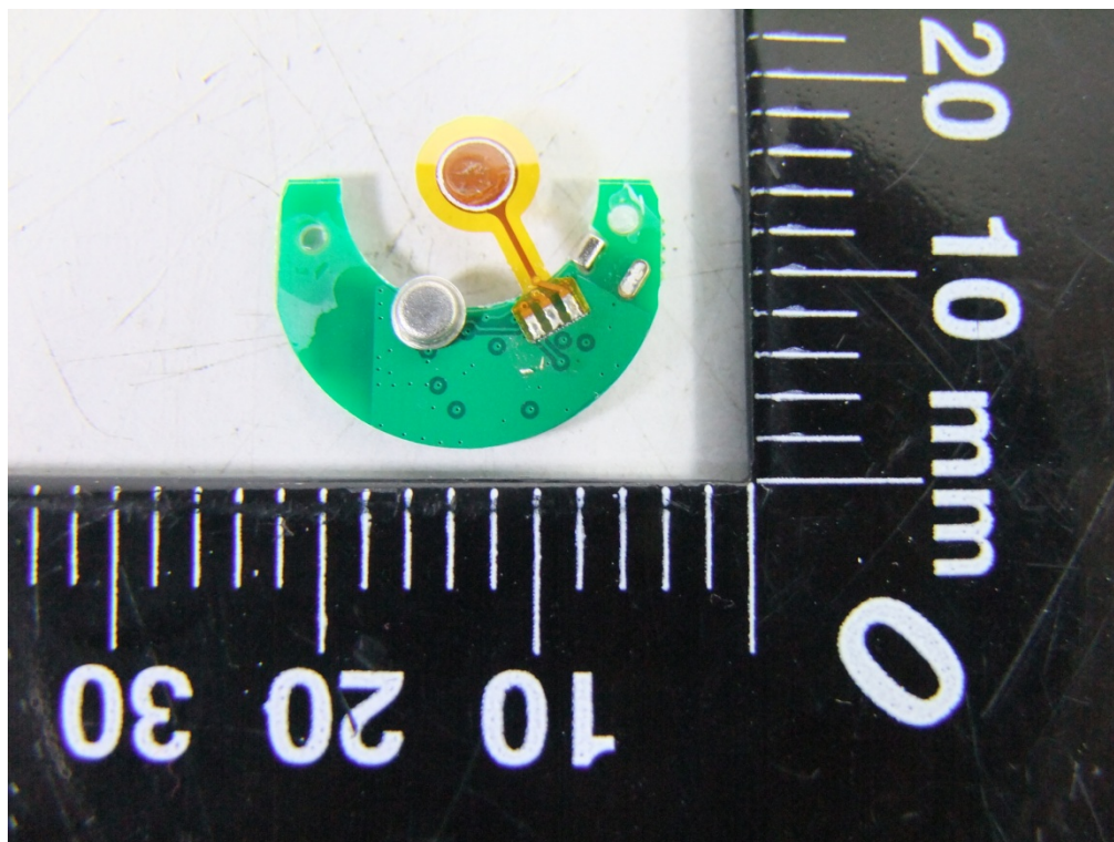
Photo 4 Inside of EUT (RIT-P02-MED)
