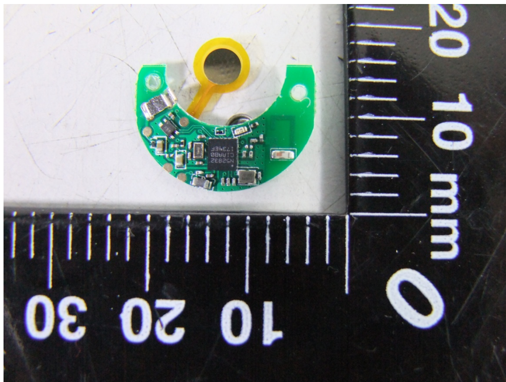
Photo 3 Inside of EUT (RIT-P02-MED)
