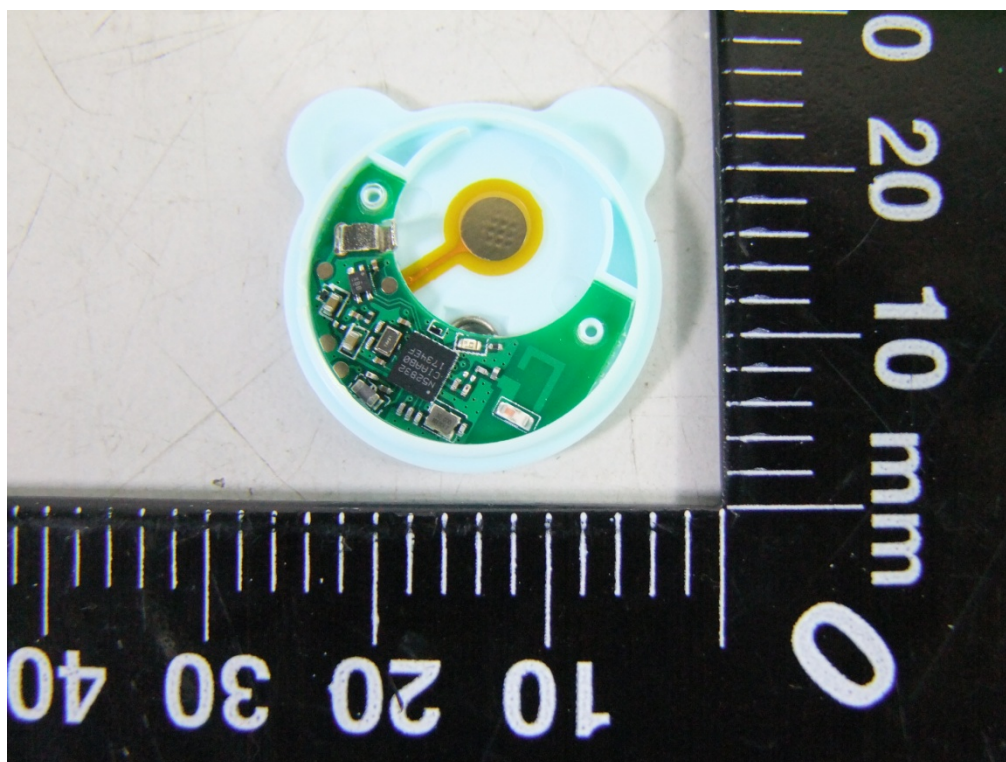
Photo 2 Inside of EUT (RIT-P02-MED)
