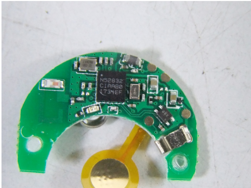
Photo 5 Inside of EUT (RIT-P02-MED)
