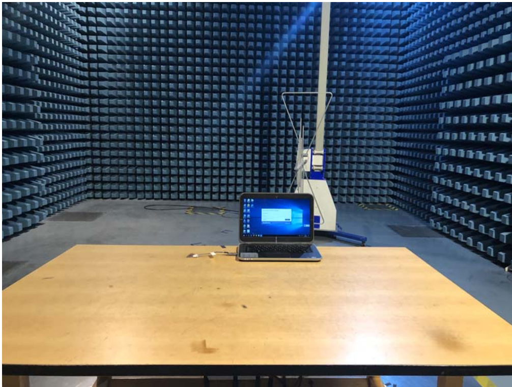
FCC Part15C Radiated Emission below 1GHz
