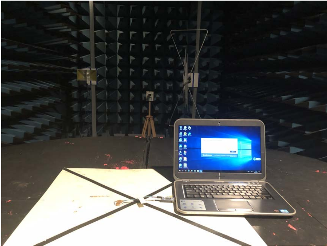
FCC Part15C Radiated Emission 18-26.5GHz
