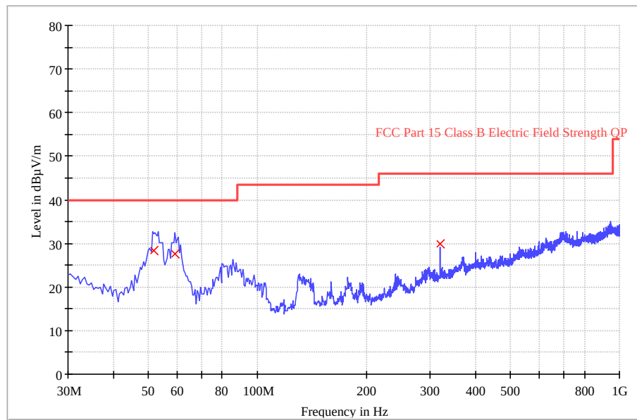
FCC Part 15
