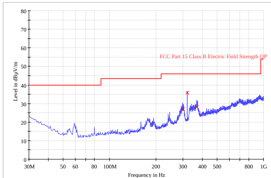
FCC Part 15
