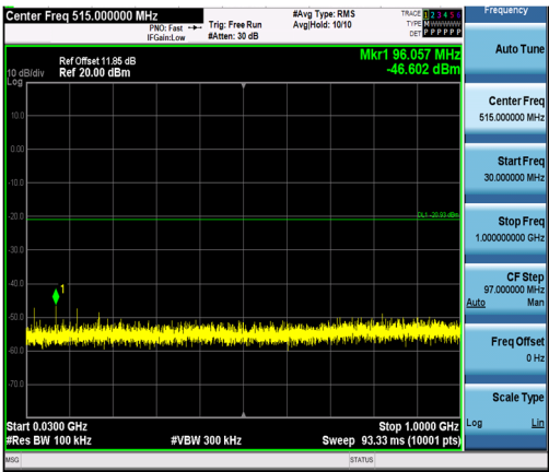
3DH5-Ant1-2402-30~1000-PASS
