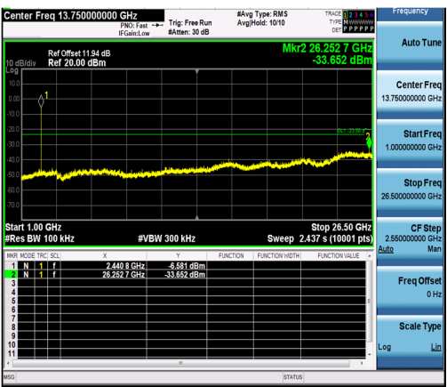
2DH5-Ant1-2441-1000~26500-PASS
