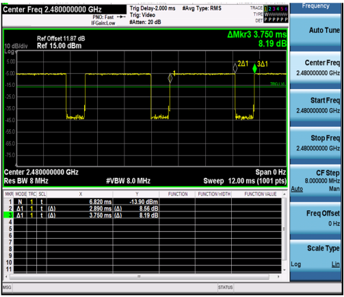
NTNV-3DH5-Ant1-2480
