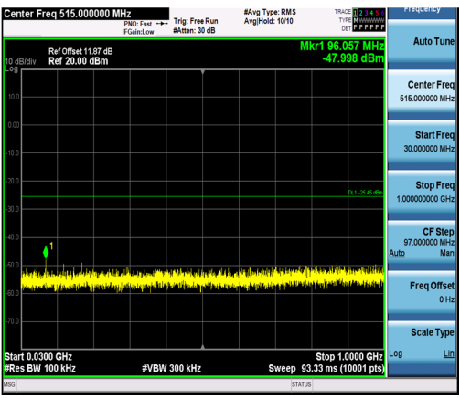
2DH5-Ant1-2480-30~1000-PASS
