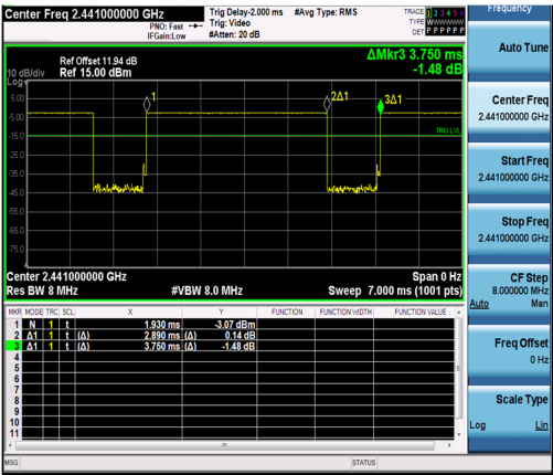
NTNV-DH5-Ant1-2441
