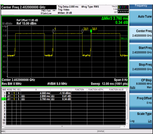
NTNV-DH5-Ant1-2402
