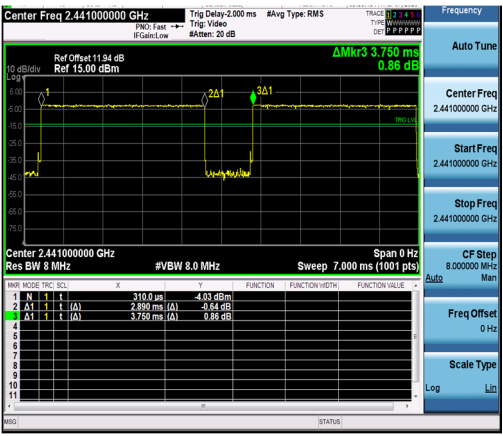
NTNV-3DH5-Ant1-2441
