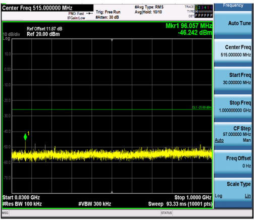
3DH5-Ant1-2480-30~1000-PASS
