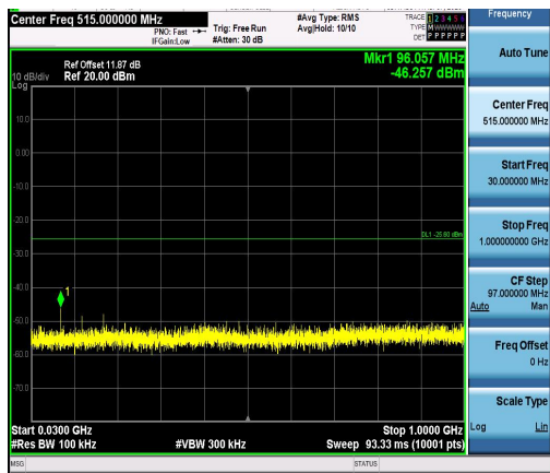
2DH5-Ant1-2480-30~1000-PASS
