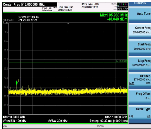
2DH5-Ant1-2441-30~1000-PASS
