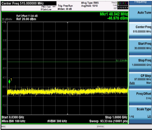
DH5-Ant1-2441-30~1000-PASS
