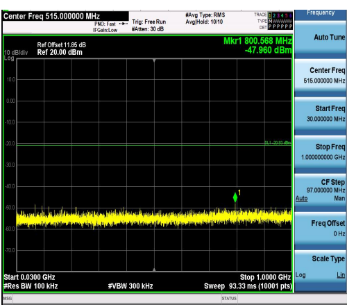
DH5-Ant1-2402-30~1000-PASS
