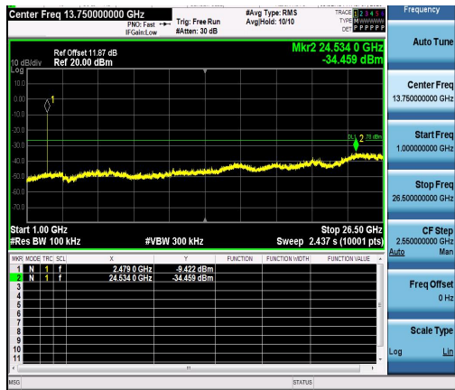
3DH5-Ant1-2480-1000~26500-PASS
