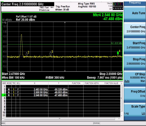
DH5-Ant1-2480-PASS
