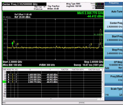
2DH5-Ant1-2402-PASS
