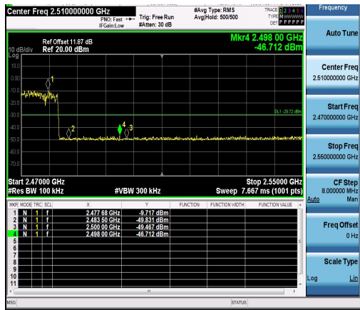
3DH5-Ant1-Hop_2480-PASS
