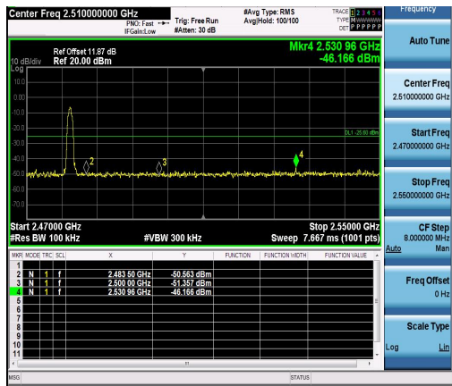
2DH5-Ant1-2480-PASS
