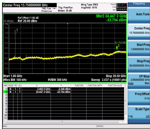
3DH5-Ant1-2402-1000~26500-PASS
