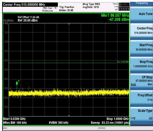
3DH5-Ant1-2441-30~1000-PASS
