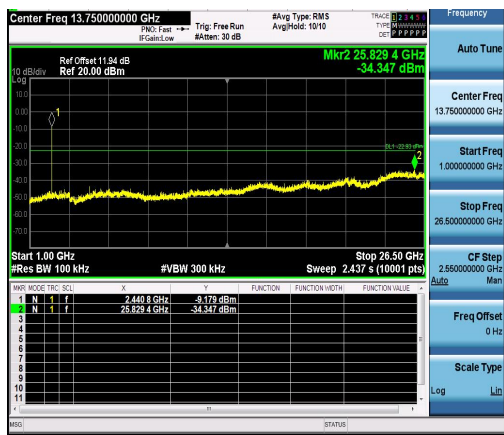
3DH5-Ant1-2441-1000~26500-PASS
