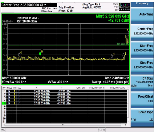
DH5-Ant1-Hop_2402-PASS
