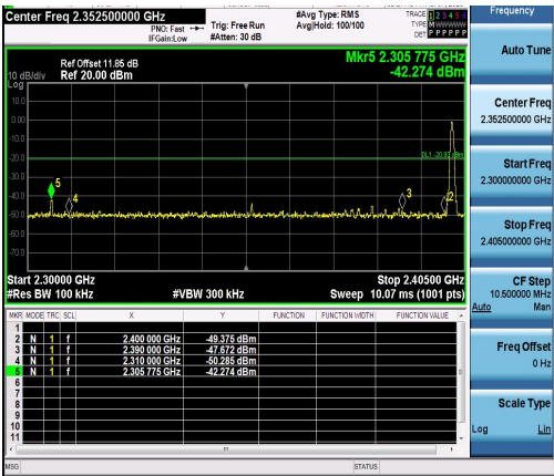
DH5-Ant1-2402-PASS
