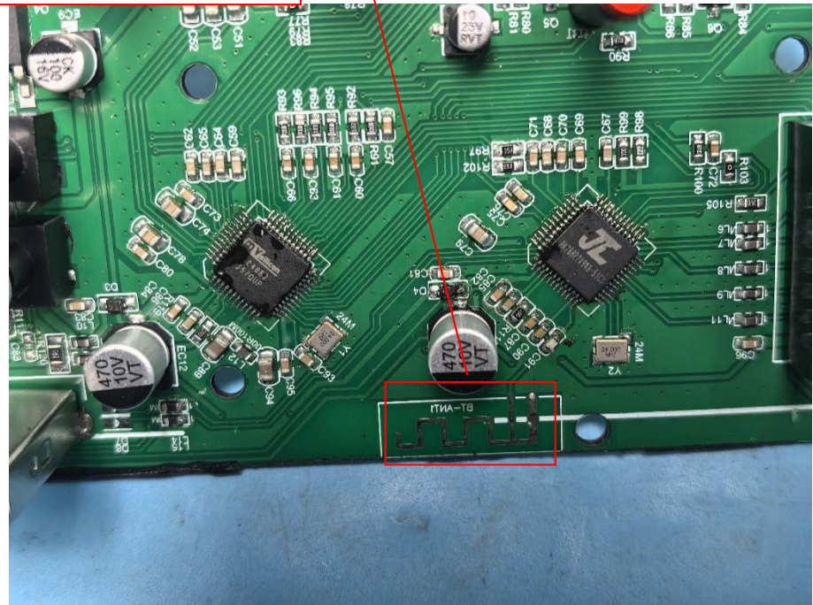
Bluetooth Antenna
