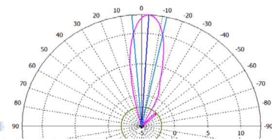
Elevation beam pattern
