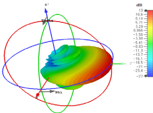
Without Radome
