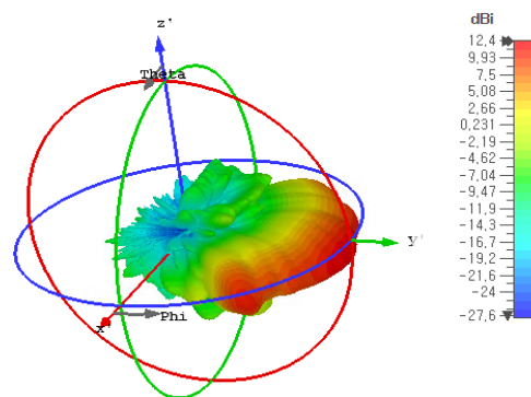
With Radome
