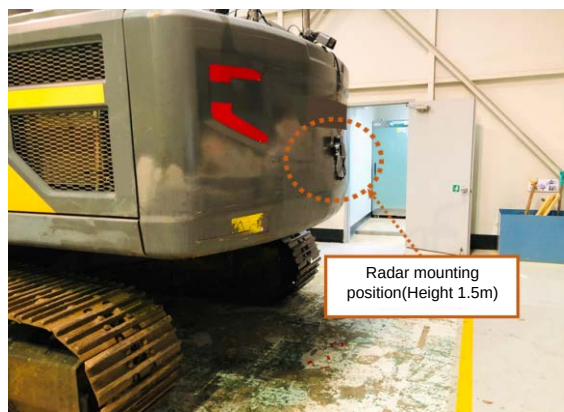
Mount on an excavator(For Example)
