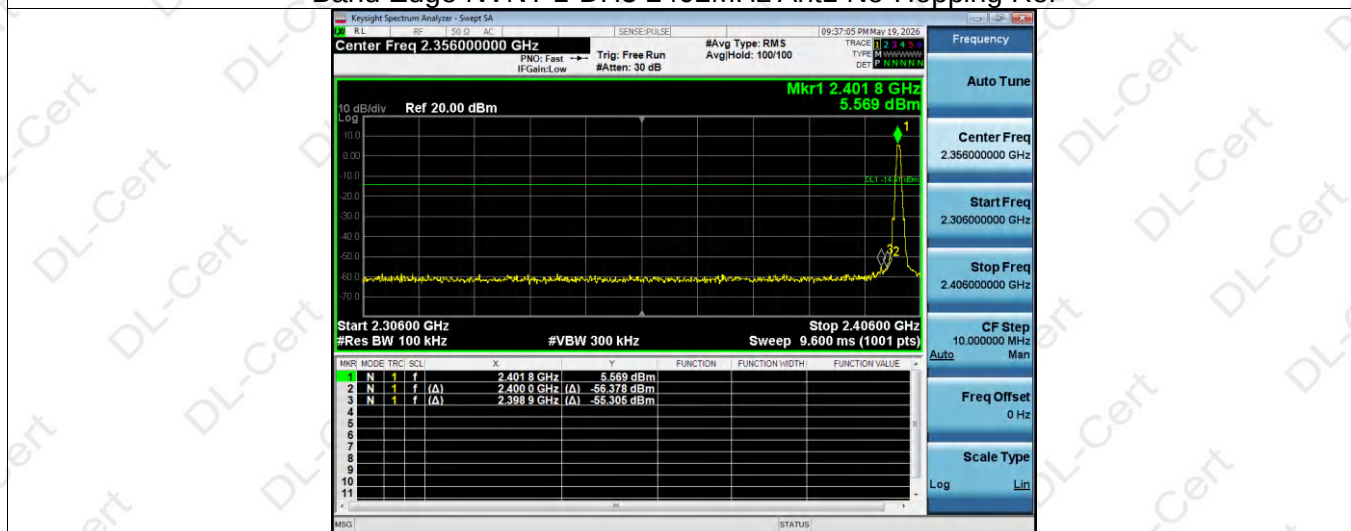
Band Edge NVNT 1-DH5 2402MHz Ant1 No-Hopping Emission
