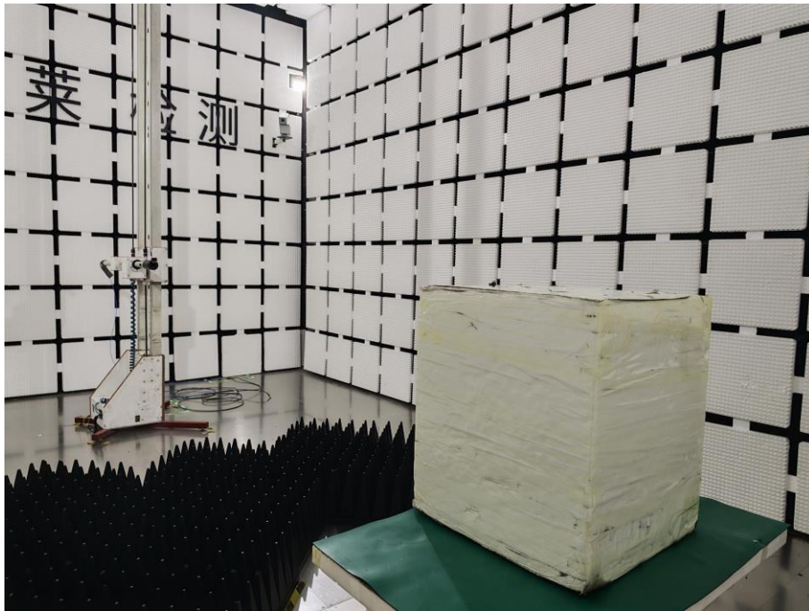
Radiated Measurement Photos(18GHz-25GHz)
