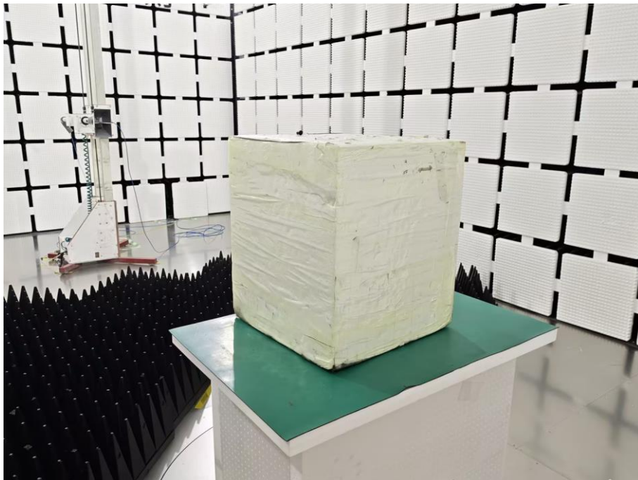
Radiated Measurement Photos(1GHz-18GHz)
