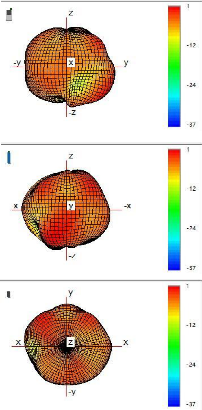
9-1.3D Gain Pattern (Radiation Pattern at 2450 MHz)
