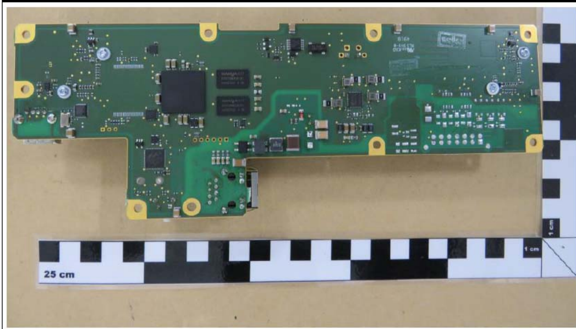
PCB back
