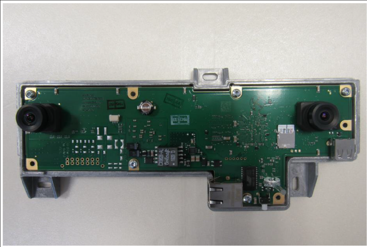
EUT PCB FRONT
