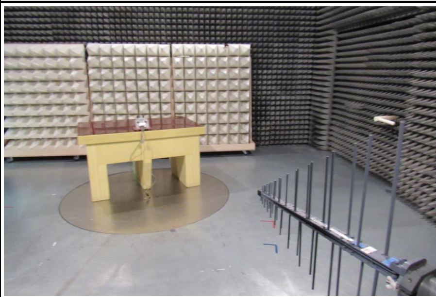
TEST SETUP-2 EUT CONFIGURATION-1 RE
