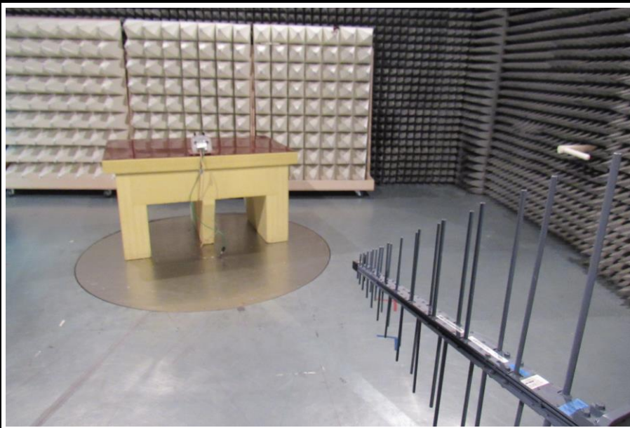
TEST SETUP-2 EUT CONFIGURATION-2 RADIATED EMISSION
