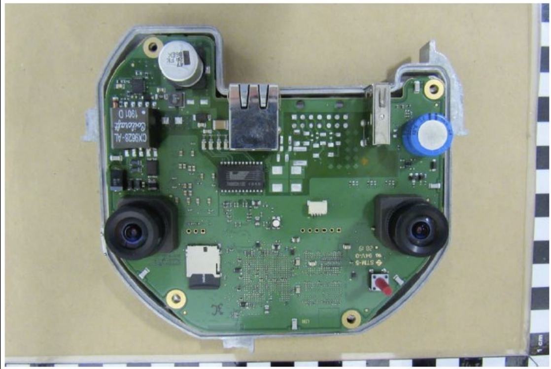
EUT FRONT SIDE WITHOUT CASE
