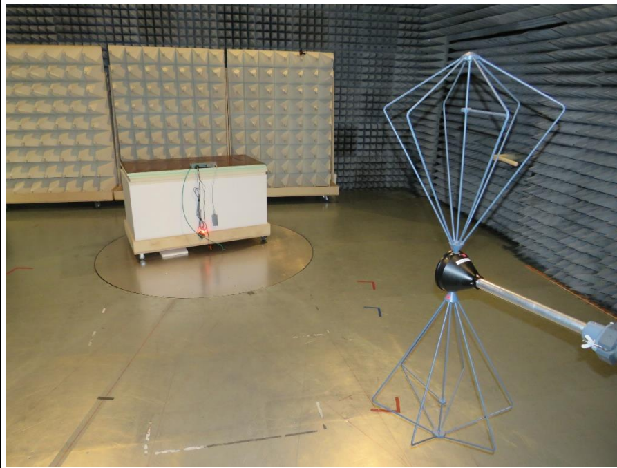
RADIATED EMSSION: 30MHz - 200MHz
