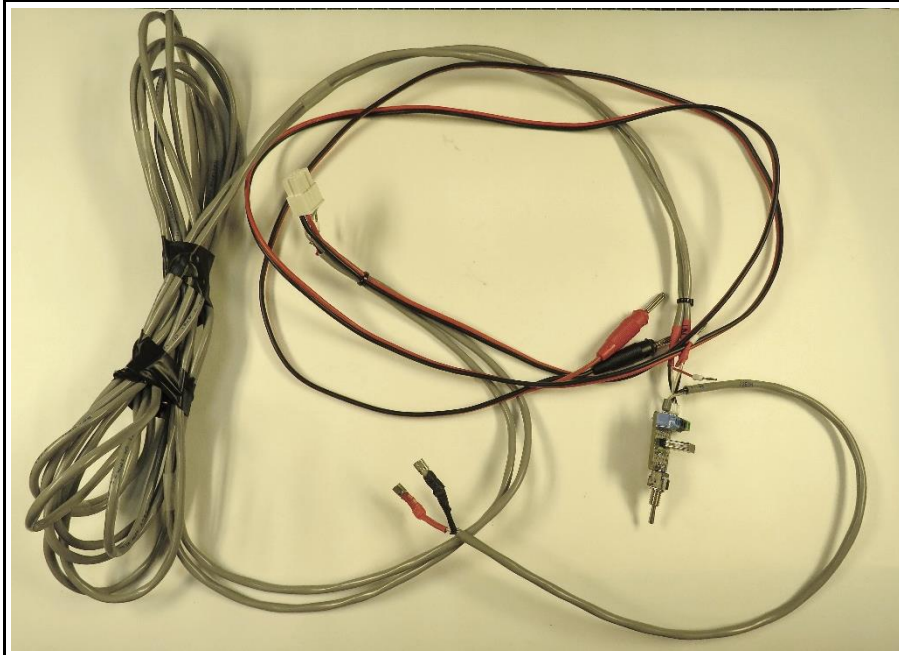
EUT – Cable for multi purpose connector incl. LED driver board and DC-connectors (4mm banana plugs)
