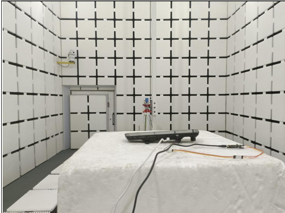
RADIATED EMISSION TEST (1-18GHz)
