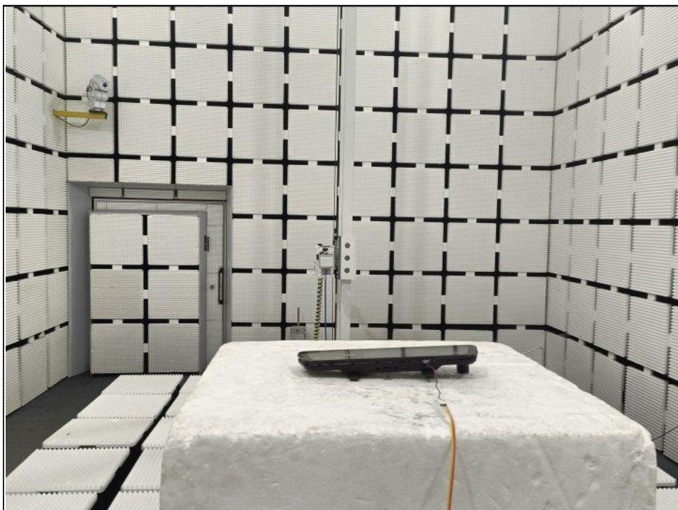
RADIATED EMISSION TEST (18-40GHz)
