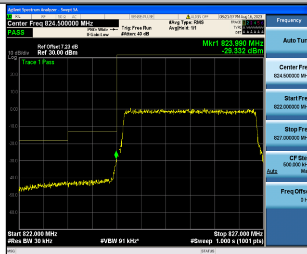
Band5_3MHz_QPSK_20415_15RB#0
