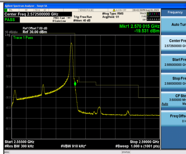
Band7_15MHz_QPSK_21375_1RB#74
