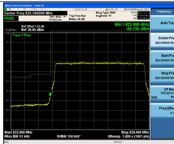
Band5_5MHz_QPSK_20425_25RB#0
