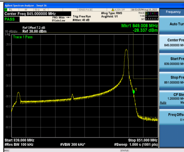
Band5_10MHz_QPSK_20600_1RB#49
