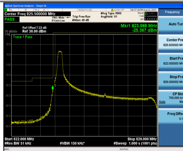
Band5_5MHz_QPSK_20425_1RB#0
