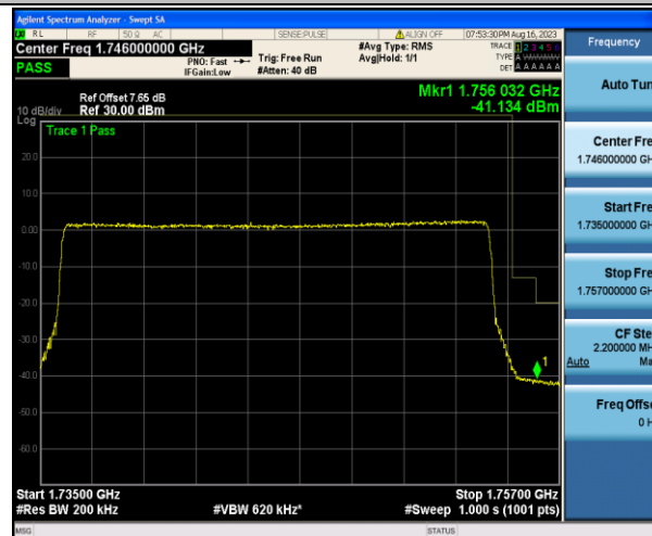
Band4_20MHz_QPSK_20300_100RB#0
