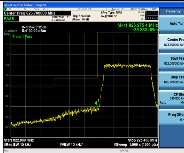
Band5_1.4MHz_QPSK_20407_6RB#0
