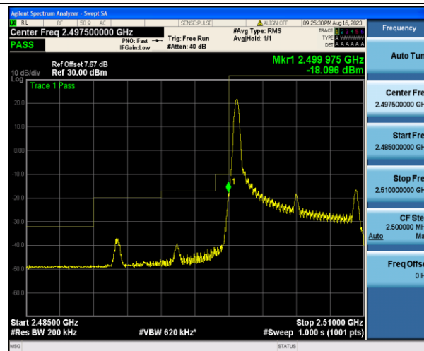
Band7_10MHz_16QAM_20800_1RB#0
