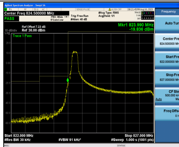
Band5_3MHz_QPSK_20415_1RB#0
