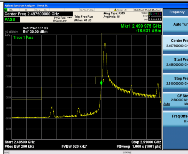
Band7_10MHz_QPSK_20800_1RB#0
