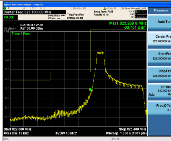
Band5_1.4MHz_16QAM_20407_1RB#0
