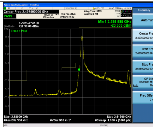
Band7_15MHz_16QAM_20825_1RB#0
