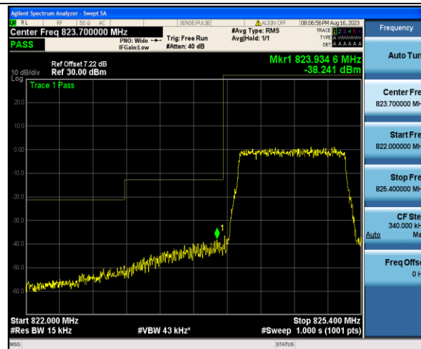
Band5_1.4MHz_16QAM_20407_6RB#0
