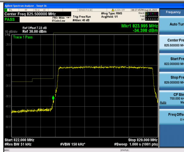
Band5_5MHz_16QAM_20425_25RB#0
