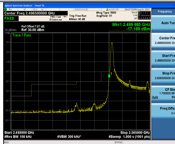
Band7_5MHz_16QAM_20775_1RB#0
