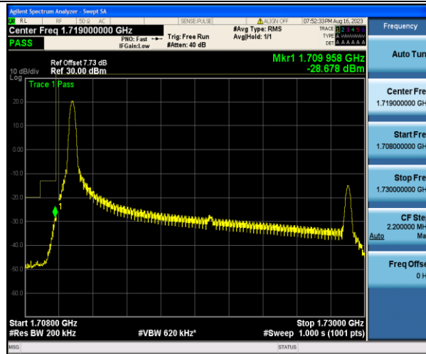
Band4_20MHz_QPSK_20050_1RB#0
