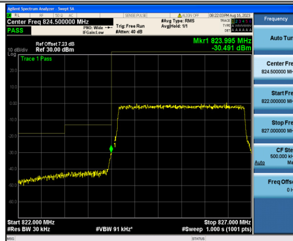
Band5_3MHz_16QAM_20415_15RB#0
