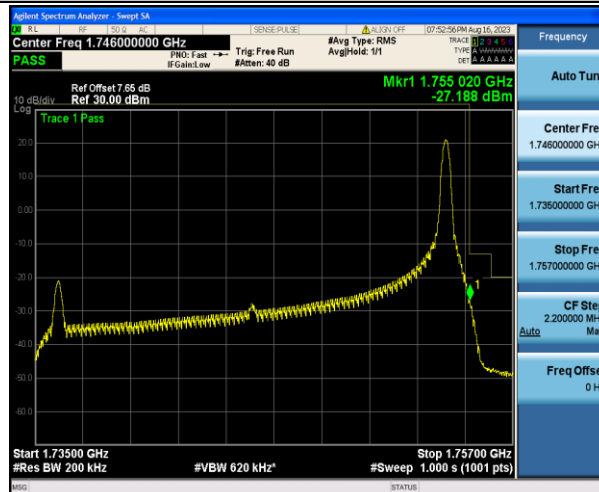
Band4_20MHz_QPSK_20300_1RB#99
