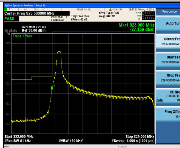
Band5_5MHz_16QAM_20425_1RB#0
