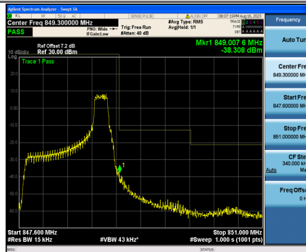
Band5_1.4MHz_16QAM_20643_1RB#5
