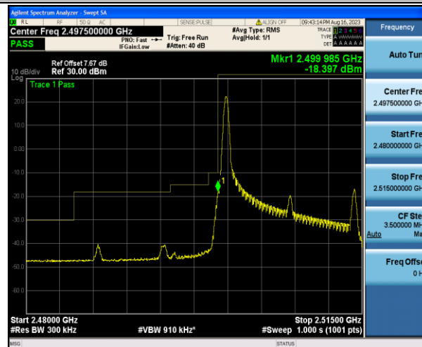
Band7_15MHz_QPSK_20825_1RB#0
