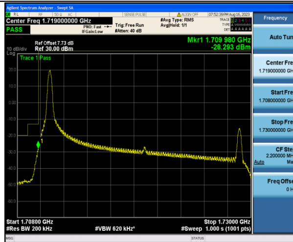
Band4_20MHz_16QAM_20050_1RB#0
