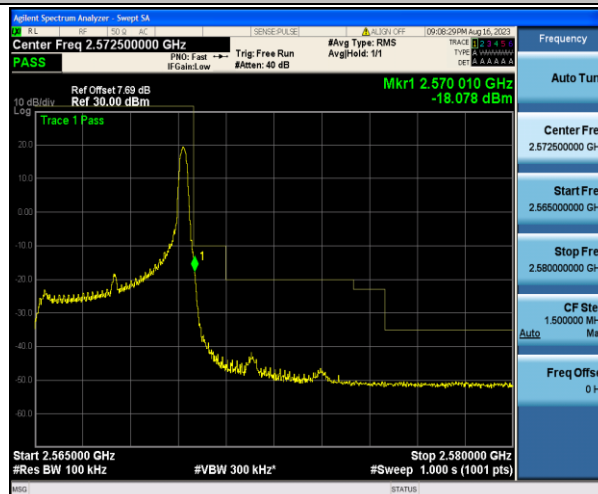
Band7_5MHz_16QAM_21425_1RB#24
