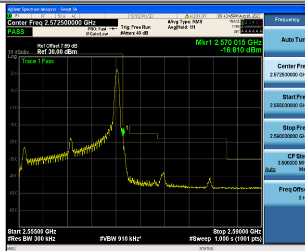
Band7_15MHz_16QAM_21375_1RB#74
