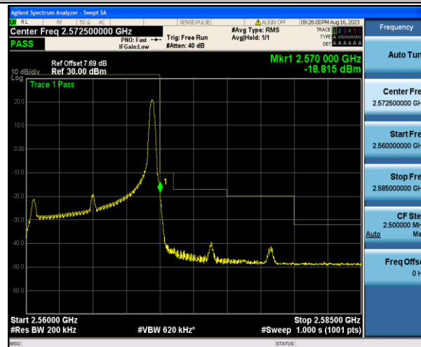
Band7_10MHz_16QAM_21400_1RB#49
