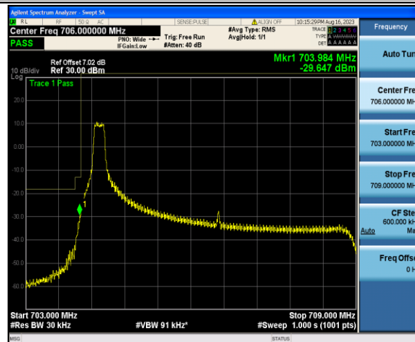
Band17_5MHz_QPSK_23755_1RB#0
