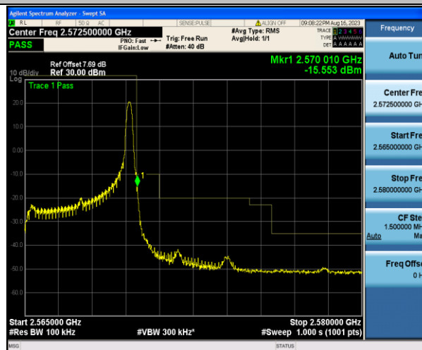
Band7_5MHz_QPSK_21425_1RB#24
