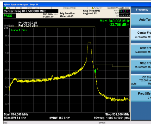
Band5_5MHz_QPSK_20625_1RB#24
