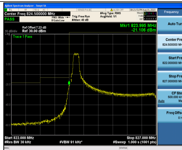
Band5_3MHz_16QAM_20415_1RB#0
