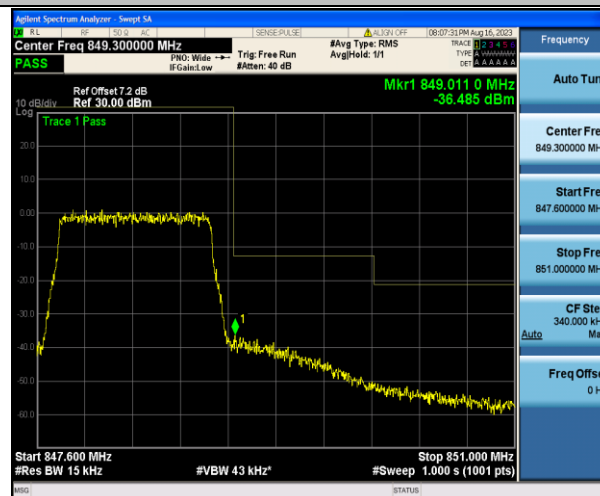
Band5_1.4MHz_16QAM_20643_6RB#0
