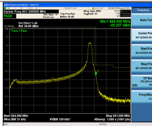
Band5_5MHz_16QAM_20625_1RB#24
