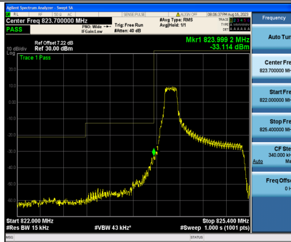
Band5_1.4MHz_QPSK_20407_1RB#0
