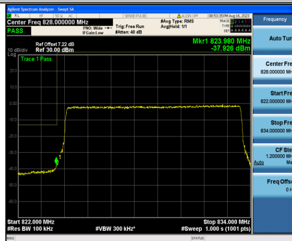
Band5_10MHz_QPSK_20450_50RB#0
