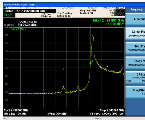
Band7_5MHz_QPSK_20775_1RB#0
