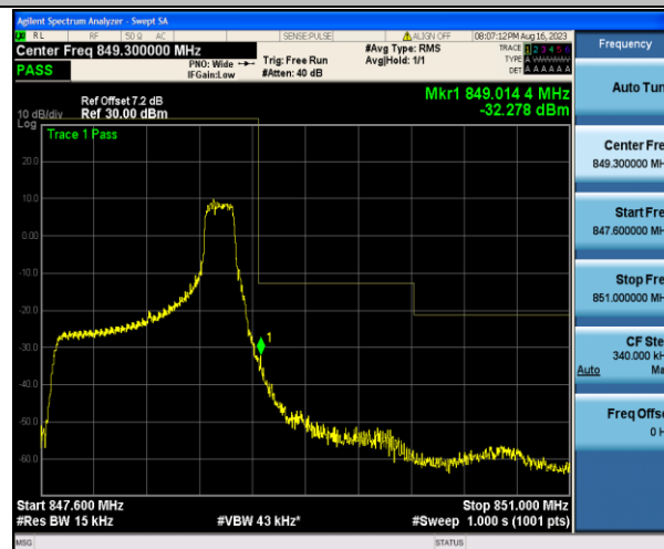
Band5_1.4MHz_QPSK_20643_1RB#5
