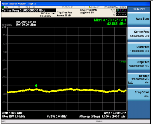
Band17_10MHz_QPSK_23800_1RB#0_1000~10000_1000~10000
