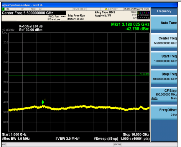
Band17_10MHz_16QAM_23800_1RB#0_1000~10000_1000~10000
