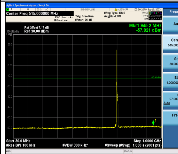
Band17_10MHz_16QAM_23800_1RB#0_30~1000_30~1000
