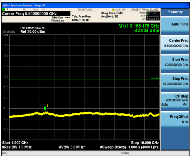
Band17_10MHz_16QAM_23790_1RB#0_1000~10000_1000~10000
