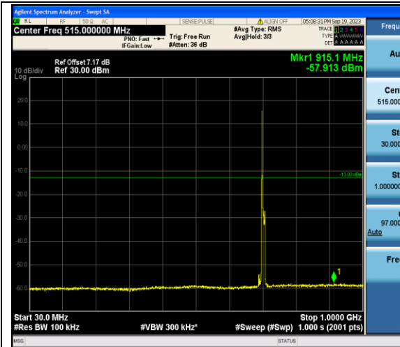
Band17_10MHz_16QAM_23790_1RB#0_30~1000_30~1000
