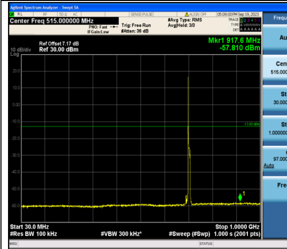
Band17_10MHz_QPSK_23800_1RB#0_30~1000_30~1000
