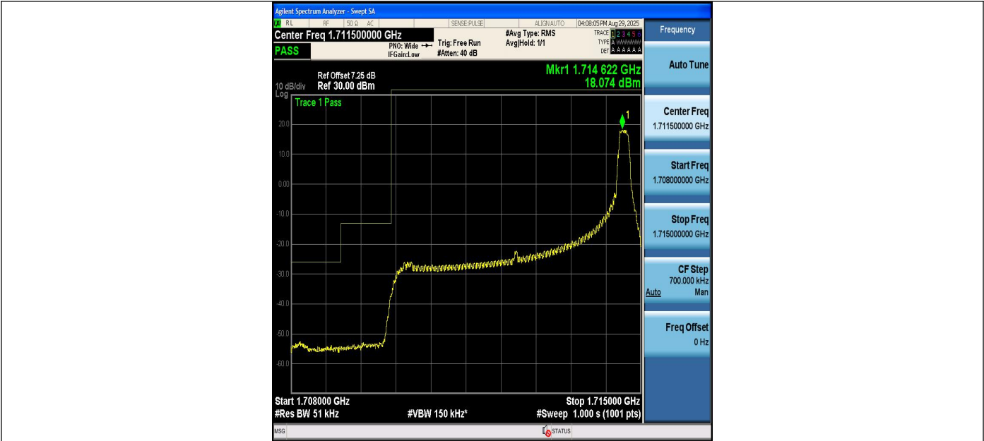
Band4_5MHz_QPSK_19975_1RB#24
