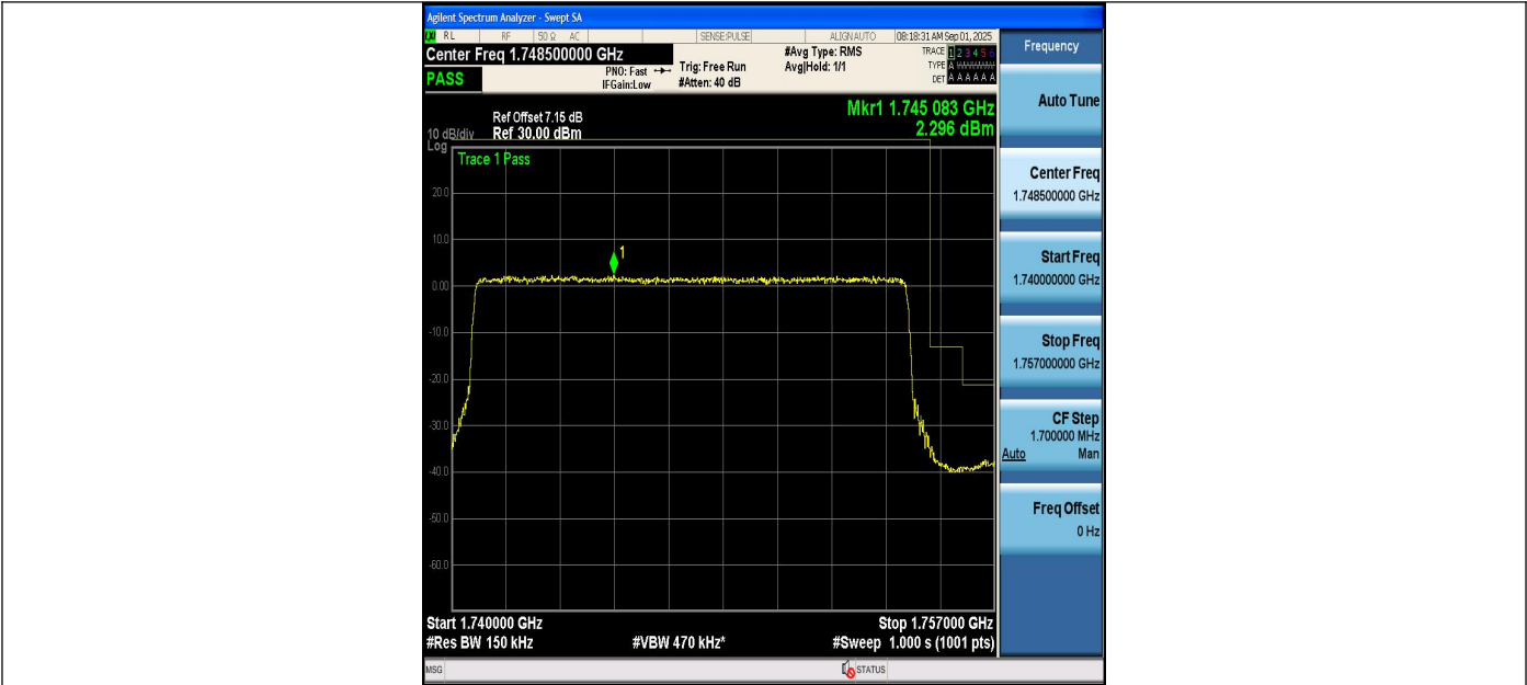
Band4_15MHz_QPSK_20325_75RB#0
