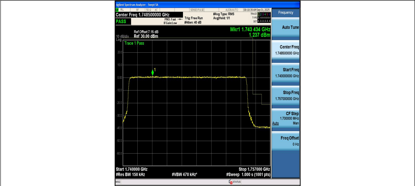
Band4_15MHz_16QAM_20325_75RB#0
