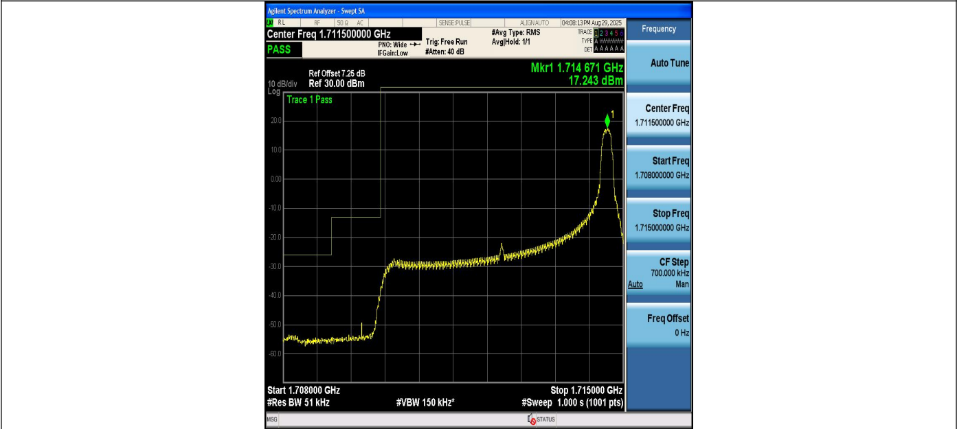
Band4_5MHz_16QAM_19975_1RB#24
