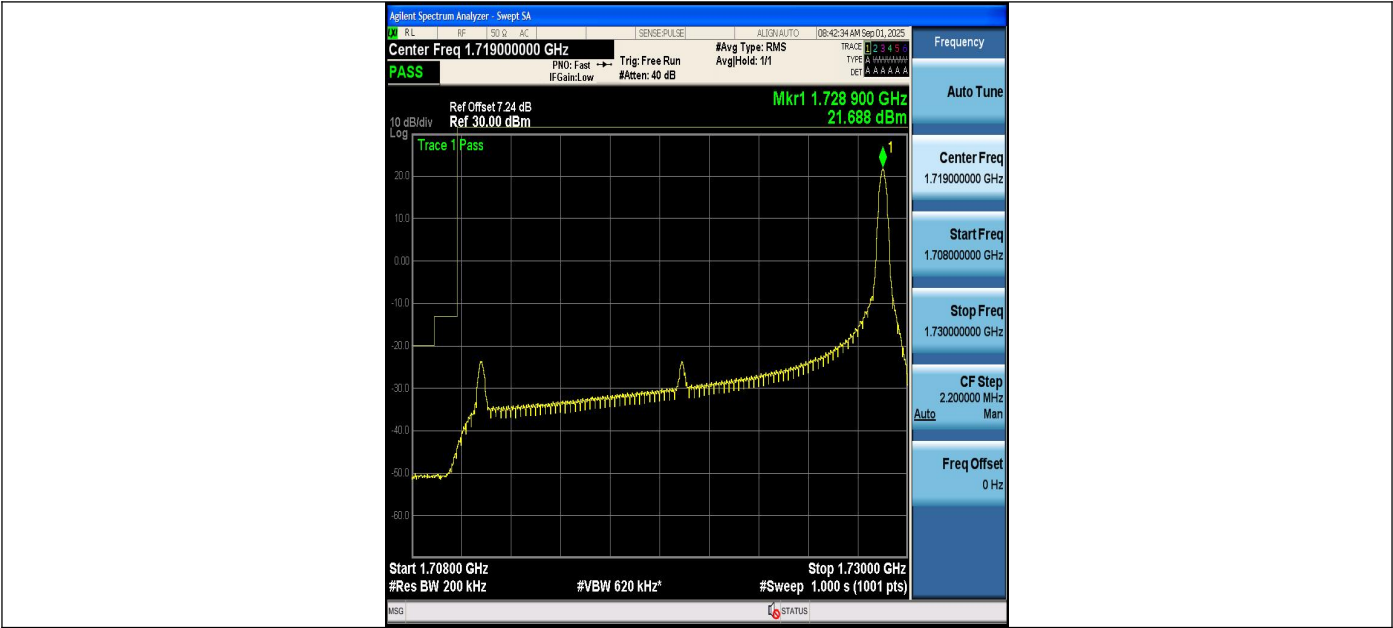
Band4_20MHz_QPSK_20050_1RB#99
