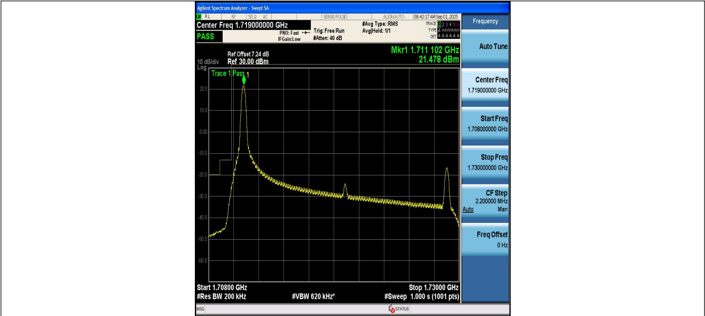
Band4_20MHz_QPSK_20050_1RB#0
