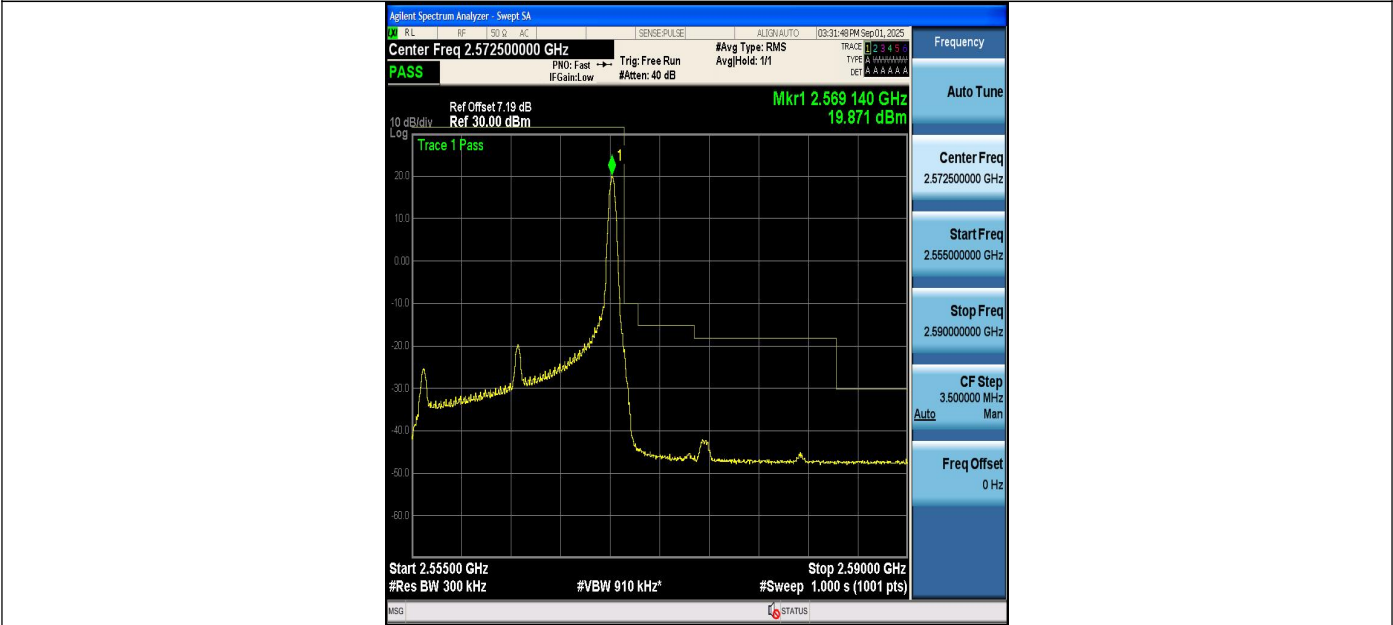
Band7_15MHz_16QAM_21375_1RB#74
