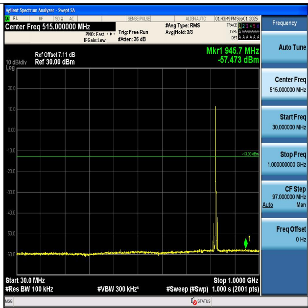
Band5 5MHz QPSK 20425 1RB#0 30~1000 30~1000
