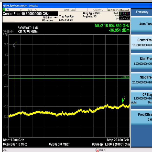
Band2-9400-1000~20000MHz-PASS
