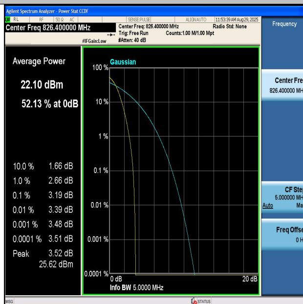
Band5-4132-PASS
