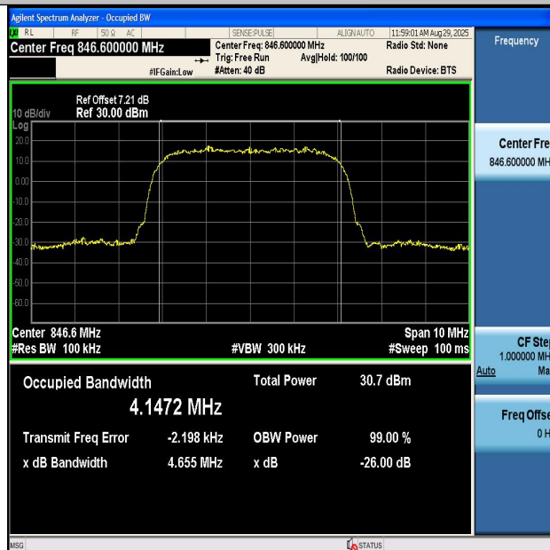
Band5-4233-PASS
