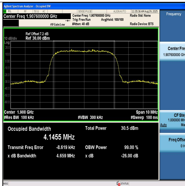
Band2-9538-PASS
