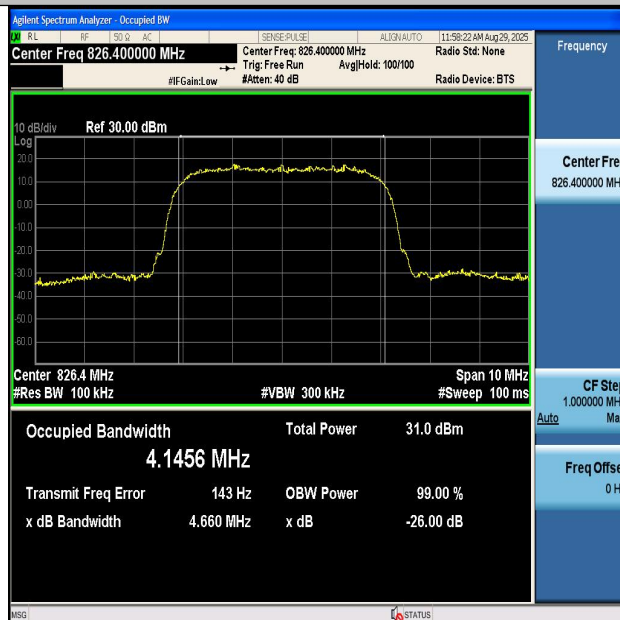
Band5-4132-PASS
