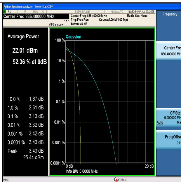
Band5-4182-PASS
