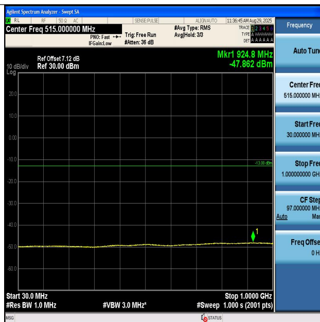
Band2-9400-30~1000MHz-PASS
