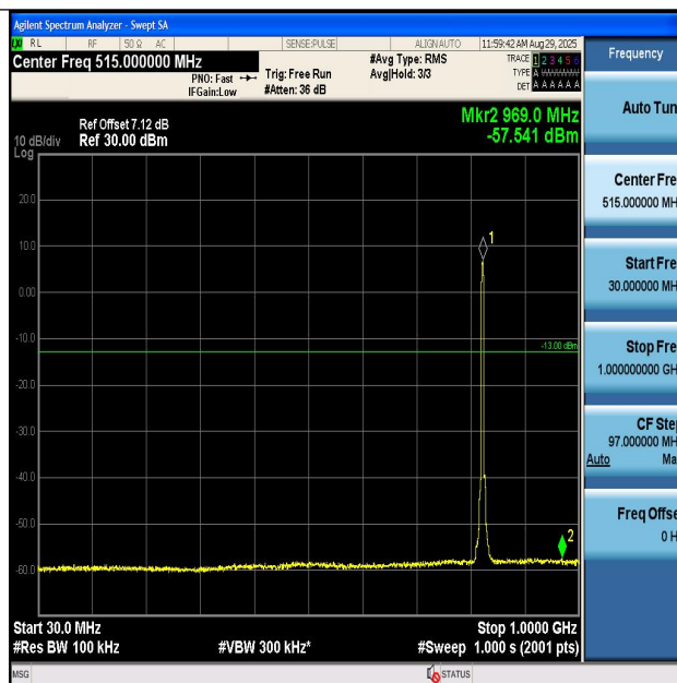
Band5-4132-30~1000MHz-PASS
