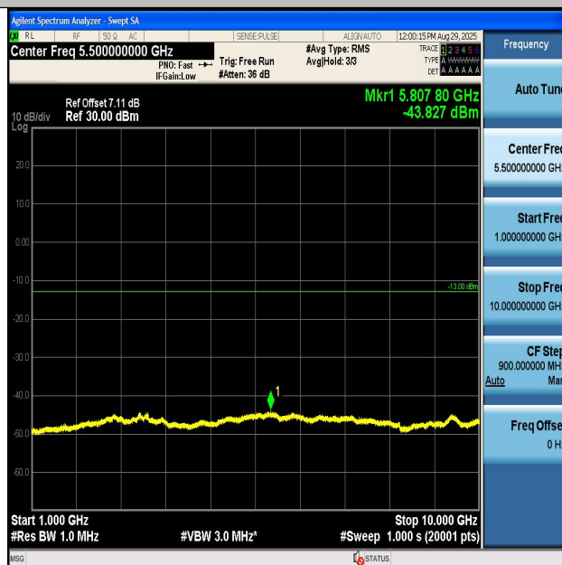
Band5-4182-1000~10000MHz-PASS
