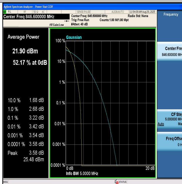
Band5-4233-PASS
