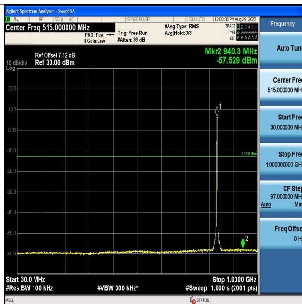
Band5-4182-30~1000MHz-PASS
