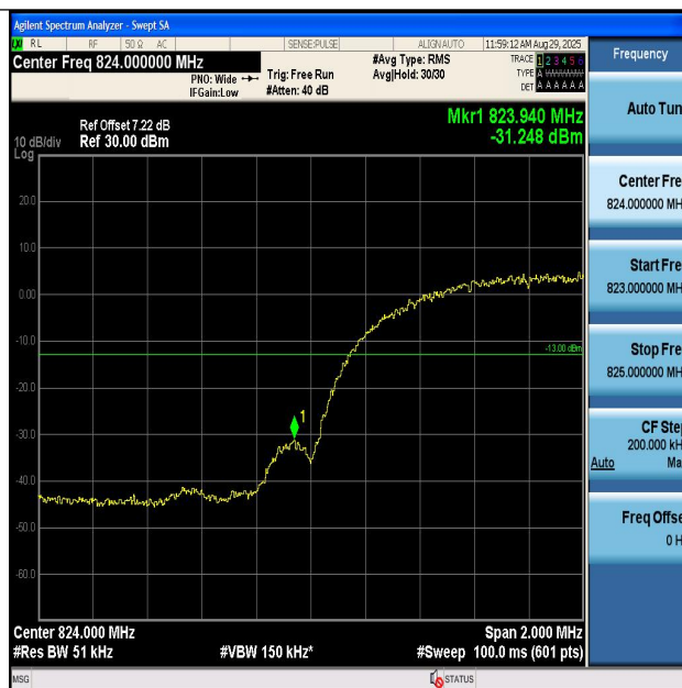
Band5-4132-PASS
