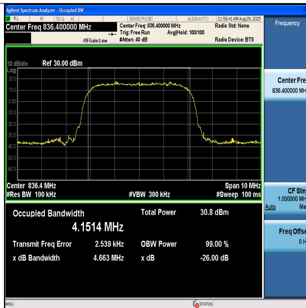
Band5-4182-PASS
