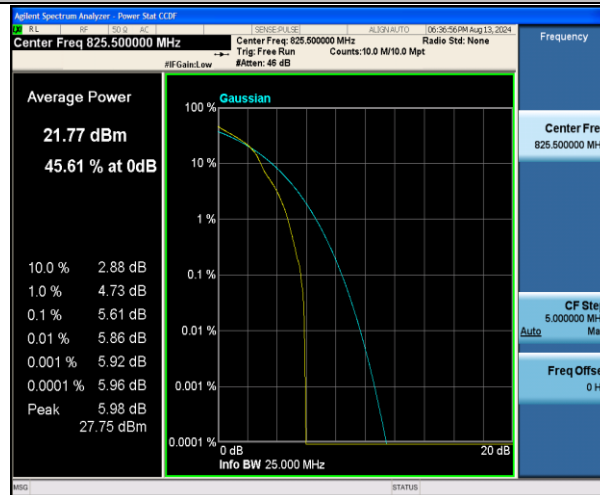
Band5-3MHz-16QAM-20415-1RB#0-PASS
