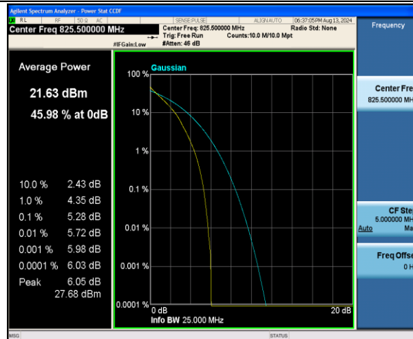
Band5-3MHz-QPSK-20415-15RB#0-PASS
