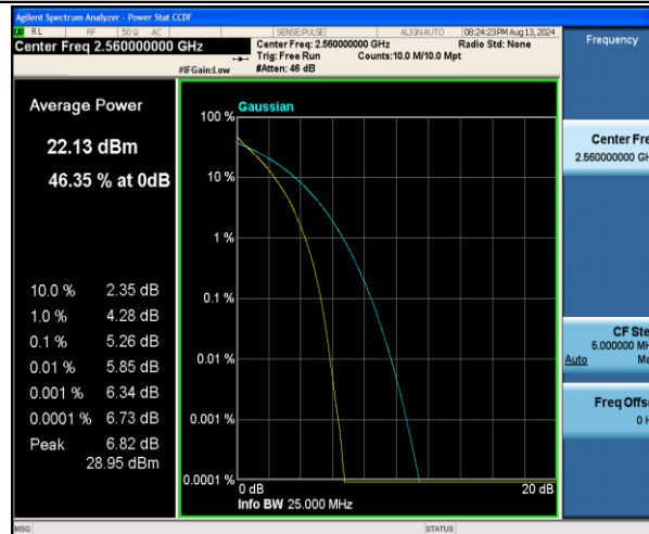
Band7-20MHz-QPSK-21350-100RB#0-PASS
