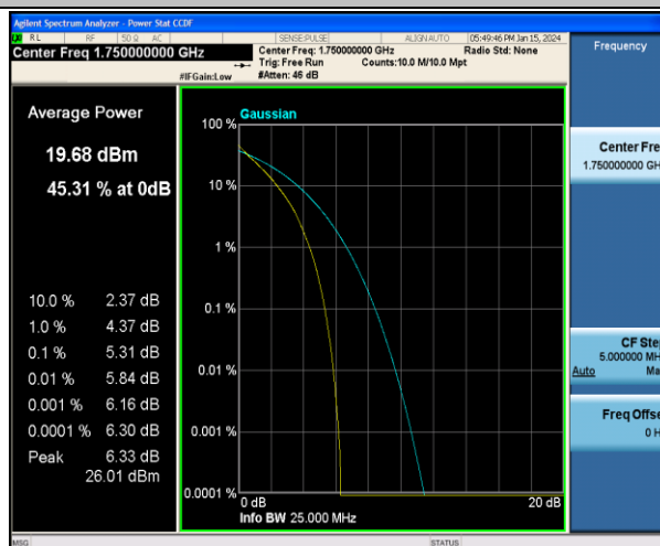
Band4-10MHz-QPSK-20350-50RB#0-PASS
