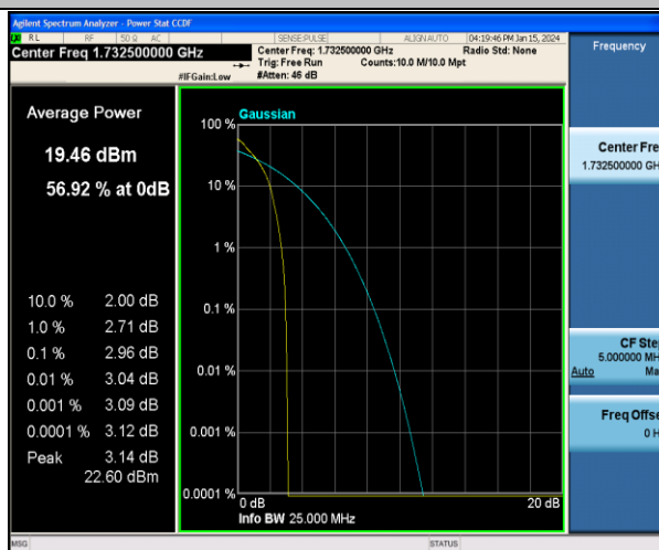
Band4-1.4MHz-QPSK-20175-1RB#0-PASS
