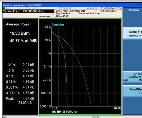
Band4-10MHz-QPSK-20175-50RB#0-PASS
