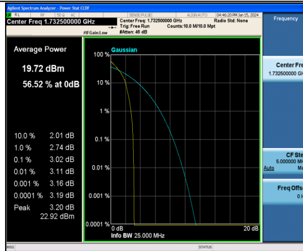
Band4-3MHz-QPSK-20175-1RB#0-PASS
