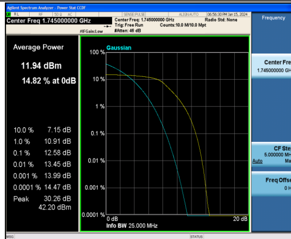
Band4-20MHz-QPSK-20300-100RB#0-PASS
