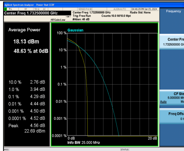
Band4-3MHz-16QAM-20175-1RB#0-PASS
