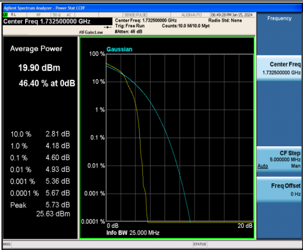
Band4-20MHz-16QAM-20175-1RB#0-PASS
