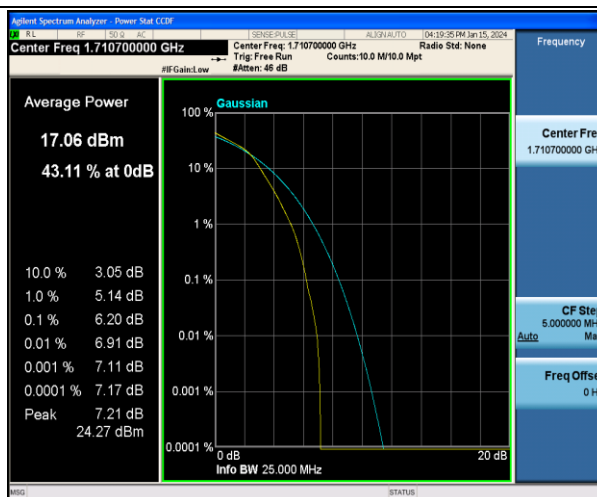
Band4-1.4MHz-16QAM-19957-6RB#0-PASS
