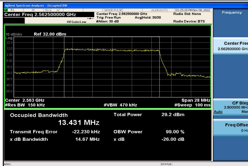
Band7-15MHz-QPSK-21375-75RB#0-13.431
