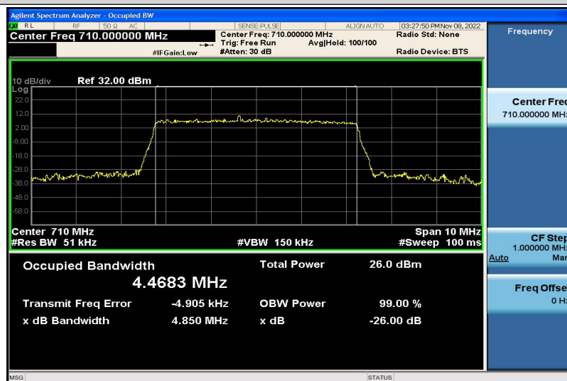
Band17-5MHz-16QAM-23790-25RB#0-4.4683
