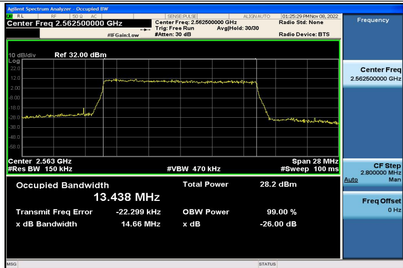
Band7-15MHz-16QAM-21375-75RB#0-13.438
