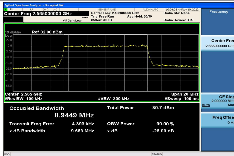
Band7-10MHz-QPSK-21400-50RB#0-8.9449
