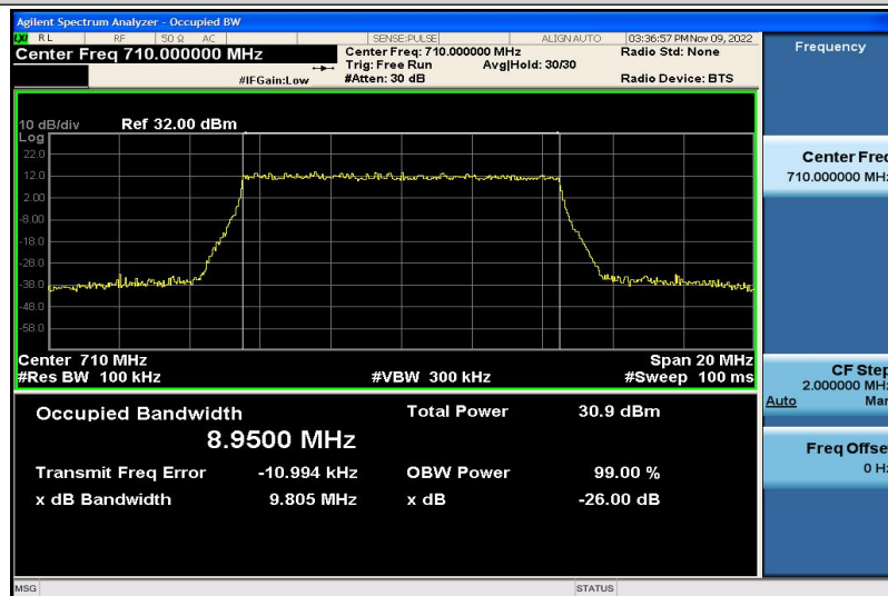
Band17-10MHz-QPSK-23790-50RB#0-8.9500
