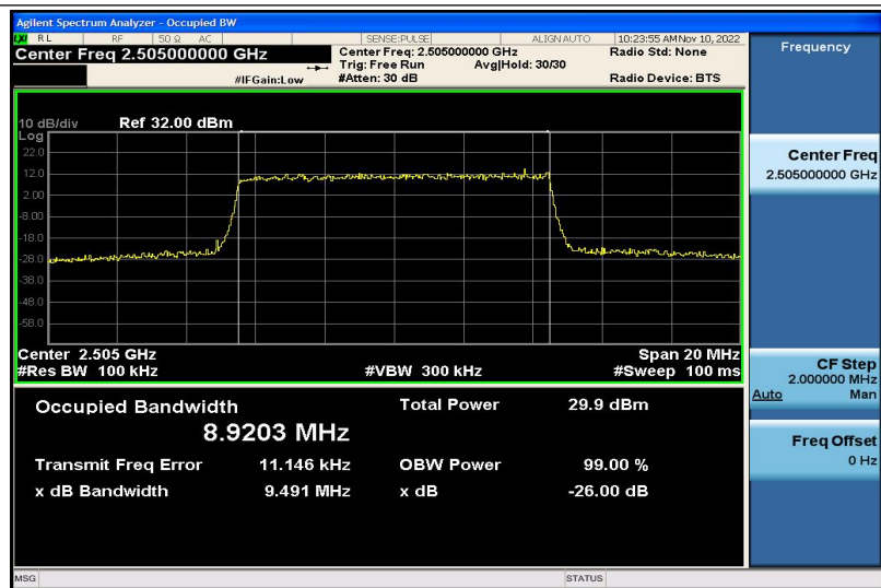
Band7-10MHz-16QAM-20800-50RB#0-8.9203
