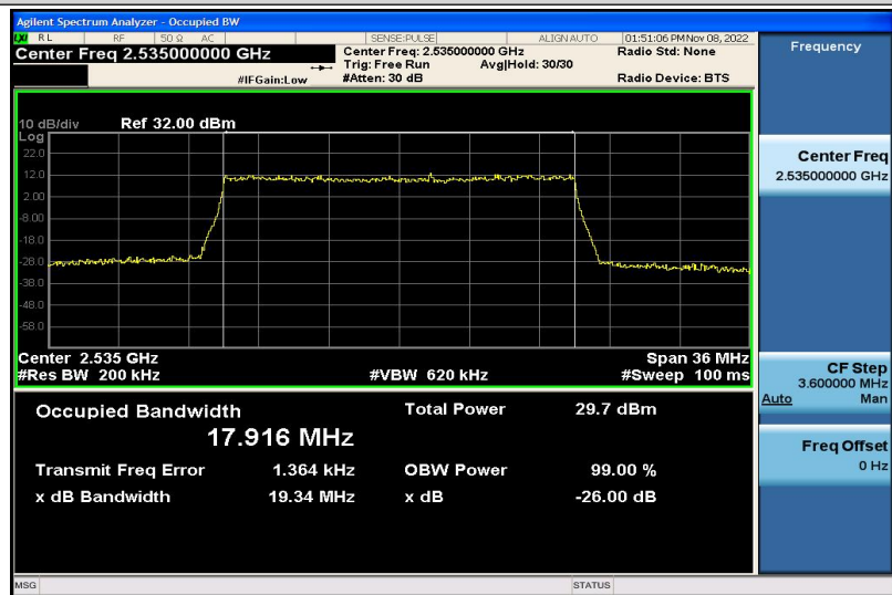
Band7-20MHz-QPSK-21100-100RB#0-17.916
