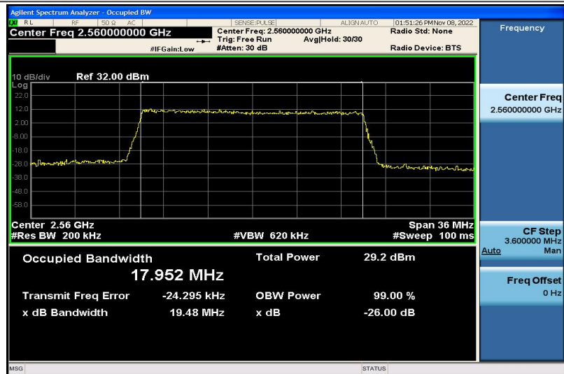
Band7-20MHz-QPSK-21350-100RB#0-17.952
