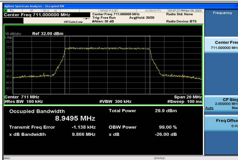
Band17-10MHz-16QAM-23800-50RB#0-8.9495
