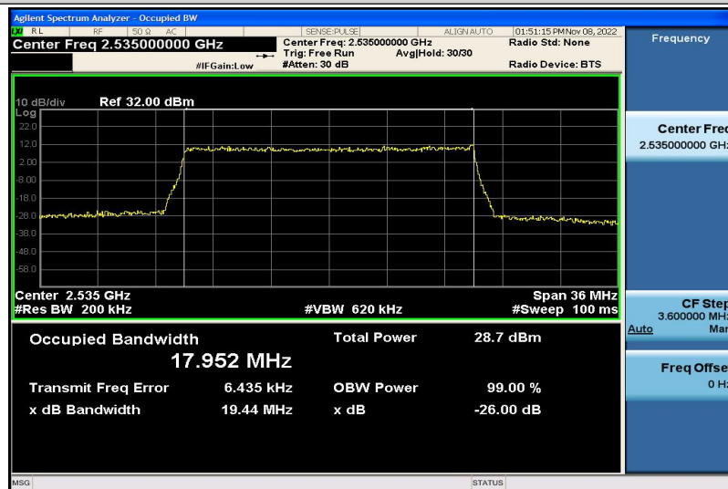
Band7-20MHz-16QAM-21100-100RB#0-17.952
