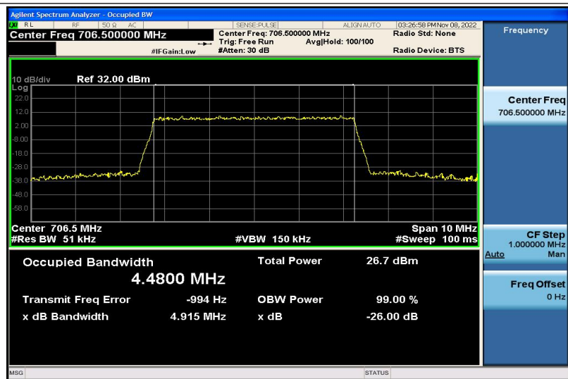
Band17-5MHz-QPSK-23755-25RB#0-4.4800
