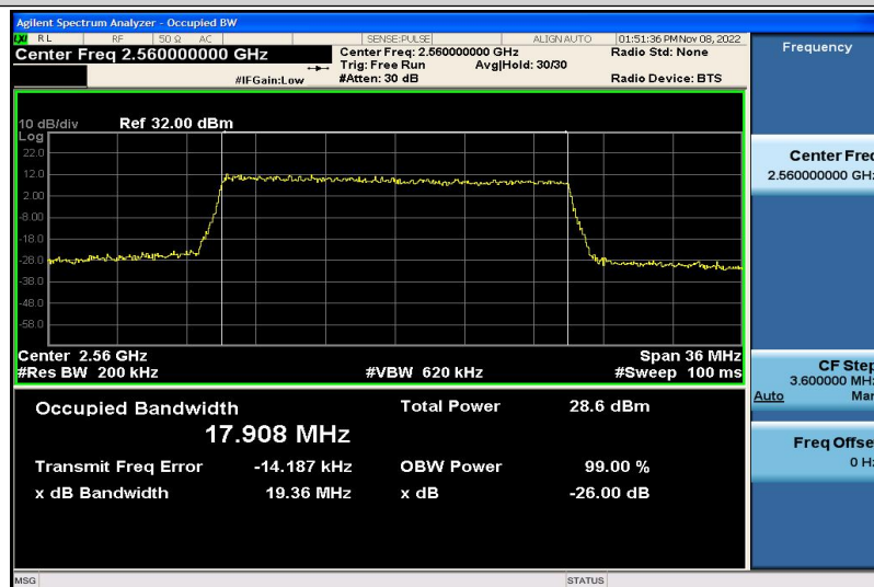
Band7-20MHz-16QAM-21350-100RB#0-17.908
