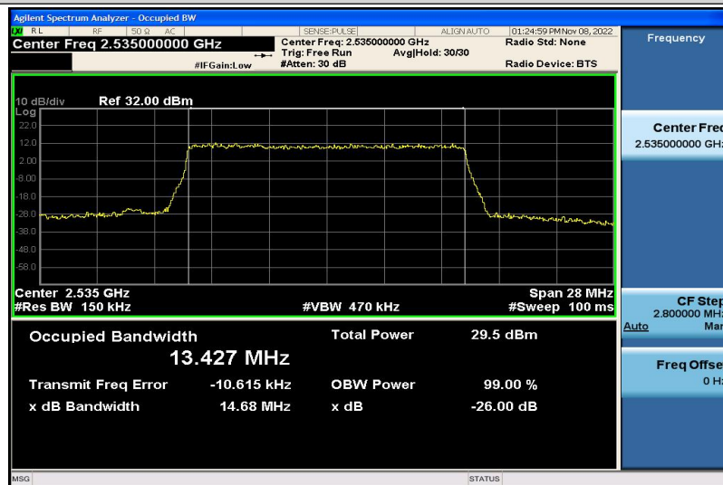
Band7-15MHz-QPSK-21100-75RB#0-13.427
