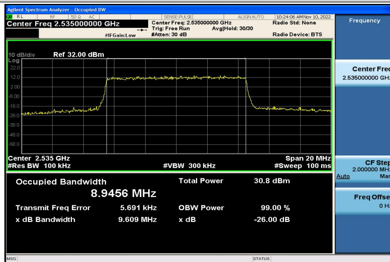
Band7-10MHz-QPSK-21100-50RB#0-8.9456
