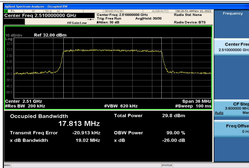
Band7-20MHz-16QAM-20850-100RB#0-17.813
