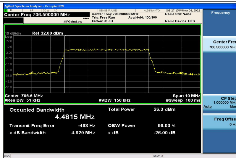
Band17-5MHz-16QAM-23755-25RB#0-4.4815
