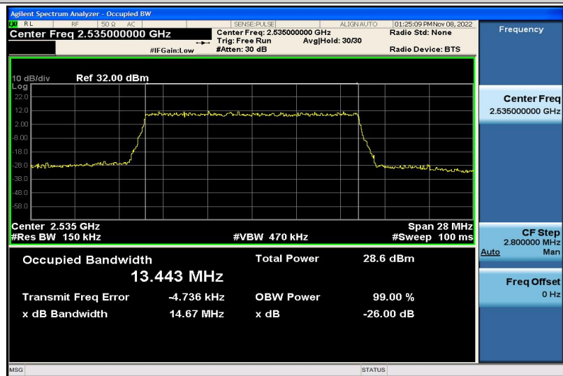
Band7-15MHz-16QAM-21100-75RB#0-13.443
