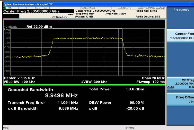
Band7-10MHz-QPSK-20800-50RB#0-8.9496
