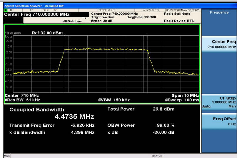
Band17-5MHz-QPSK-23790-25RB#0-4.4735
