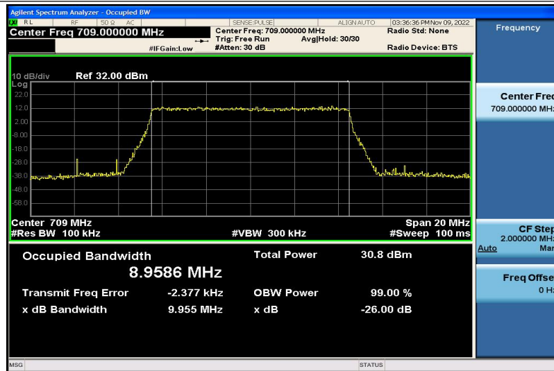
Band17-10MHz-QPSK-23780-50RB#0-8.9586
