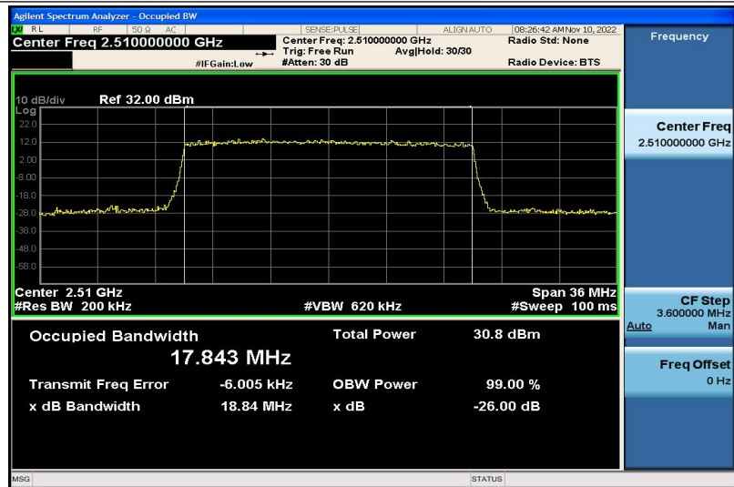
Band7-20MHz-QPSK-20850-100RB#0-17.843
