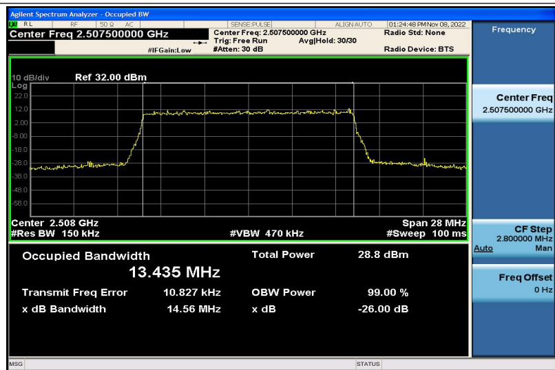
Band7-15MHz-16QAM-20825-75RB#0-13.435
