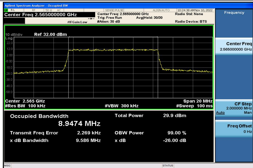
Band7-10MHz-16QAM-21400-50RB#0-8.9474
