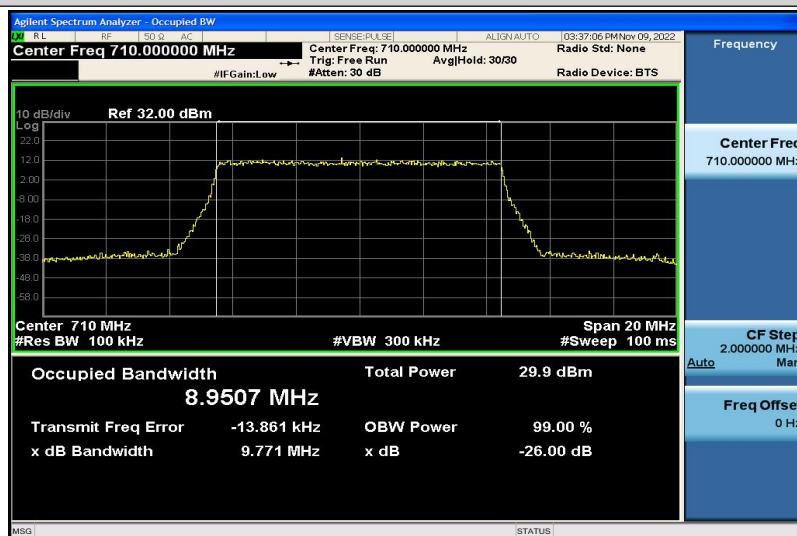
Band17-10MHz-16QAM-23790-50RB#0-8.9507
