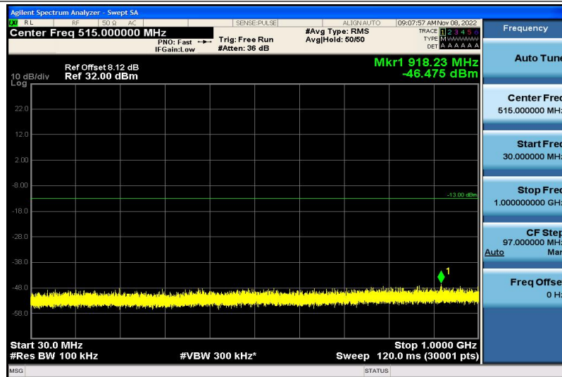
Band2-15MHz-16QAM-18675-1RB#0-30~1000MHz
