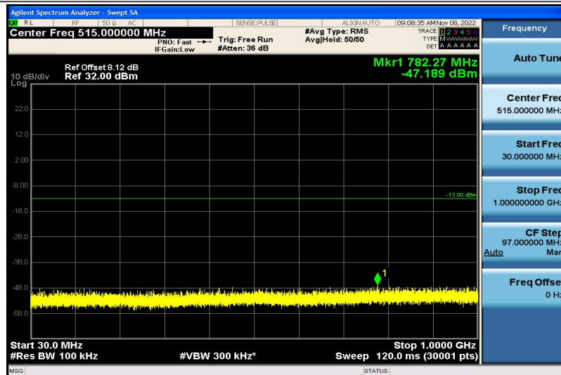
Band2-15MHz-QPSK-18900-1RB#0-30~1000MHz
