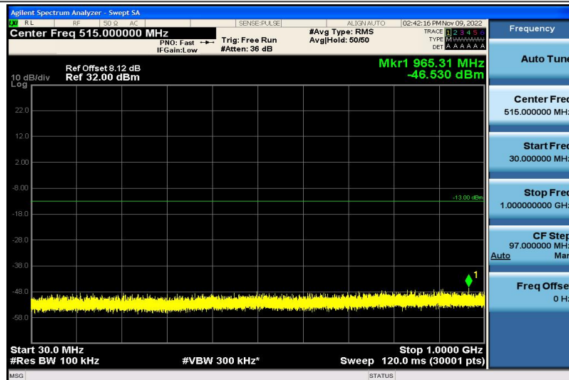
Band2-10MHz-QPSK-18900-1RB#0-30~1000MHz
