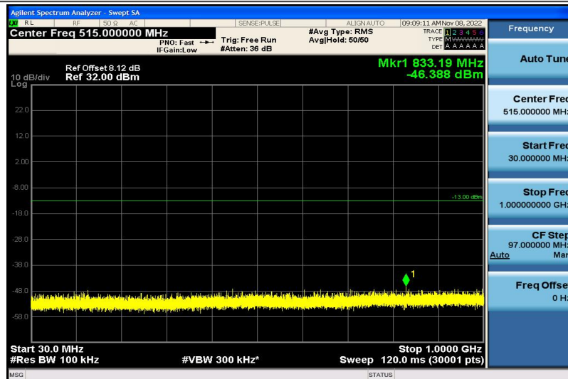
Band2-15MHz-16QAM-18900-1RB#0-30~1000MHz
