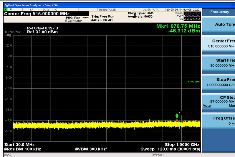
Band4-15MHz-16QAM-20175-1RB#0-30~1000MHz
