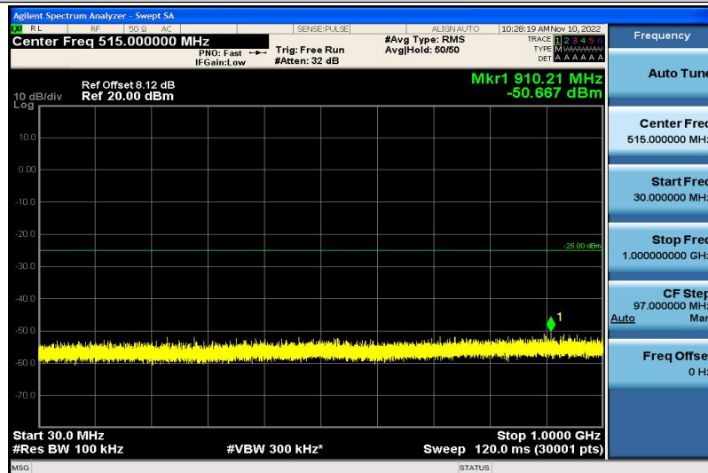
Band7-10MHz-16QAM-21100-1RB#0-30~1000MHz
