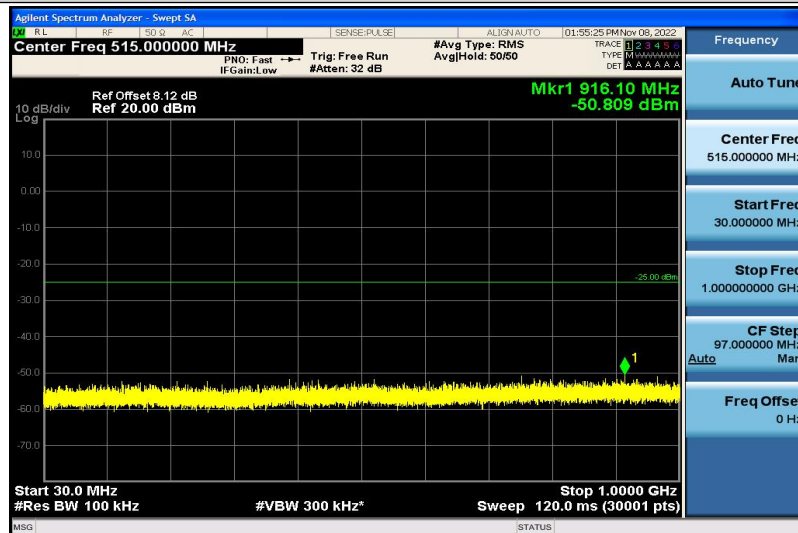
Band7-20MHz-16QAM-21100-1RB#0-30~1000MHz
