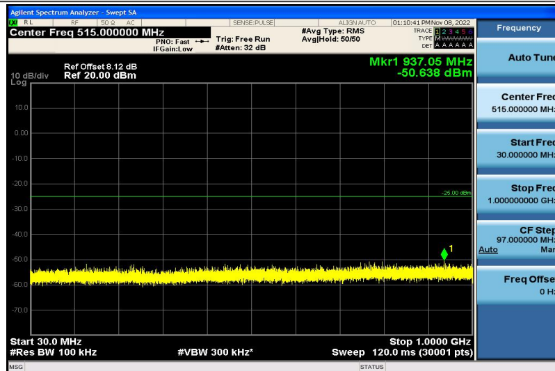
Band7-5MHz-16QAM-21100-1RB#0-30~1000MHz
