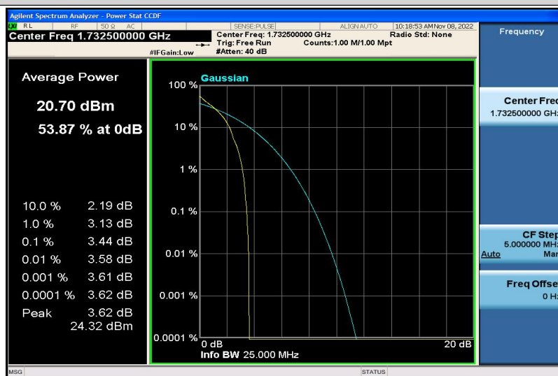
Band4-3MHz-QPSK-20175-1RB#0
