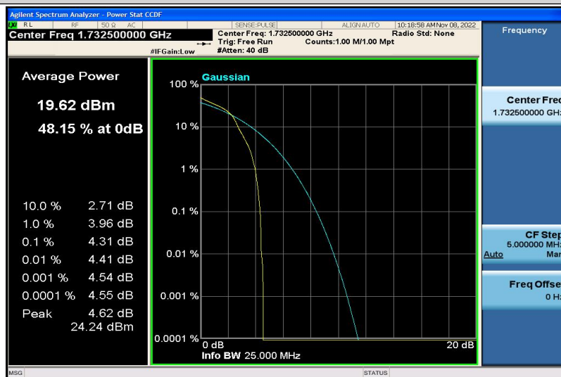
Band4-3MHz-16QAM-20175-1RB#0
