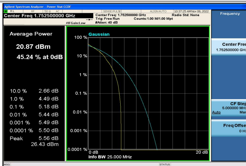
Band4-5MHz-QPSK-20375-1RB#0
