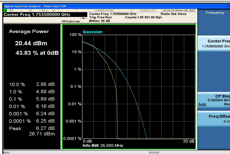
Band4-3MHz-16QAM-20385-1RB#0
