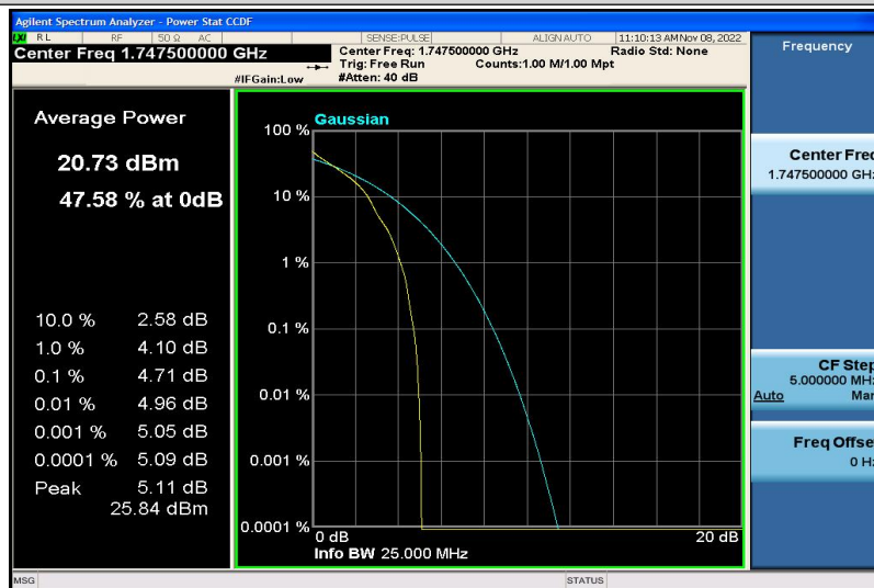
Band4-15MHz-QPSK-20325-1RB#0
