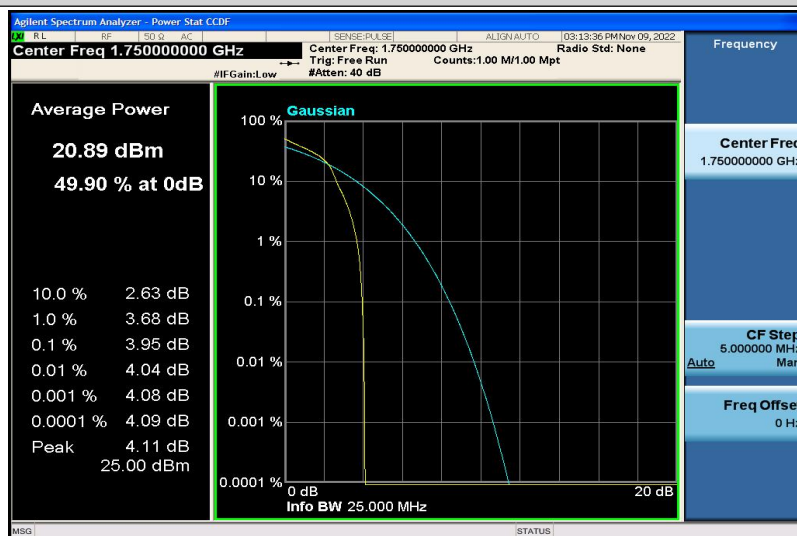
Band4-10MHz-16QAM-20350-1RB#0
