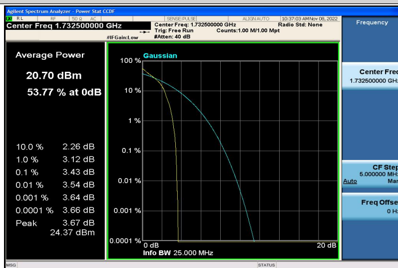
Band4-5MHz-QPSK-20175-1RB#0
