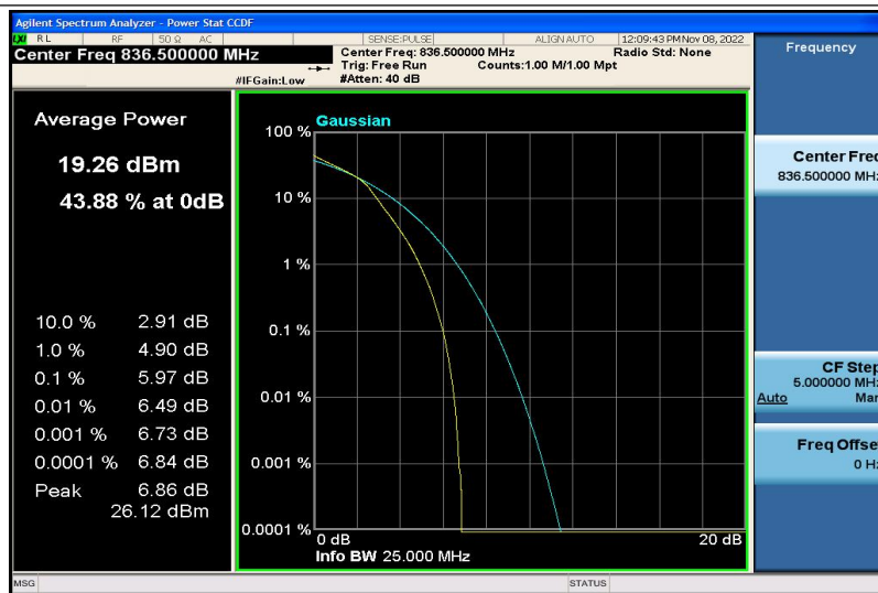
Band5-3MHz-16QAM-20525-15RB#0
