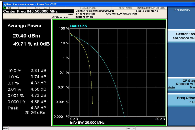
Band5-5MHz-QPSK-20625-25RB#0
