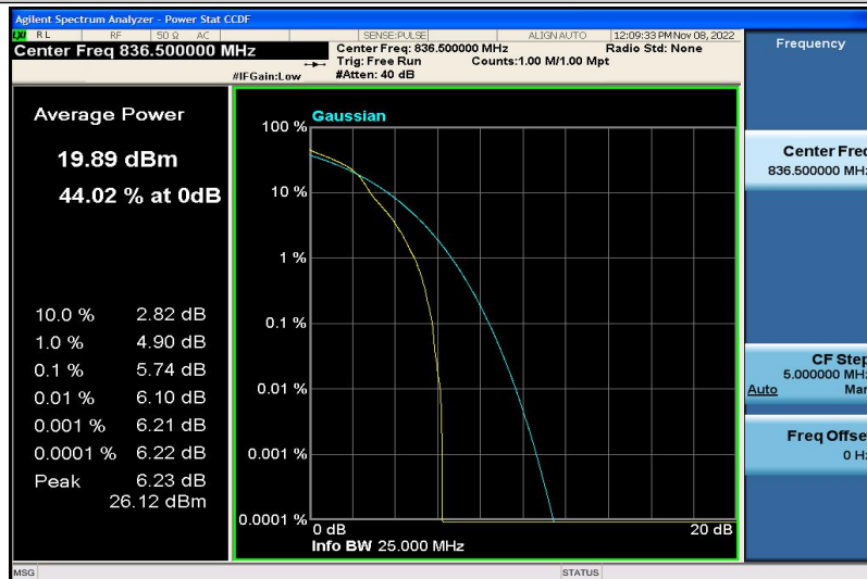
Band5-3MHz-16QAM-20525-1RB#0
