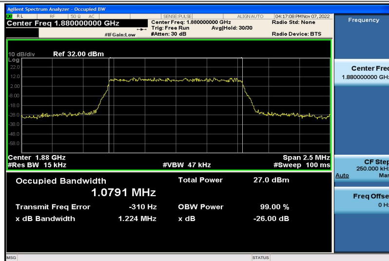
Band2-1.4MHz-QPSK-18900-6RB#0-1.0791
