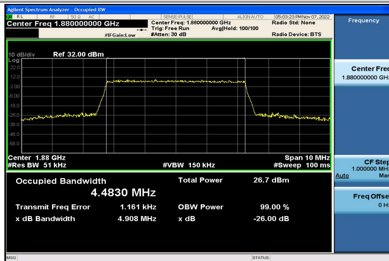
Band2-5MHz-16QAM-18900-25RB#0-4.4830
