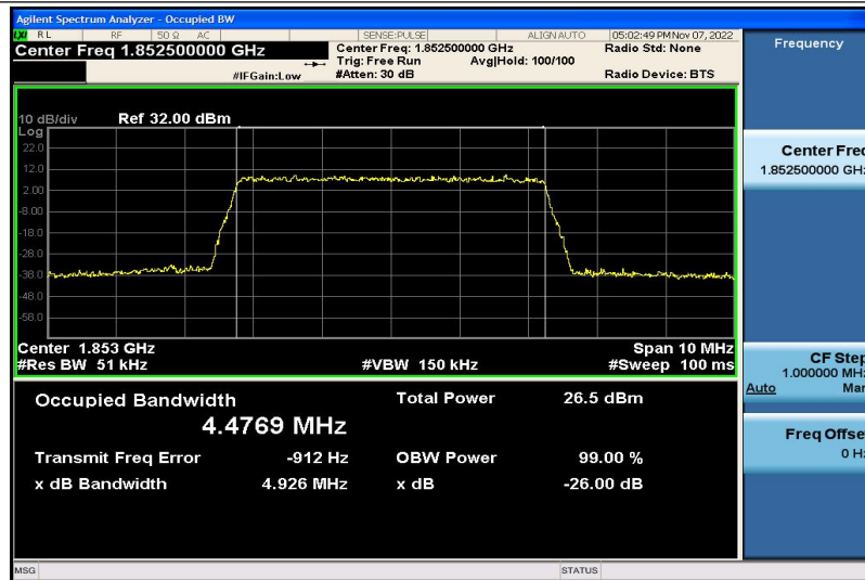
Band2-5MHz-16QAM-18625-25RB#0-4.4769
