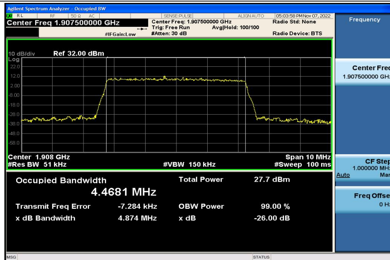
Band2-5MHz-16QAM-19175-25RB#0-4.4681
