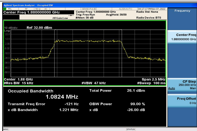
Band2-1.4MHz-16QAM-18900-6RB#0-1.0824
