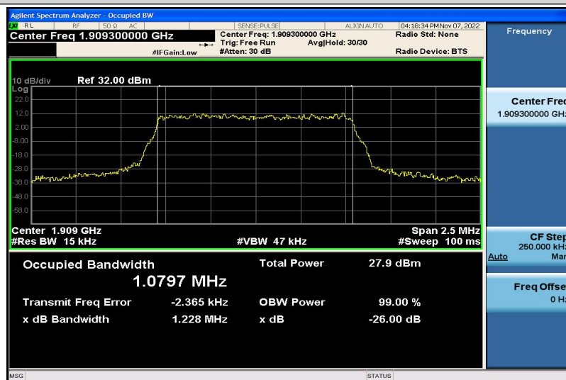
Band2-1.4MHz-QPSK-19193-6RB#0-1.0797
