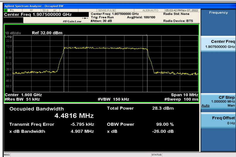
Band2-5MHz-QPSK-19175-25RB#0-4.4816
