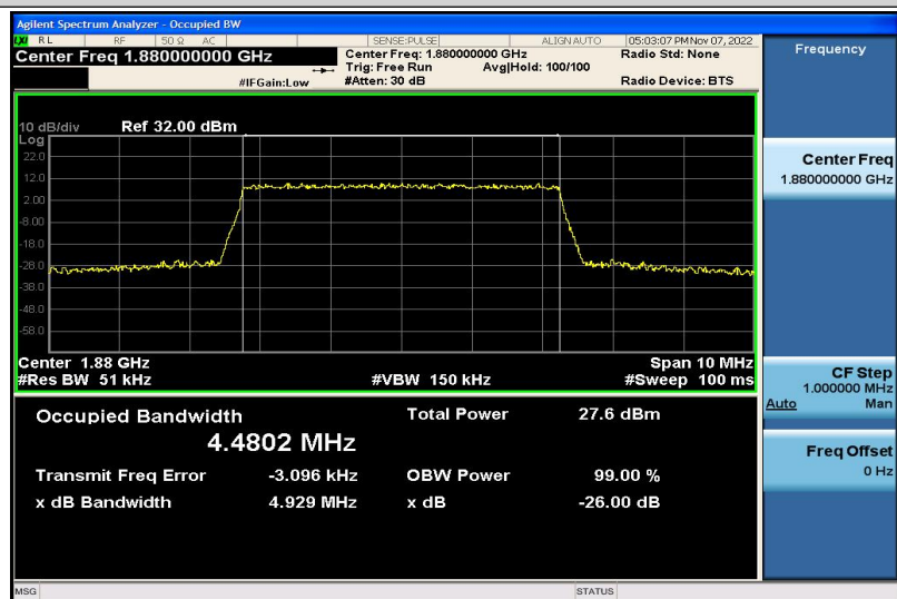
Band2-5MHz-QPSK-18900-25RB#0-4.4802
