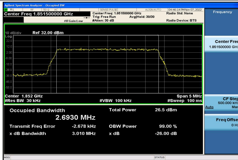
Band2-3MHz-16QAM-18615-15RB#0-2.6930
