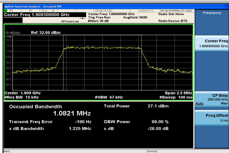
Band2-1.4MHz-16QAM-19193-6RB#0-1.0821
