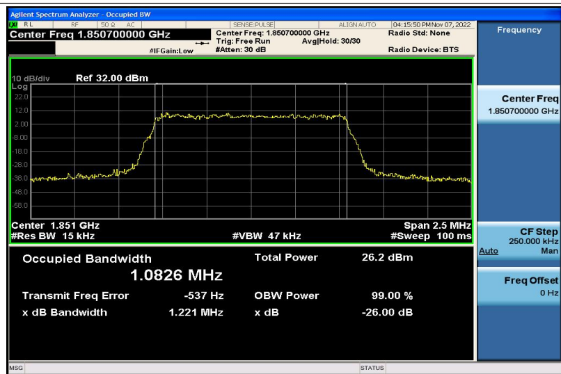
Band2-1.4MHz-16QAM-18607-6RB#0-1.0826
