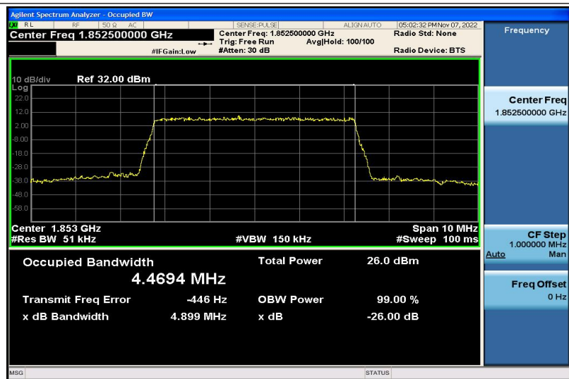
Band2-5MHz-QPSK-18625-25RB#0-4.4694
