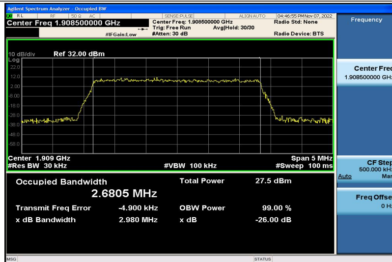
Band2-3MHz-16QAM-19185-15RB#0-2.6805
