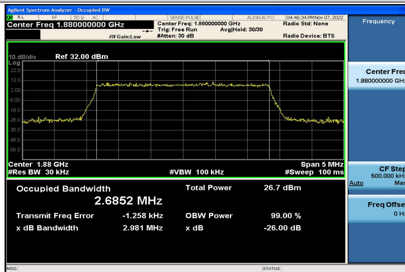
Band2-3MHz-16QAM-18900-15RB#0-2.6852
