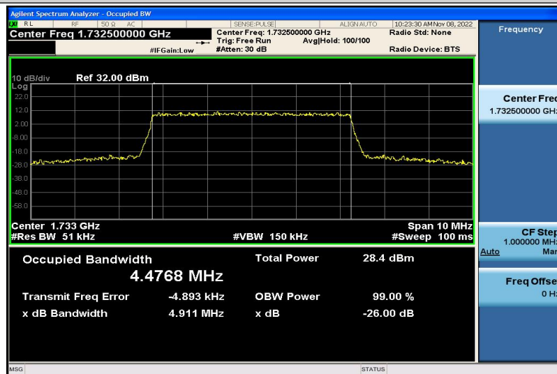
Band4-5MHz-QPSK-20175-25RB#0-4.4768
