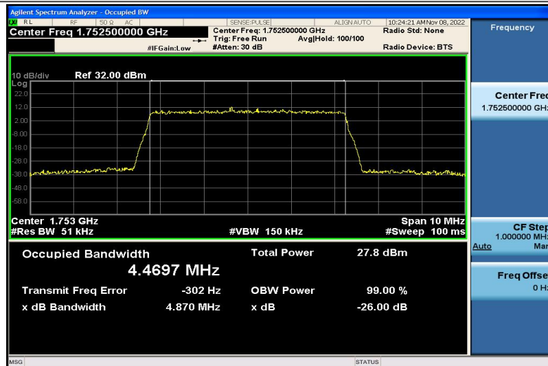
Band4-5MHz-16QAM-20375-25RB#0-4.4697
