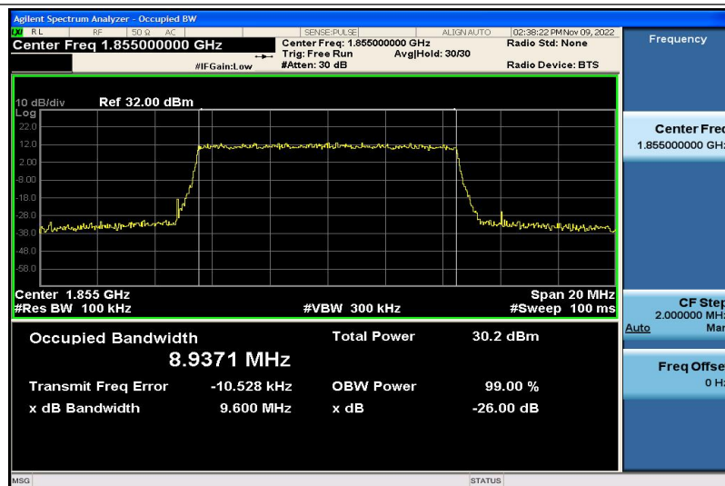
Band2-10MHz-QPSK-18650-50RB#0-8.9371
