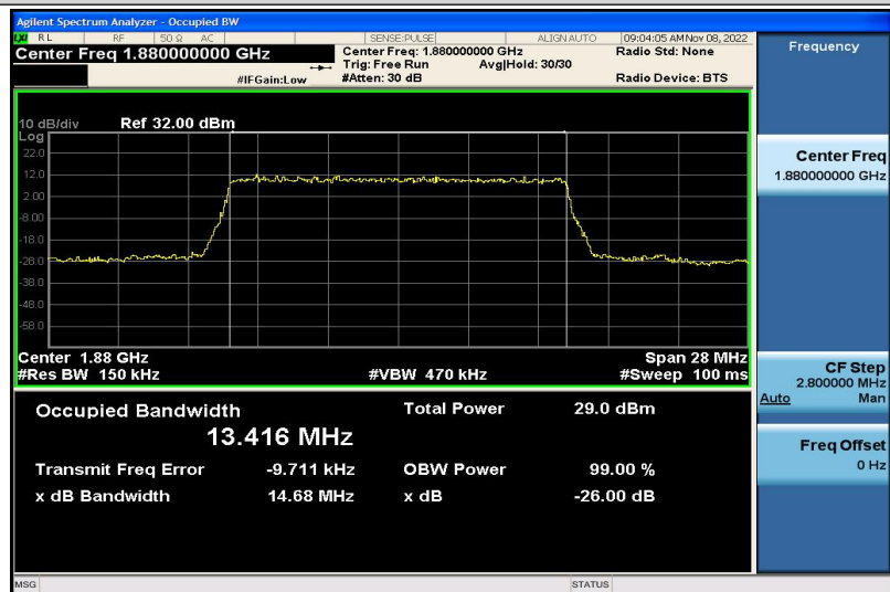
Band2-15MHz-QPSK-18900-75RB#0-13.416
