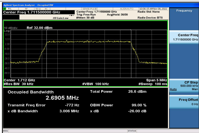
Band4-3MHz-16QAM-19965-15RB#0-2.6905
