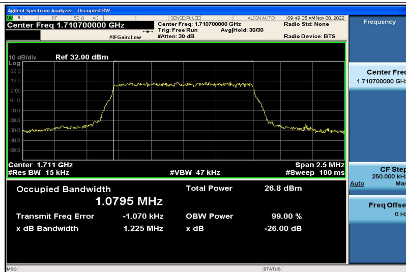
Band4-1.4MHz-QPSK-19957-6RB#0-1.0795
