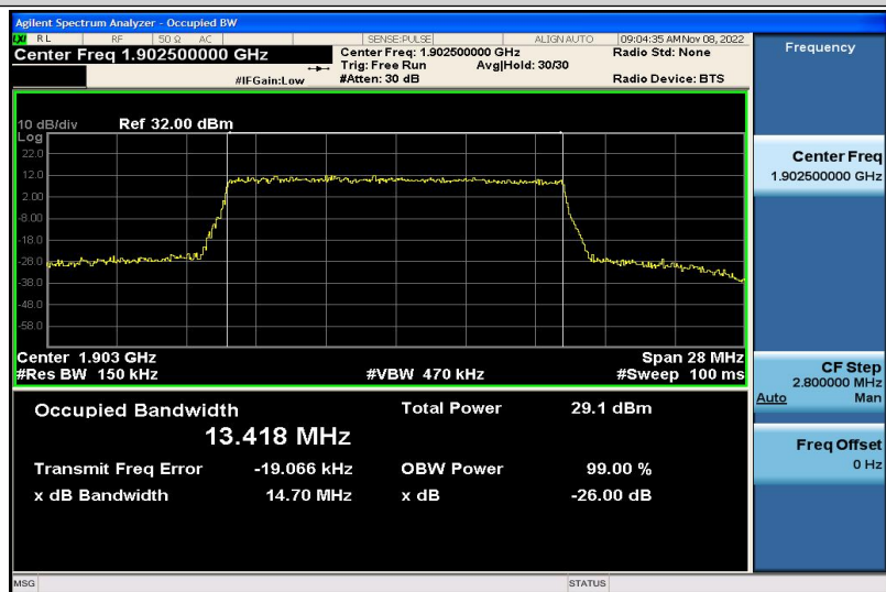
Band2-15MHz-16QAM-19125-75RB#0-13.418
