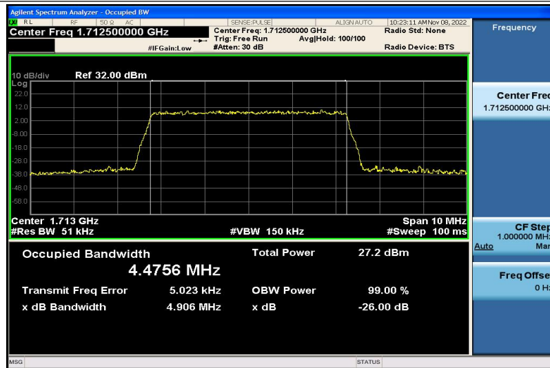
Band4-5MHz-16QAM-19975-25RB#0-4.4756
