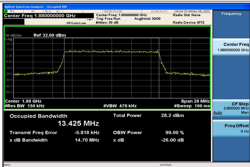
Band2-15MHz-16QAM-18900-75RB#0-13.425
