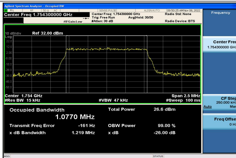
Band4-1.4MHz-16QAM-20393-6RB#0-1.0770
