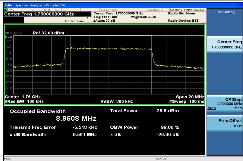
Band4-10MHz-16QAM-20350-50RB#0-8.9608
