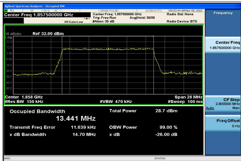
Band2-15MHz-QPSK-18675-75RB#0-13.441
