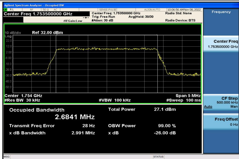
Band4-3MHz-16QAM-20385-15RB#0-2.6841
