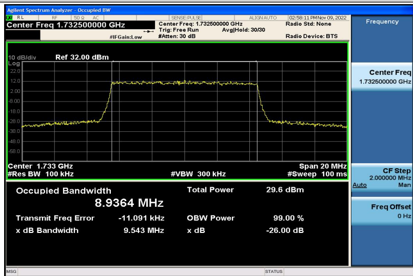
Band4-10MHz-QPSK-20175-50RB#0-8.9364
