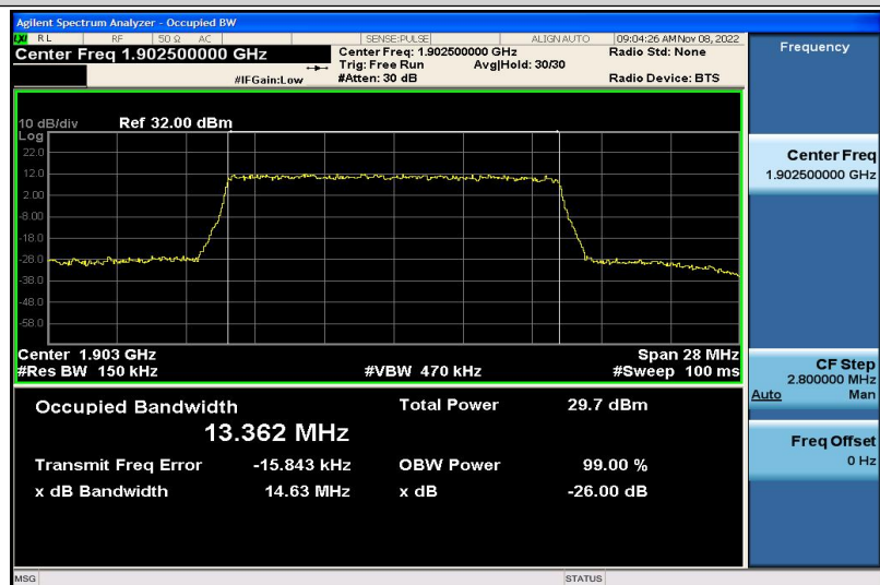
Band2-15MHz-QPSK-19125-75RB#0-13.362
