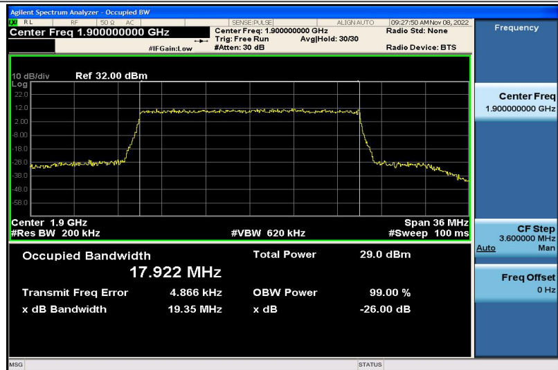
Band2-20MHz-16QAM-19100-100RB#0-17.922
