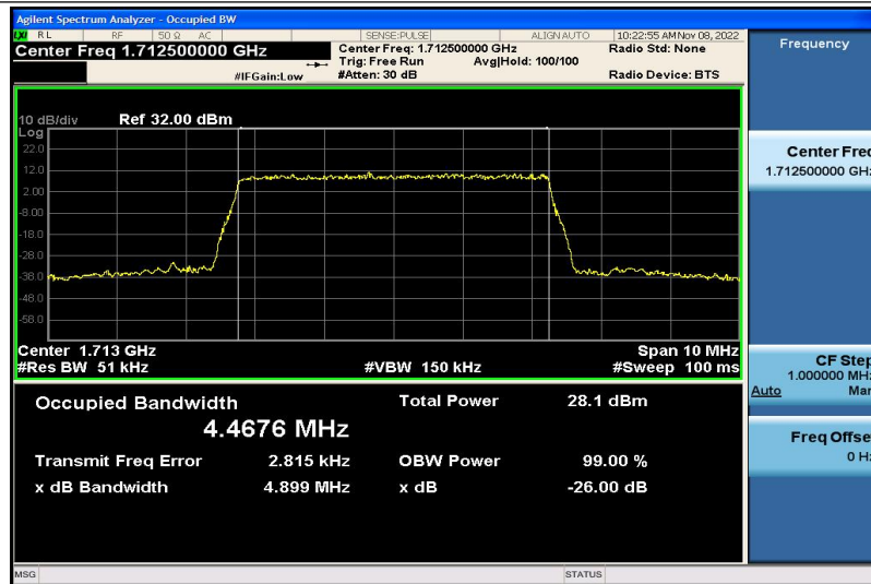
Band4-5MHz-QPSK-19975-25RB#0-4.4676
