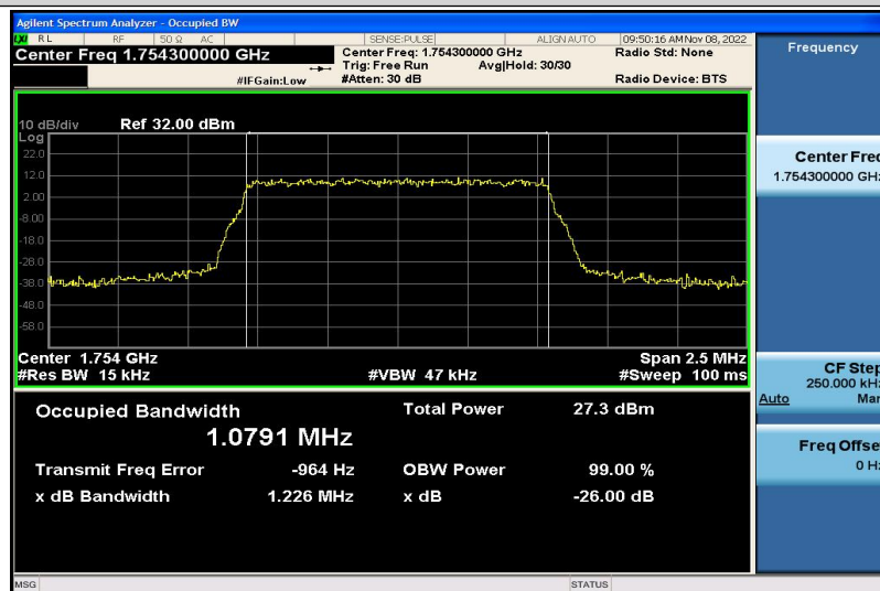
Band4-1.4MHz-QPSK-20393-6RB#0-1.0791
