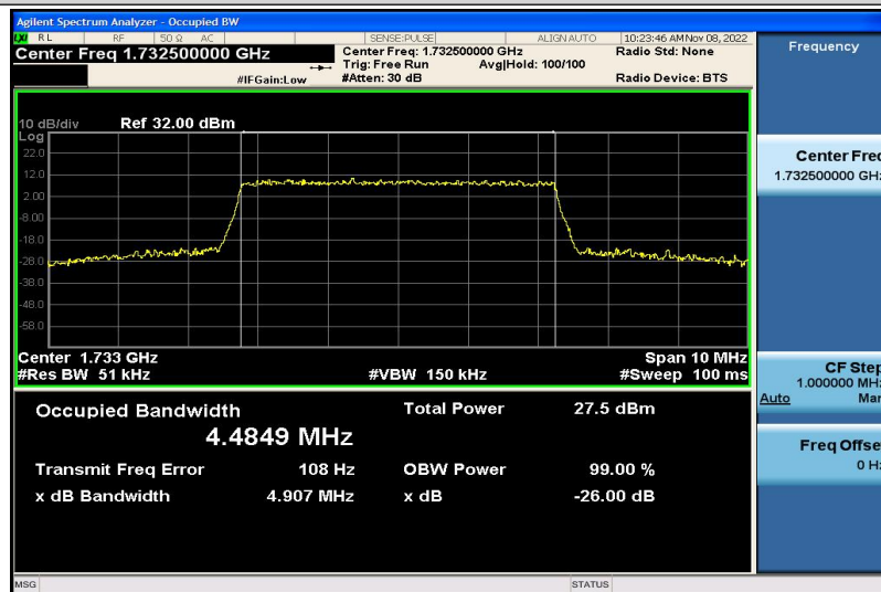
Band4-5MHz-16QAM-20175-25RB#0-4.4849
