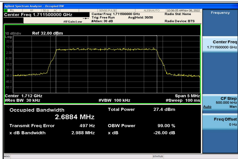
Band4-3MHz-QPSK-19965-15RB#0-2.6884
