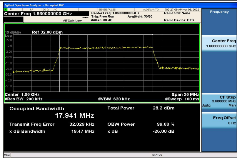
Band2-20MHz-16QAM-18700-100RB#0-17.941
