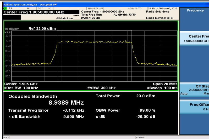
Band2-10MHz-16QAM-19150-50RB#0-8.9389
