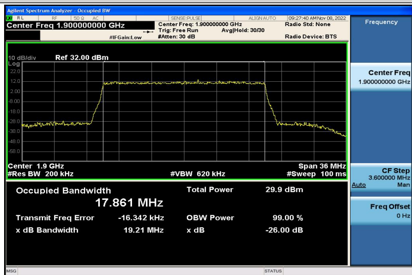
Band2-20MHz-QPSK-19100-100RB#0-17.861
