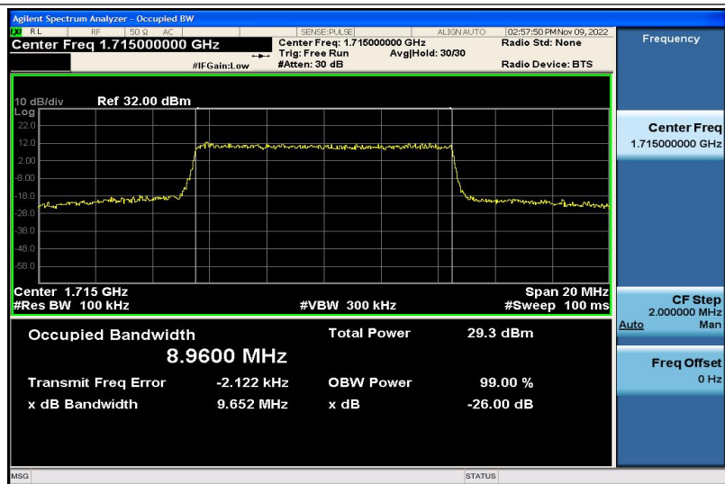
Band4-10MHz-QPSK-20000-50RB#0-8.9600
