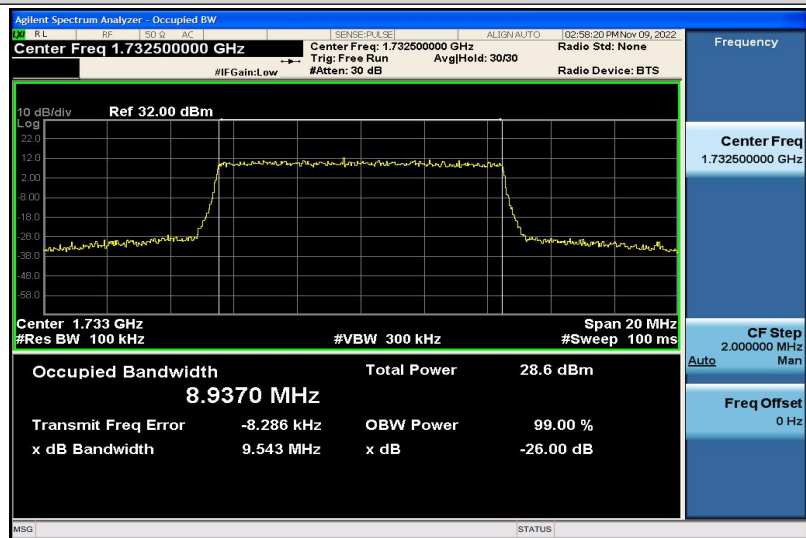
Band4-10MHz-16QAM-20175-50RB#0-8.9370
