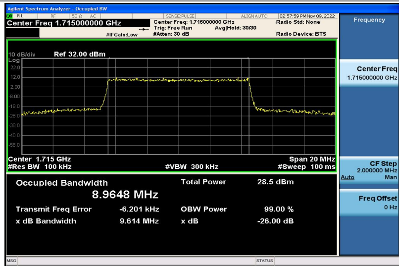
Band4-10MHz-16QAM-20000-50RB#0-8.9648
