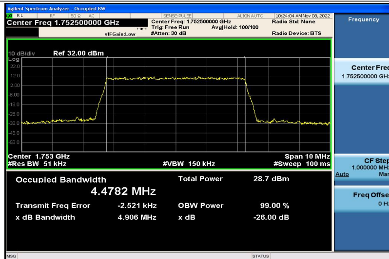
Band4-5MHz-QPSK-20375-25RB#0-4.4782
