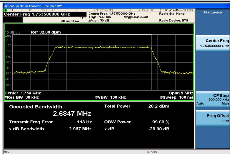
Band4-3MHz-QPSK-20385-15RB#0-2.6847
