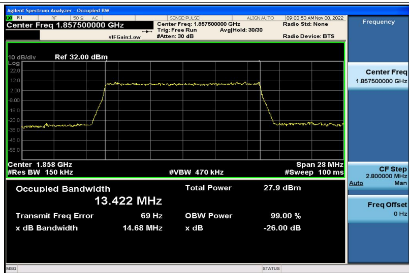
Band2-15MHz-16QAM-18675-75RB#0-13.422
