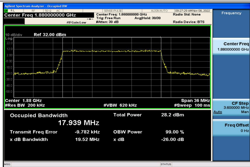
Band2-20MHz-16QAM-18900-100RB#0-17.939
