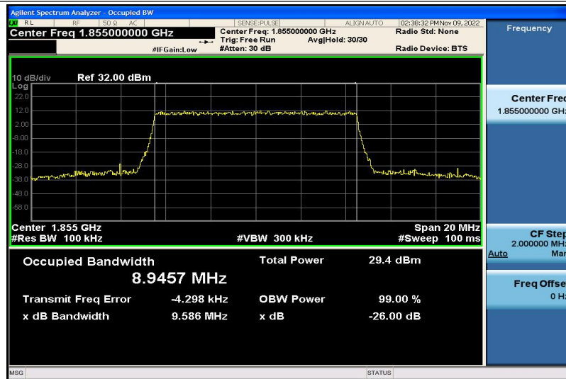
Band2-10MHz-16QAM-18650-50RB#0-8.9457
