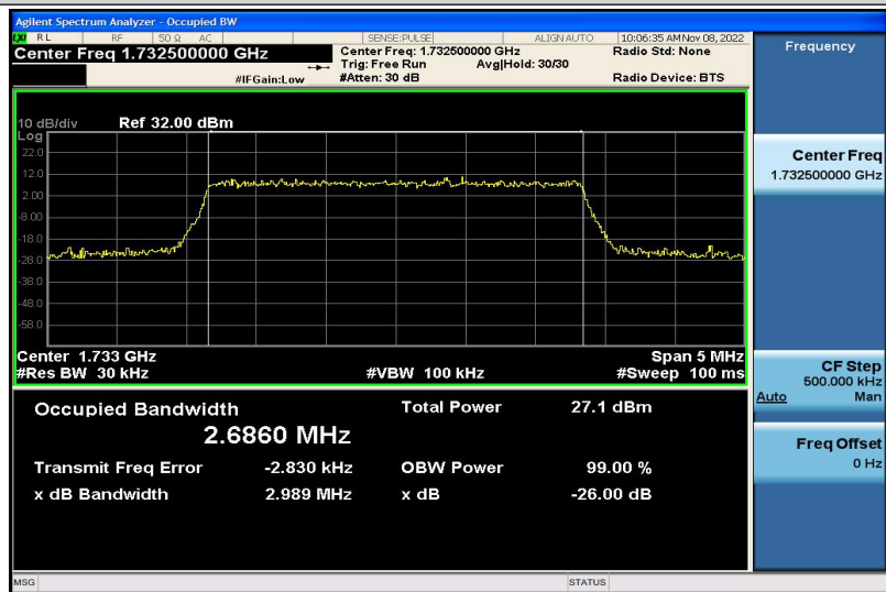
Band4-3MHz-16QAM-20175-15RB#0-2.6860
