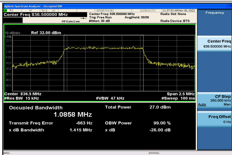
Band5-1.4MHz-16QAM-20525-6RB#0-1.0858
