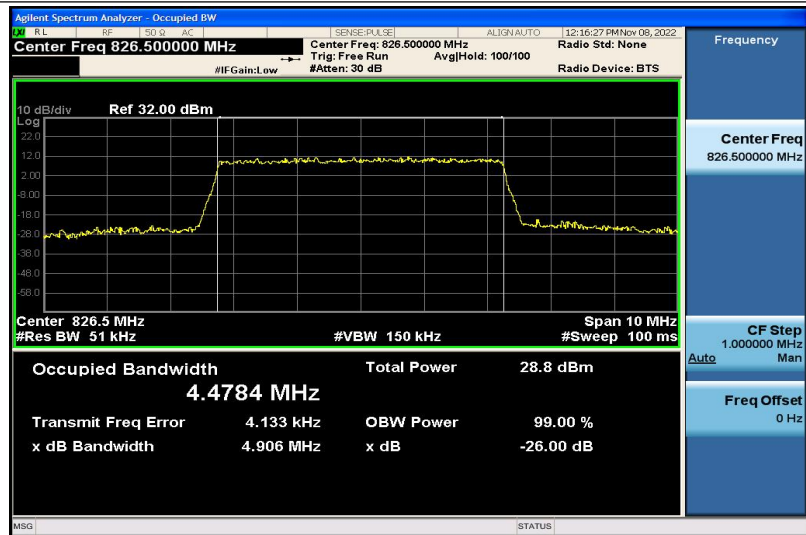
Band5-5MHz-QPSK-20425-25RB#0-4.4784
