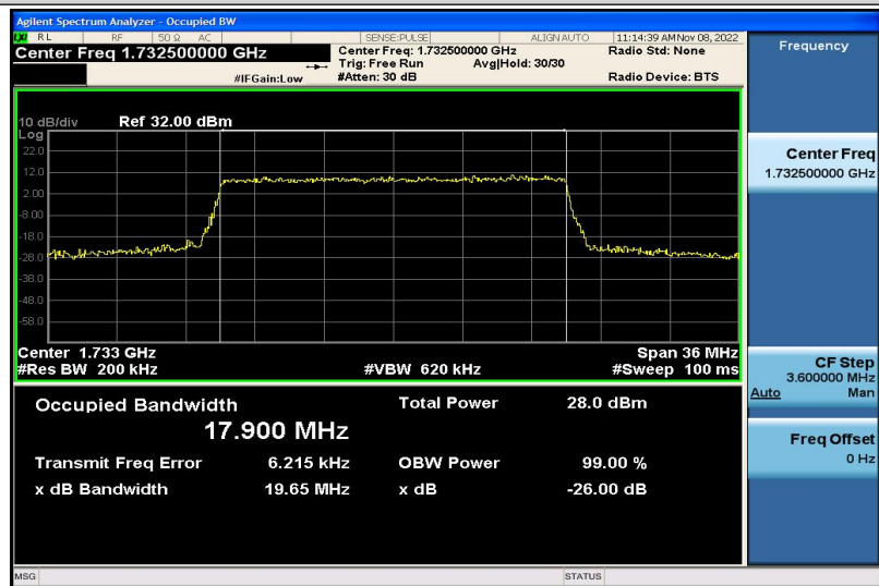
Band4-20MHz-16QAM-20175-100RB#0-17.900
