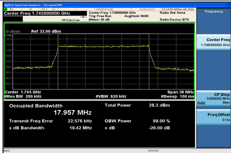
Band4-20MHz-16QAM-20300-100RB#0-17.957
