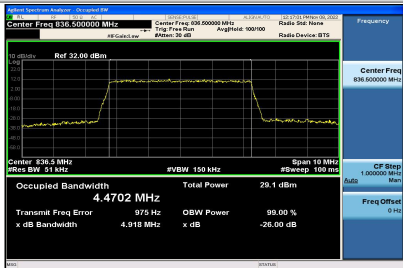
Band5-5MHz-QPSK-20525-25RB#0-4.4702
