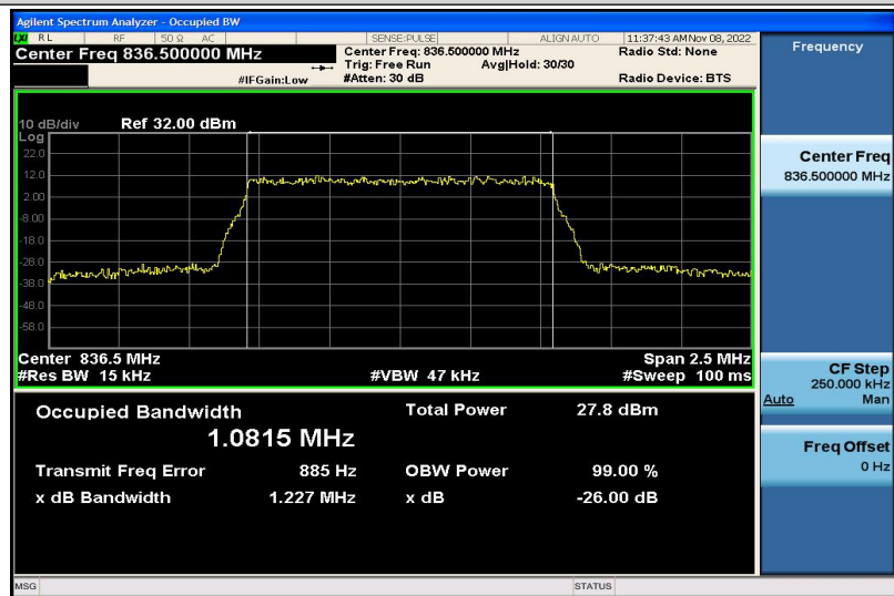
Band5-1.4MHz-QPSK-20525-6RB#0-1.0815
