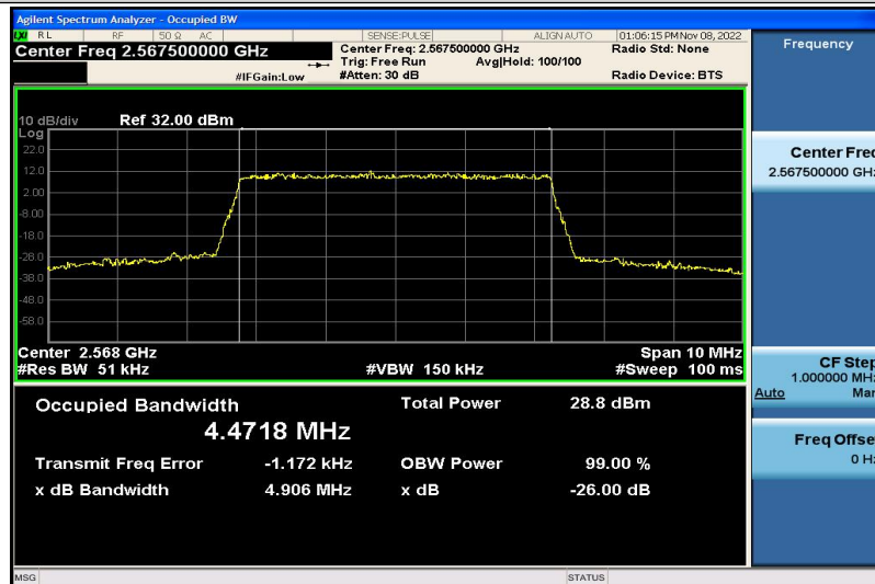
Band7-5MHz-QPSK-21425-25RB#0-4.4718
