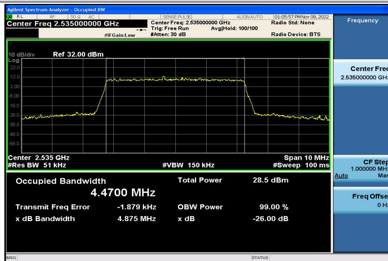
Band7-5MHz-16QAM-21100-25RB#0-4.4700
