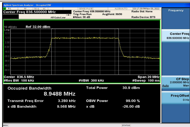
Band5-10MHz-16QAM-20525-50RB#0-8.9488
