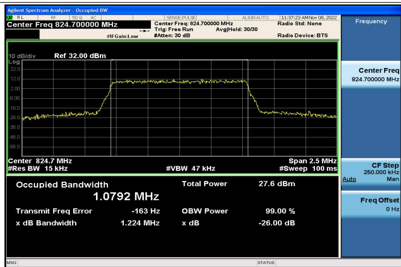
Band5-1.4MHz-QPSK-20407-6RB#0-1.0792
