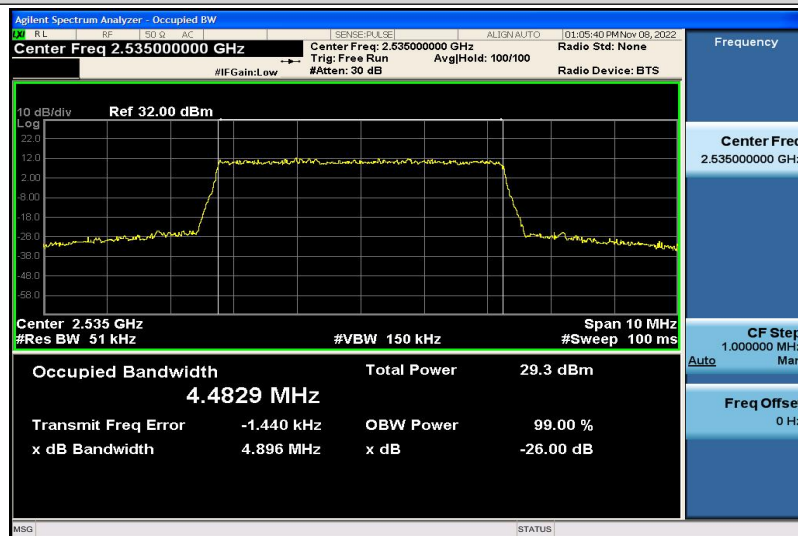
Band7-5MHz-QPSK-21100-25RB#0-4.4829
