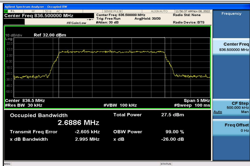
Band5-3MHz-16QAM-20525-15RB#0-2.6886
