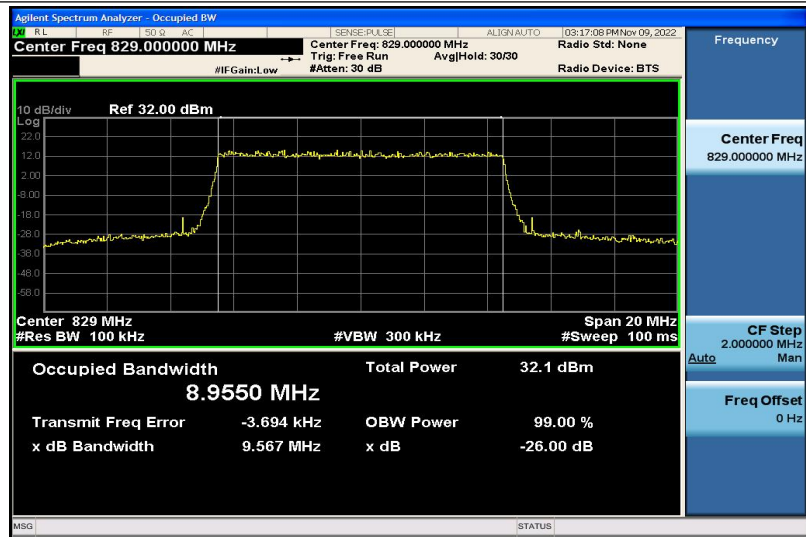
Band5-10MHz-QPSK-20450-50RB#0-8.9550
