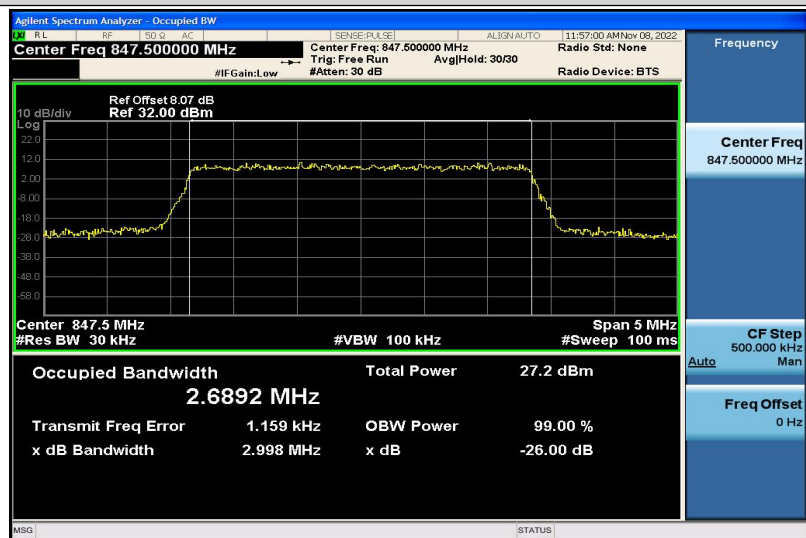
Band5-3MHz-16QAM-20635-15RB#0-2.6892
