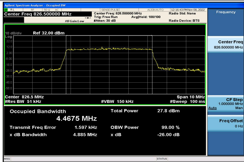
Band5-5MHz-16QAM-20425-25RB#0-4.4675
