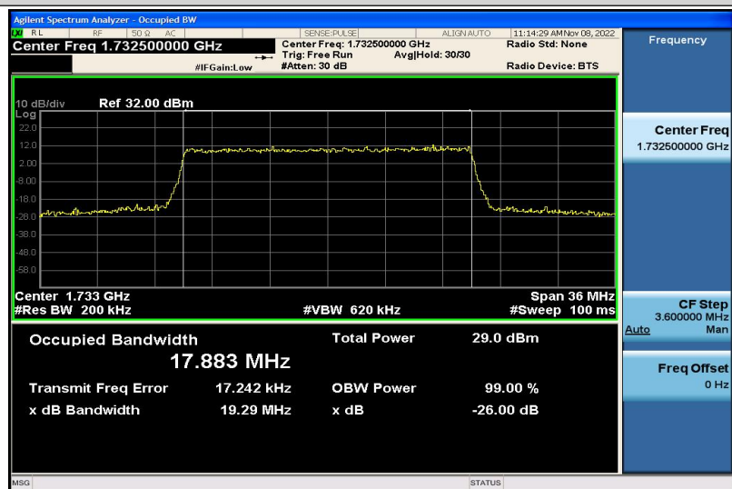
Band4-20MHz-QPSK-20175-100RB#0-17.883
