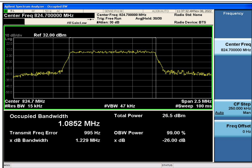
Band5-1.4MHz-16QAM-20407-6RB#0-1.0852
