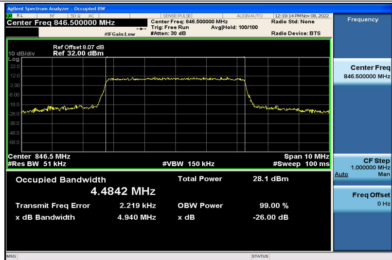
Band5-5MHz-16QAM-20625-25RB#0-4.4842
