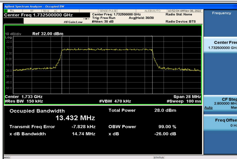
Band4-15MHz-16QAM-20175-75RB#0-13.432
