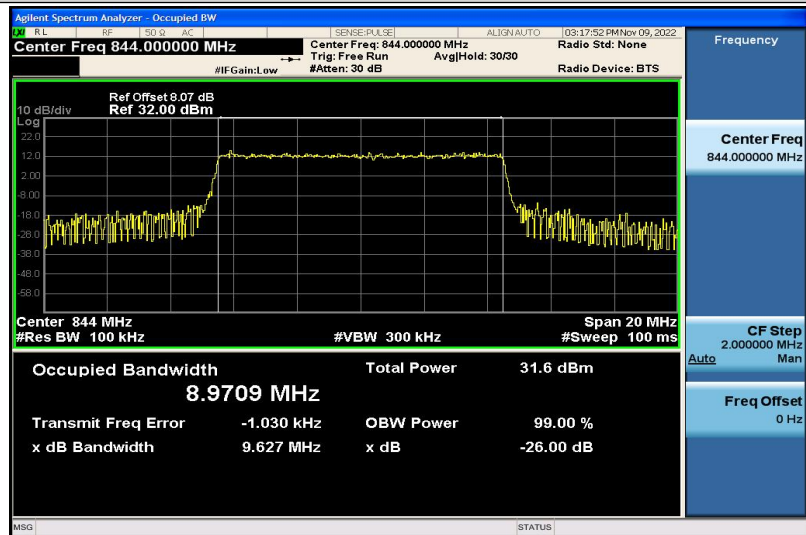
Band5-10MHz-QPSK-20600-50RB#0-8.9709
