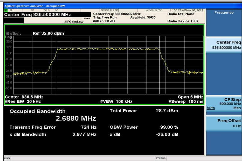
Band5-3MHz-QPSK-20525-15RB#0-2.6880
