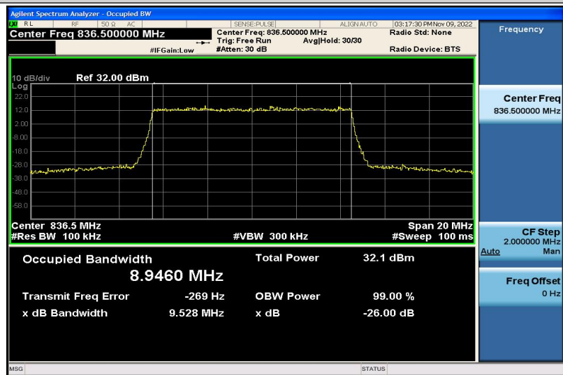
Band5-10MHz-QPSK-20525-50RB#0-8.9460
