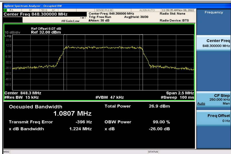
Band5-1.4MHz-16QAM-20643-6RB#0-1.0807
