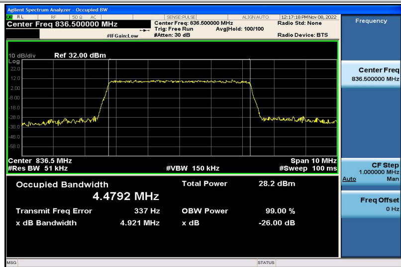
Band5-5MHz-16QAM-20525-25RB#0-4.4792
