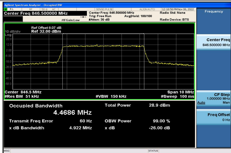
Band5-5MHz-QPSK-20625-25RB#0-4.4686
