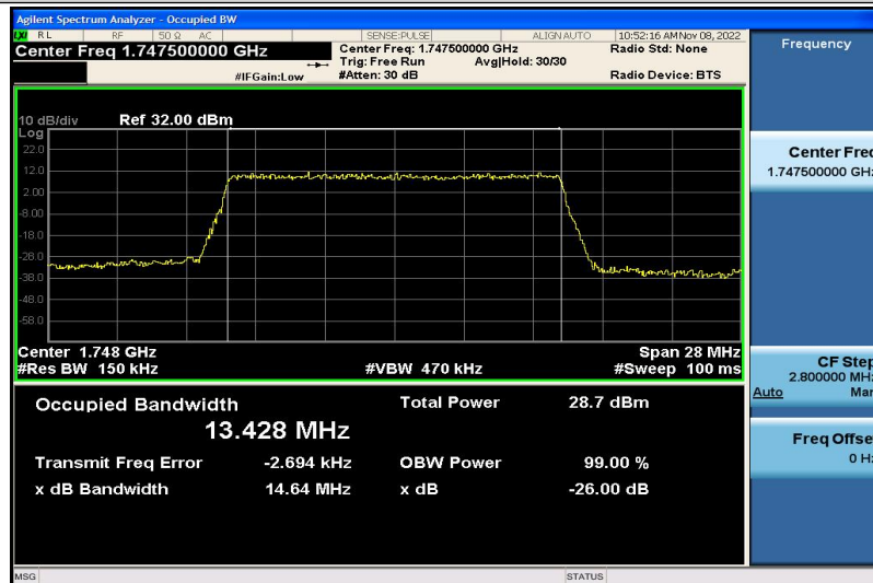
Band4-15MHz-QPSK-20325-75RB#0-13.428
