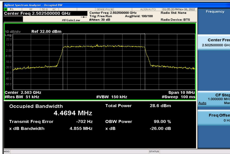
Band7-5MHz-16QAM-20775-25RB#0-4.4694
