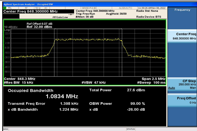
Band5-1.4MHz-QPSK-20643-6RB#0-1.0834
