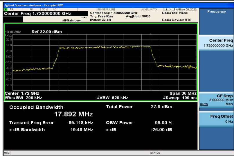
Band4-20MHz-16QAM-20050-100RB#0-17.892
