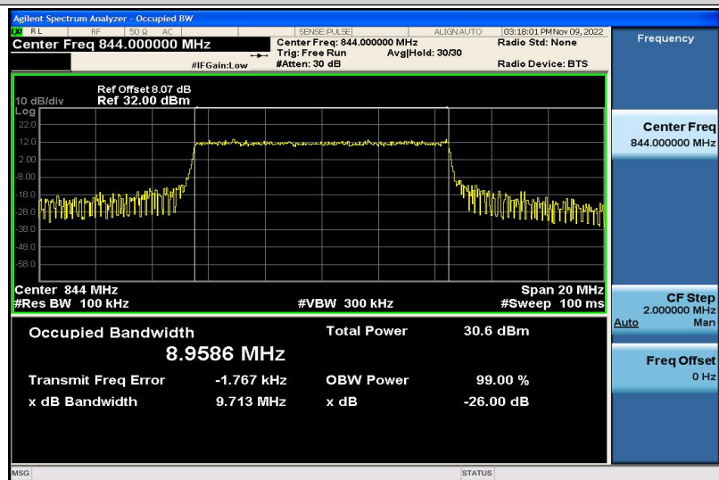
Band5-10MHz-16QAM-20600-50RB#0-8.9586
