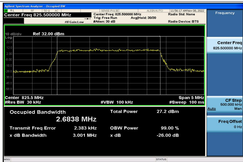
Band5-3MHz-16QAM-20415-15RB#0-2.6838
