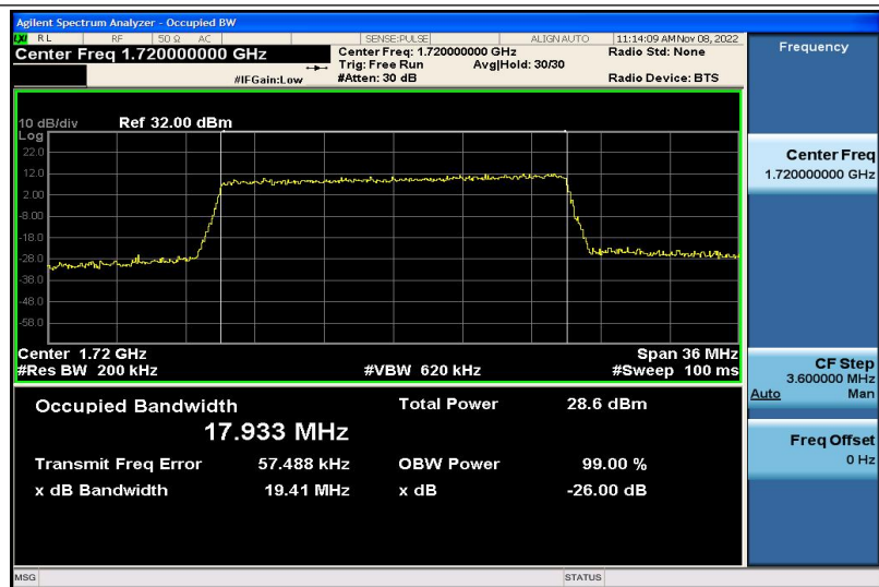
Band4-20MHz-QPSK-20050-100RB#0-17.933
