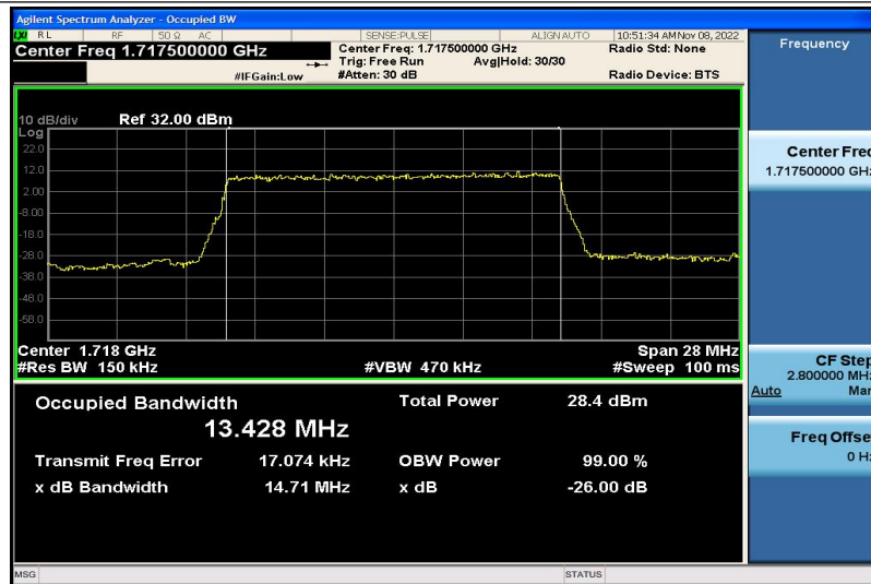
Band4-15MHz-QPSK-20025-75RB#0-13.428
