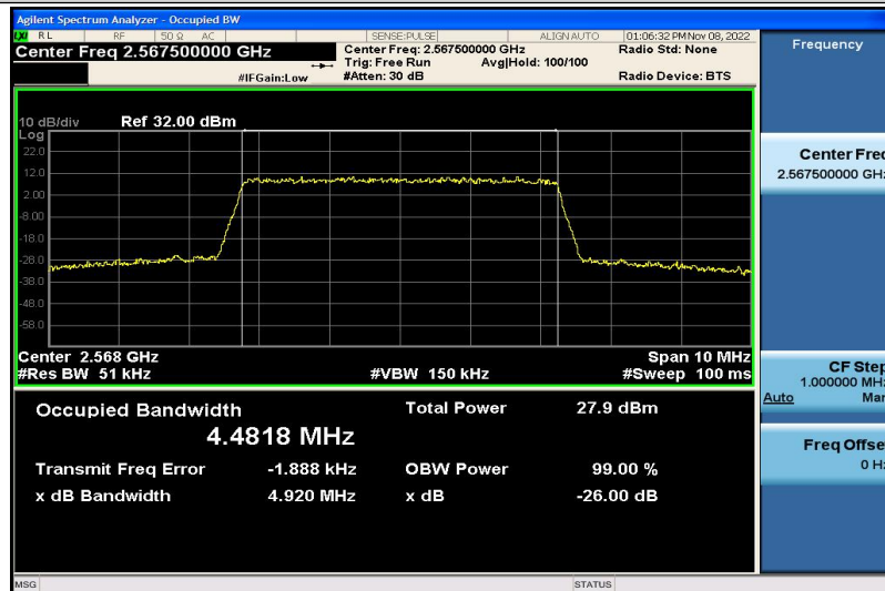
Band7-5MHz-16QAM-21425-25RB#0-4.4818
