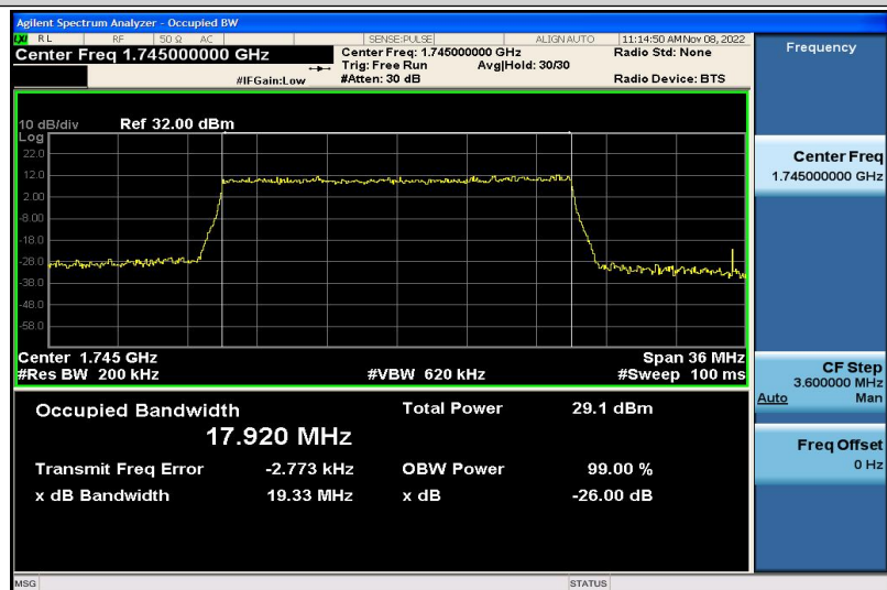
Band4-20MHz-QPSK-20300-100RB#0-17.920
