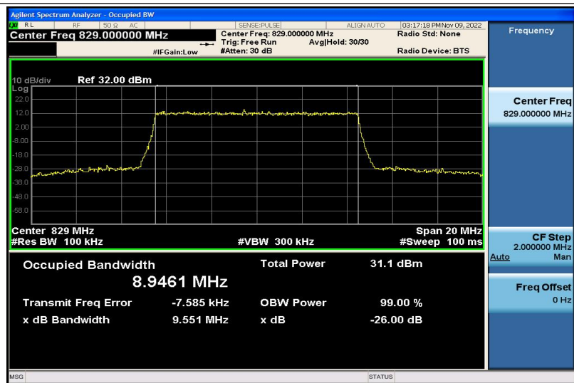
Band5-10MHz-16QAM-20450-50RB#0-8.9461
