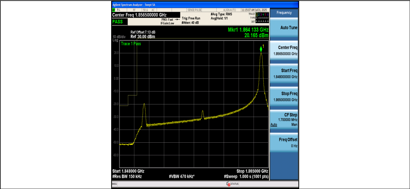
Band2_15MHz_QPSK_18675_1RB#74
