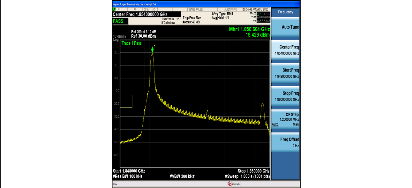
Band2_10MHz_16QAM_18650_1RB#0
