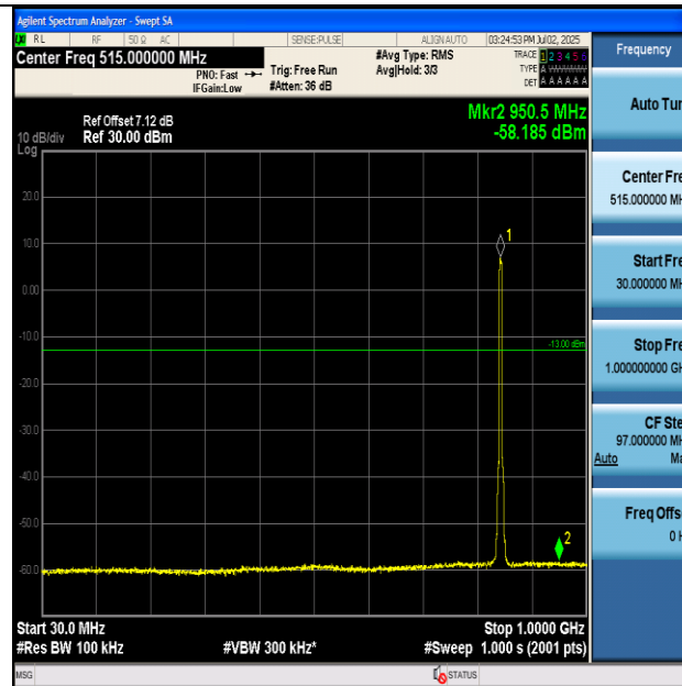
Band5-4233-30~1000MHz-PASS
