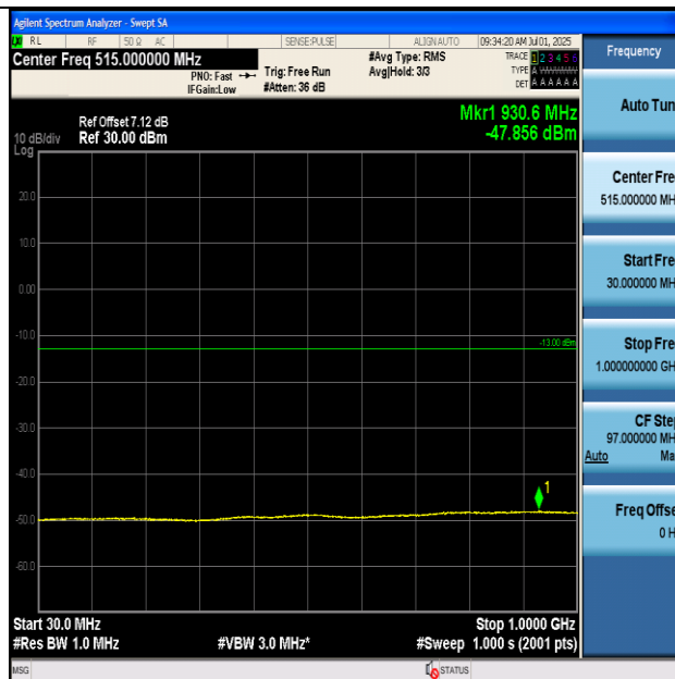
Band2-9400-30~1000MHz-PASS
