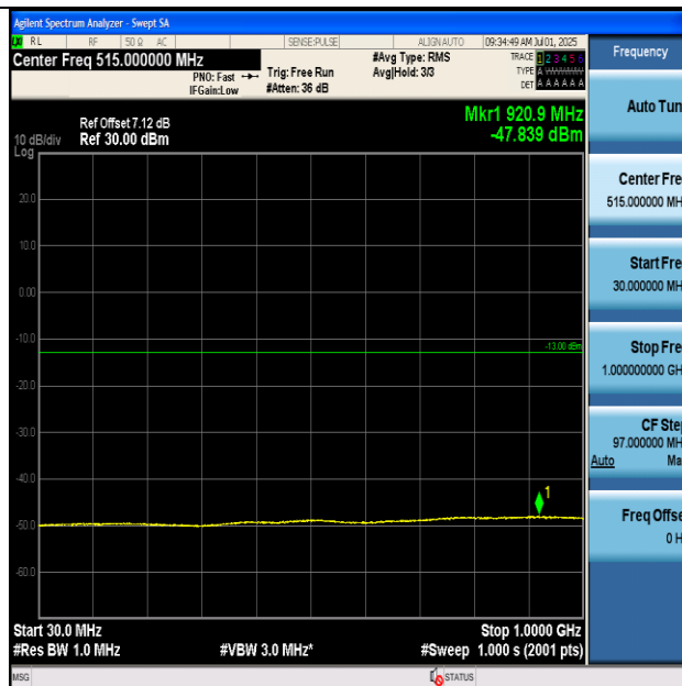
Band2-9538-30~1000MHz-PASS
