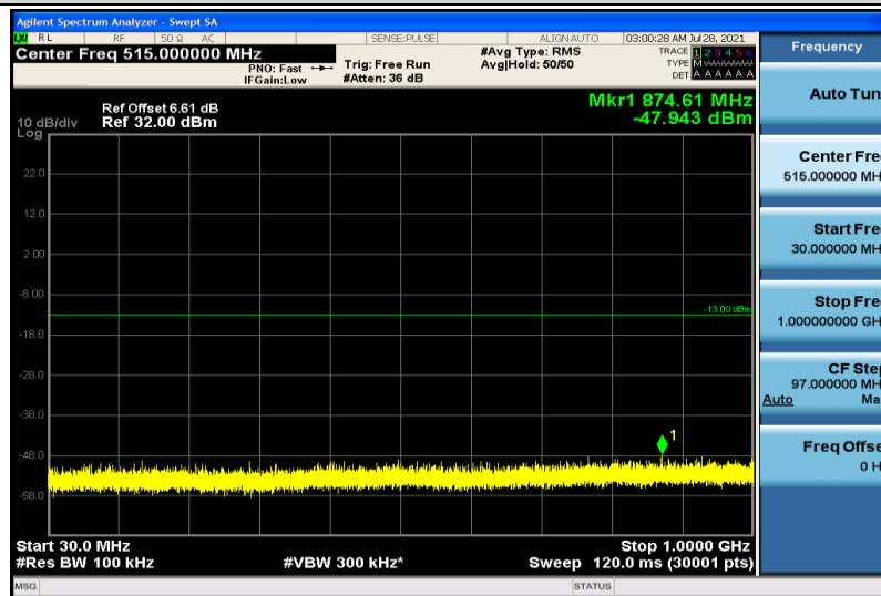
Band4-10MHz-QPSK-20350-1RB#0-30~1000MHz
