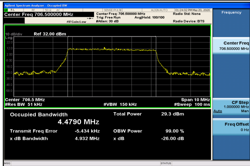
Band17-5MHz-16QAM-23755-25RB#0-4.4790
