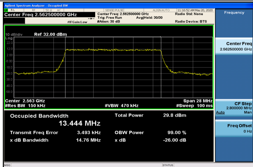
Band7-15MHz-QPSK-21375-75RB#0-13.444
