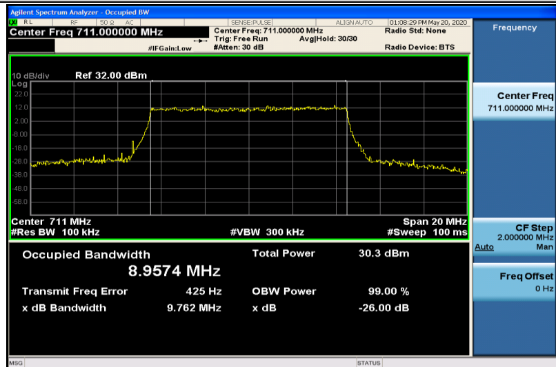
Band12-10MHz-QPSK-23130-50RB#0-8.9574
