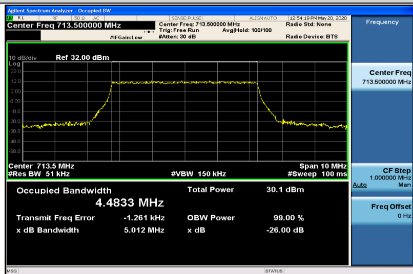
Band12-5MHz-QPSK-23155-25RB#0-4.4833
