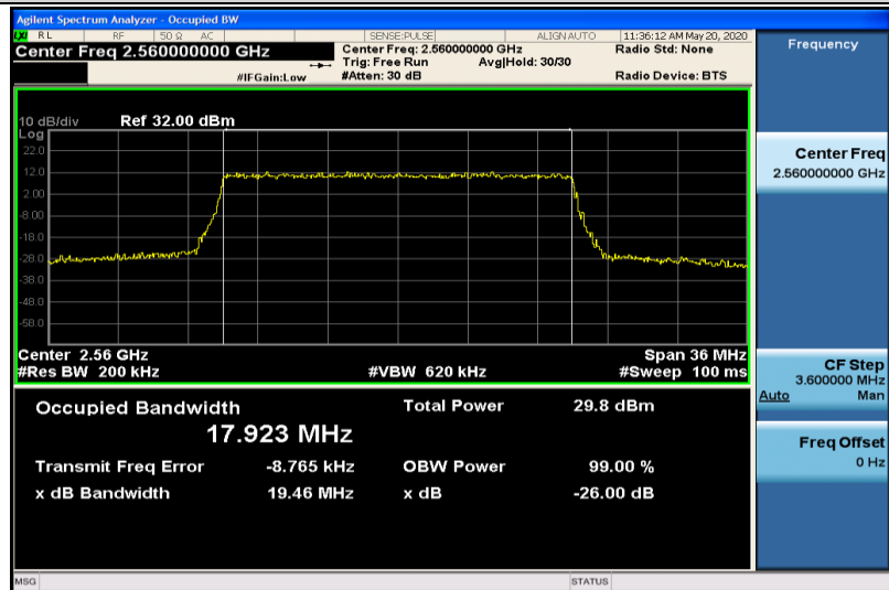
Band7-20MHz-QPSK-21350-100RB#0-17.923
