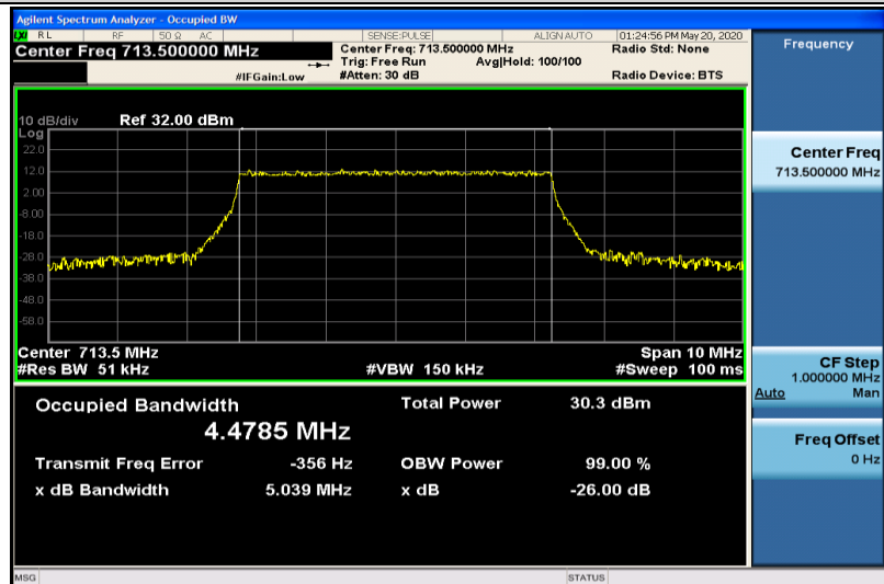
Band17-5MHz-QPSK-23825-25RB#0-4.4785
