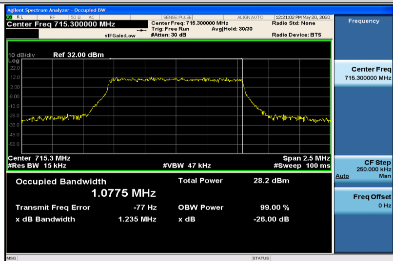
Band12-1.4MHz-16QAM-23173-6RB#0-1.0775
