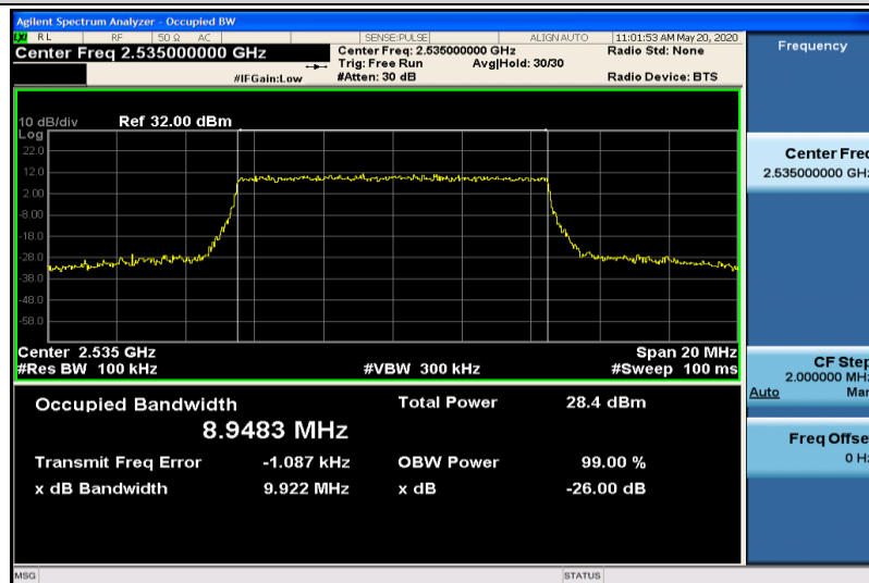
Band7-10MHz-16QAM-21100-50RB#0-8.9483
