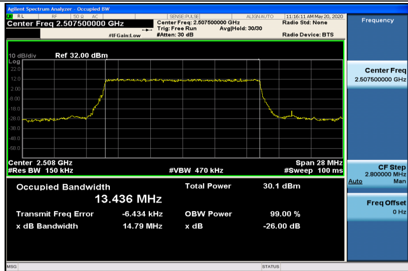
Band7-15MHz-QPSK-20825-75RB#0-13.436
