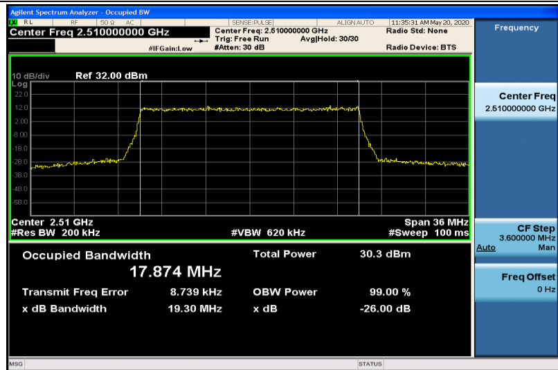
Band7-20MHz-QPSK-20850-100RB#0-17.874
