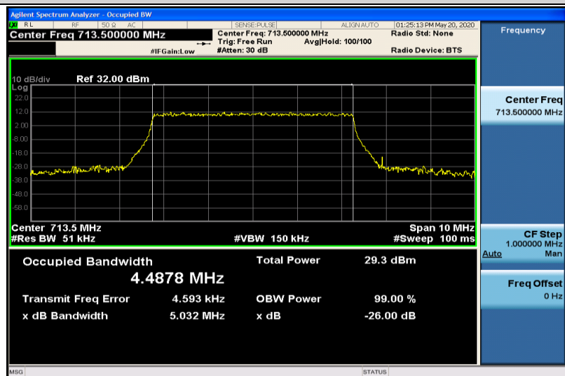
Band17-5MHz-16QAM-23825-25RB#0-4.4878
