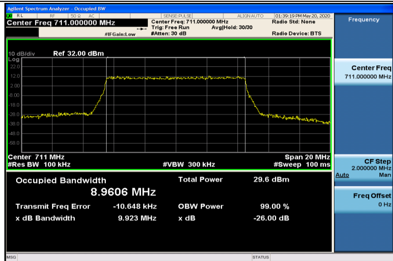
Band17-10MHz-16QAM-23800-50RB#0-8.9606
