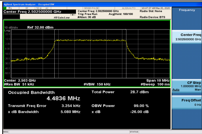
Band7-5MHz-16QAM-20775-25RB#0-4.4836
