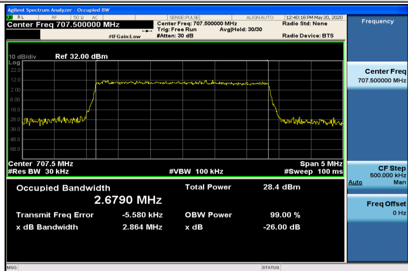
Band12-3MHz-16QAM-23095-15RB#0-2.6790
