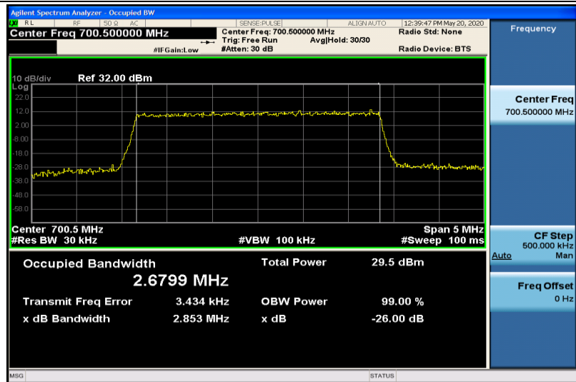
Band12-3MHz-QPSK-23025-15RB#0-2.6799
