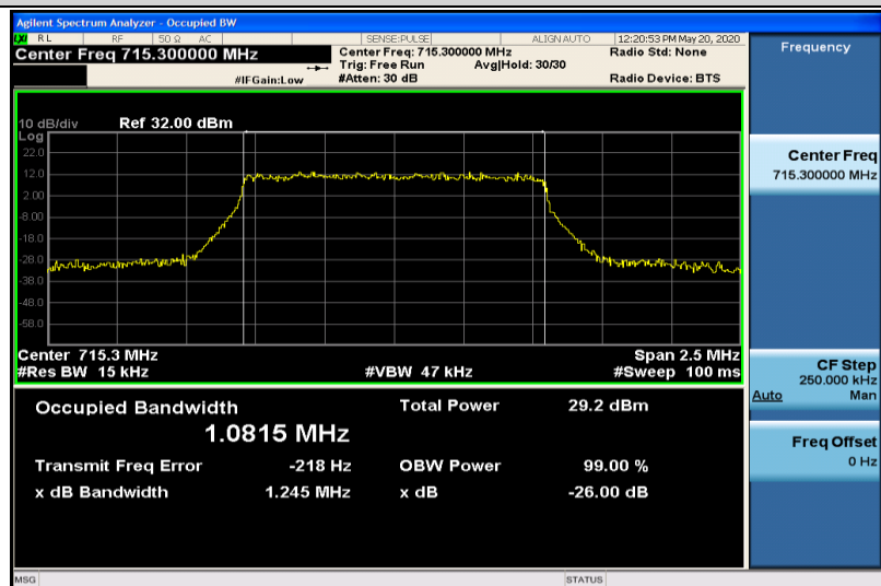
Band12-1.4MHz-QPSK-23173-6RB#0-1.0815
