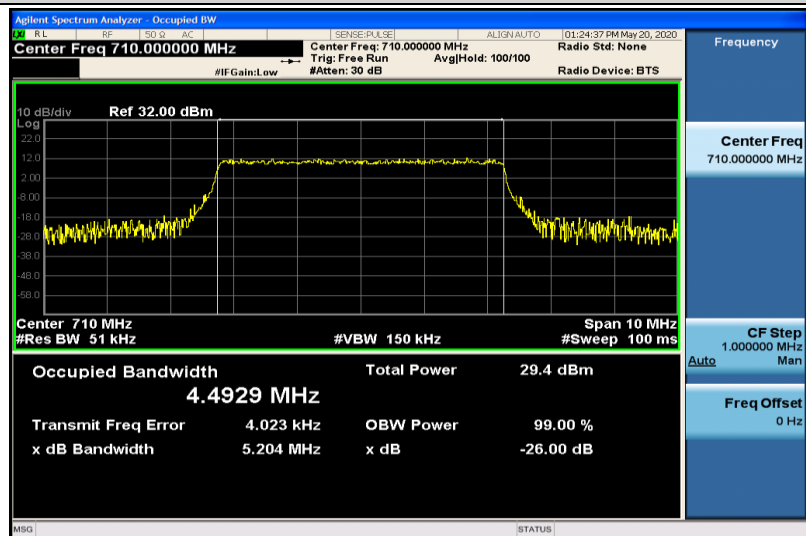
Band17-5MHz-16QAM-23790-25RB#0-4.4929
