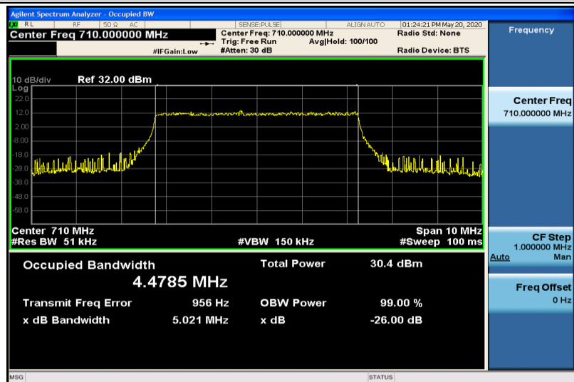
Band17-5MHz-QPSK-23790-25RB#0-4.4785
