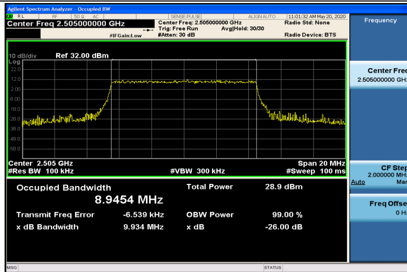
Band7-10MHz-16QAM-20800-50RB#0-8.9454
