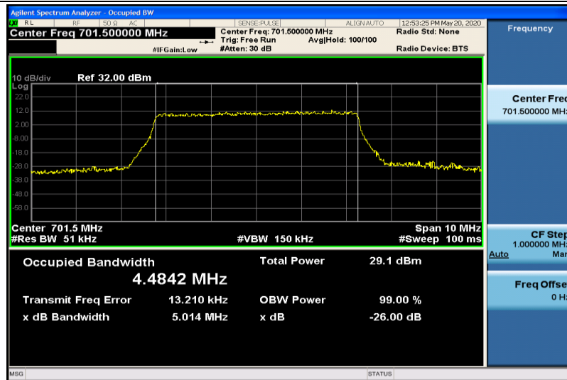
Band12-5MHz-16QAM-23035-25RB#0-4.4842
