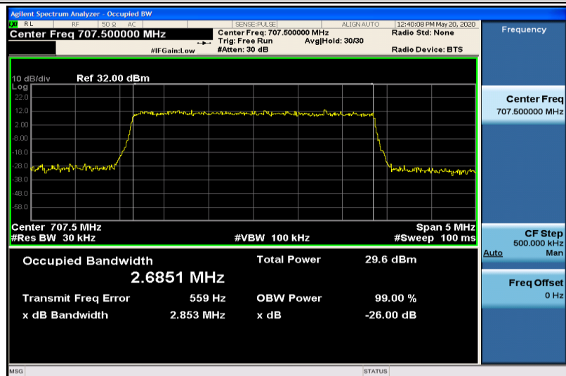
Band12-3MHz-QPSK-23095-15RB#0-2.6851
