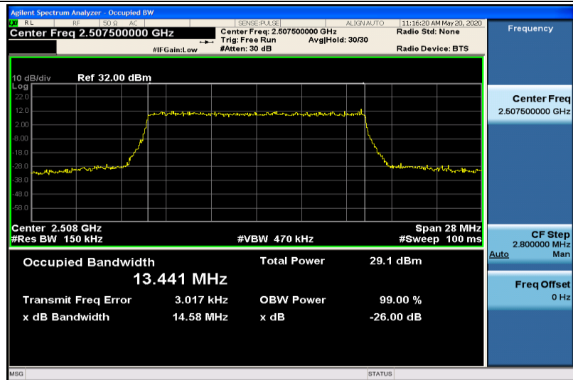
Band7-15MHz-16QAM-20825-75RB#0-13.441
