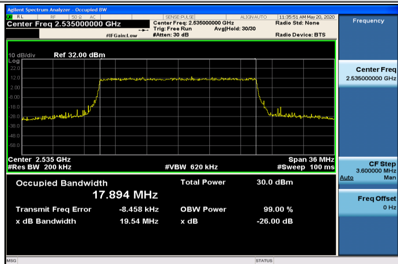
Band7-20MHz-QPSK-21100-100RB#0-17.894
