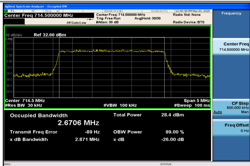
Band12-3MHz-16QAM-23165-15RB#0-2.6706
