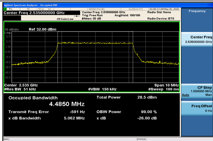
Band7-5MHz-16QAM-21100-25RB#0-4.4850
