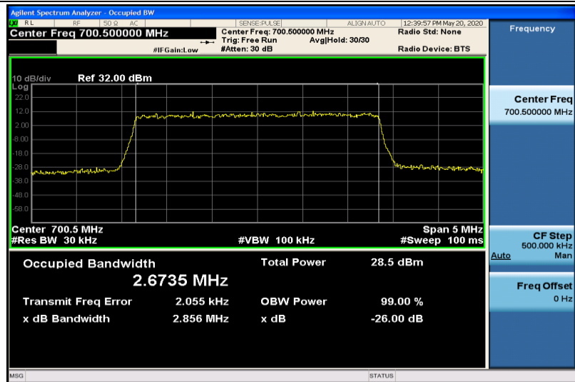
Band12-3MHz-16QAM-23025-15RB#0-2.6735
