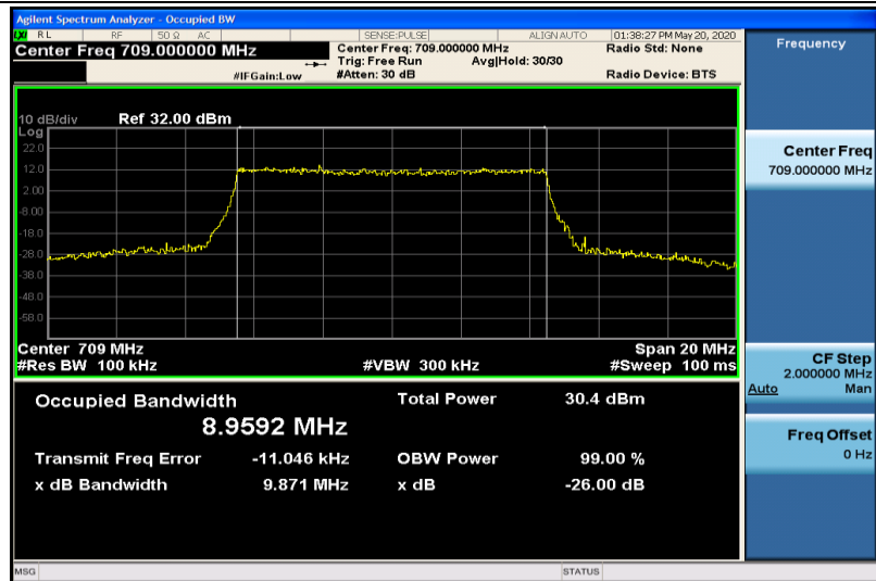
Band17-10MHz-QPSK-23780-50RB#0-8.9592
