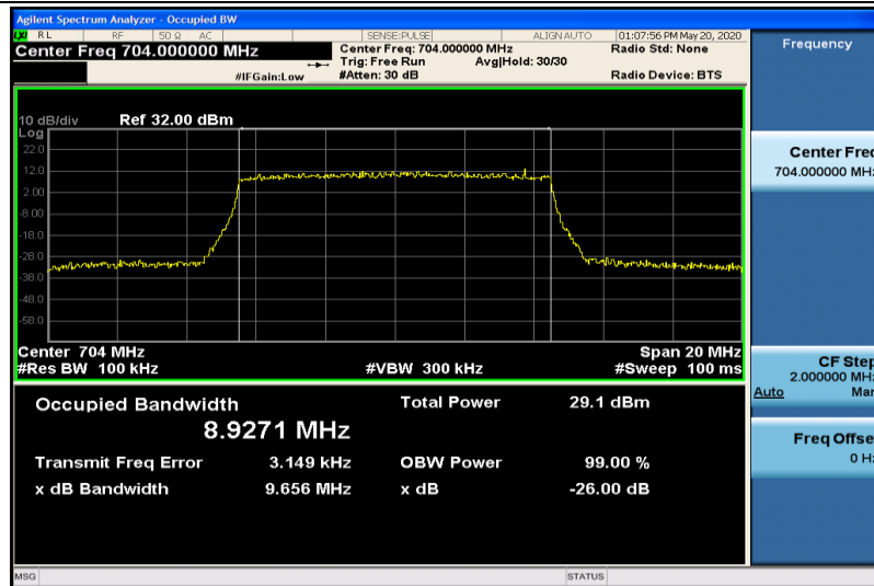
Band12-10MHz-16QAM-23060-50RB#0-8.9271
