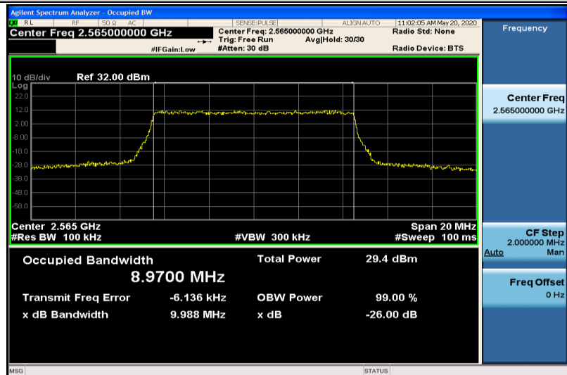
Band7-10MHz-QPSK-21400-50RB#0-8.9700
