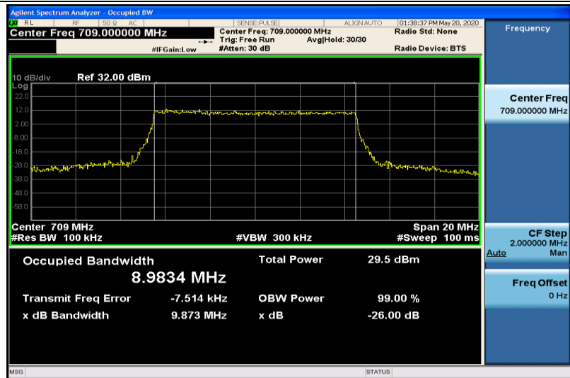
Band17-10MHz-16QAM-23780-50RB#0-8.9834
