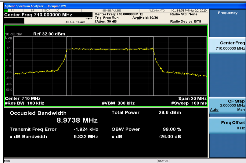
Band17-10MHz-16QAM-23790-50RB#0-8.9738
