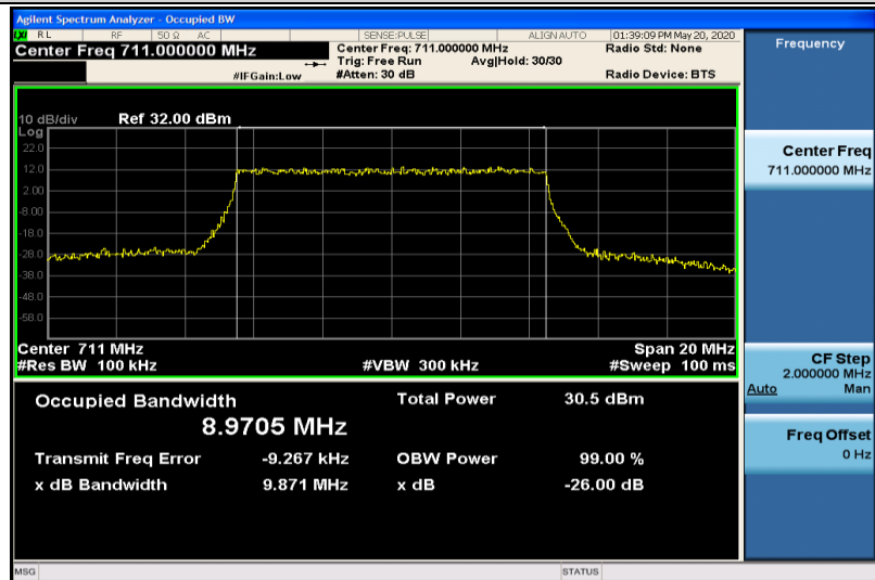
Band17-10MHz-QPSK-23800-50RB#0-8.9705
