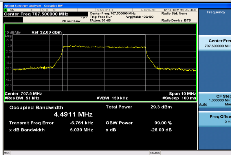
Band12-5MHz-16QAM-23095-25RB#0-4.4911
