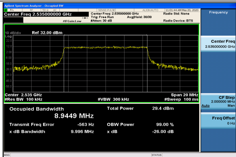
Band7-10MHz-QPSK-21100-50RB#0-8.9449
