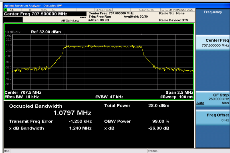
Band12-1.4MHz-16QAM-23095-6RB#0-1.0797
