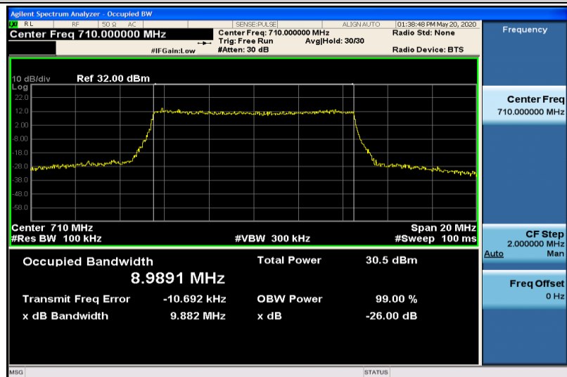
Band17-10MHz-QPSK-23790-50RB#0-8.9891
