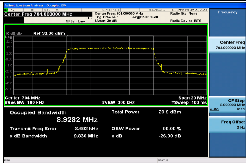
Band12-10MHz-QPSK-23060-50RB#0-8.9282
