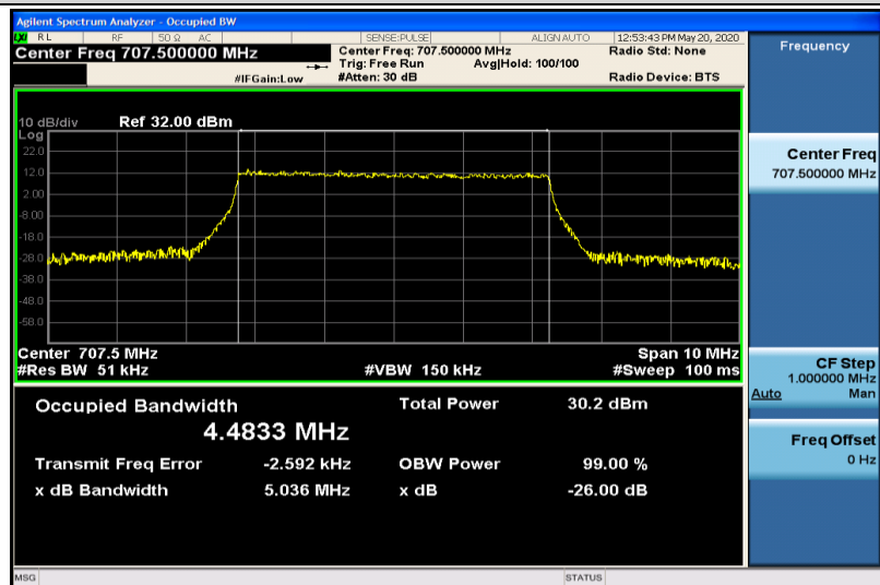
Band12-5MHz-QPSK-23095-25RB#0-4.4833
