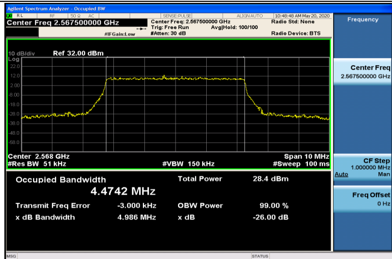
Band7-5MHz-16QAM-21425-25RB#0-4.4742
