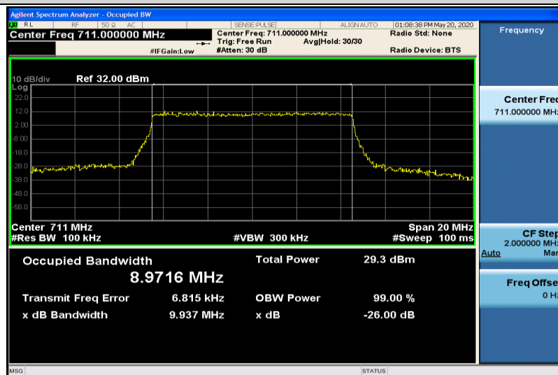
Band12-10MHz-16QAM-23130-50RB#0-8.9716
