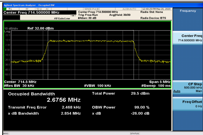
Band12-3MHz-QPSK-23165-15RB#0-2.6756
