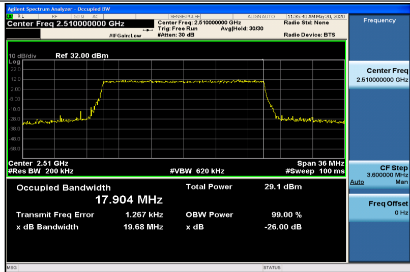
Band7-20MHz-16QAM-20850-100RB#0-17.904
