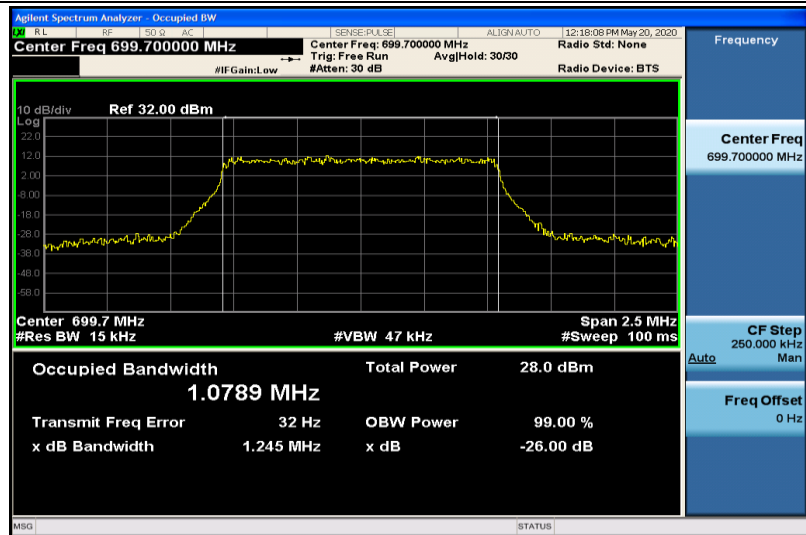
Band12-1.4MHz-16QAM-23017-6RB#0-1.0789
