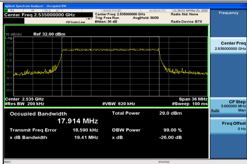
Band7-20MHz-16QAM-21100-100RB#0-17.914
