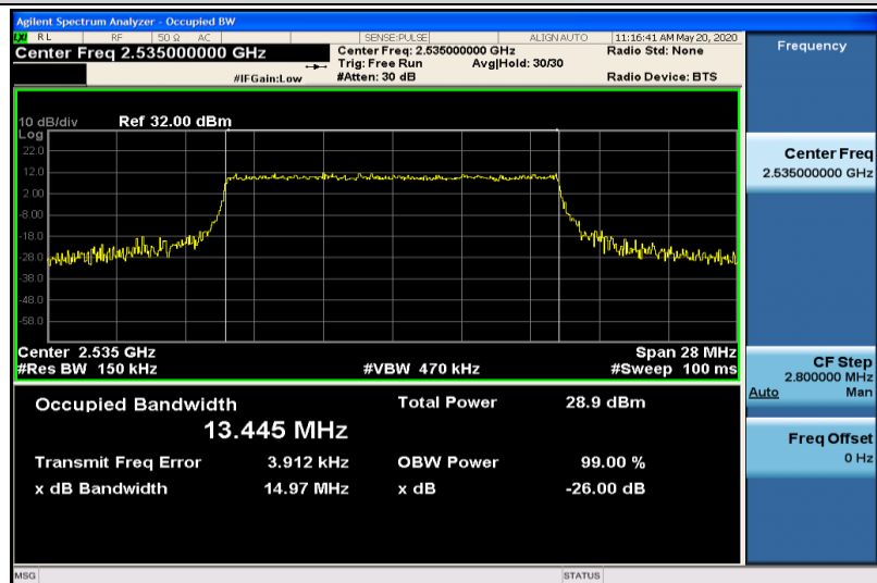
Band7-15MHz-16QAM-21100-75RB#0-13.445
