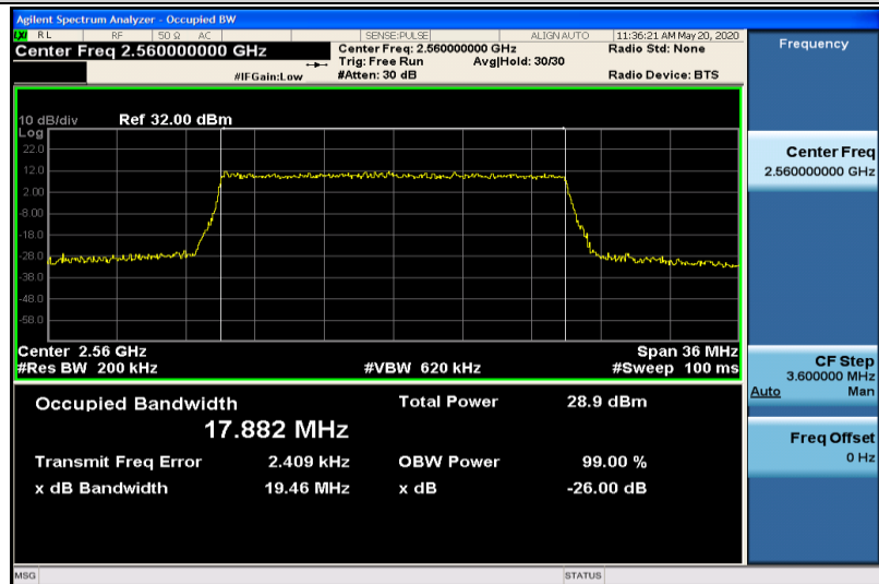
Band7-20MHz-16QAM-21350-100RB#0-17.882
