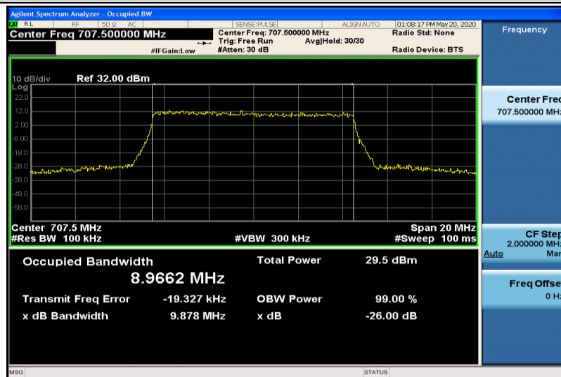
Band12-10MHz-16QAM-23095-50RB#0-8.9662
