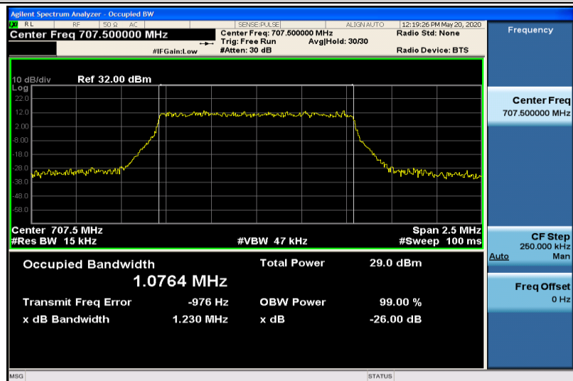
Band12-1.4MHz-QPSK-23095-6RB#0-1.0764
