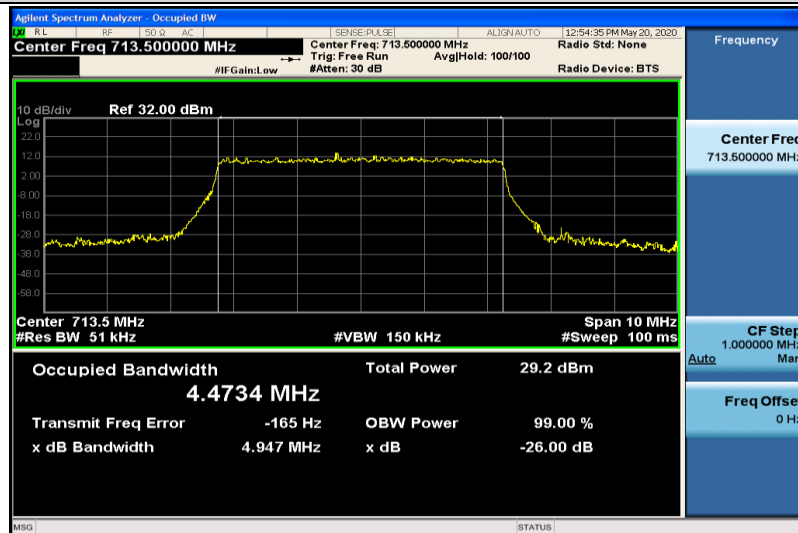
Band12-5MHz-16QAM-23155-25RB#0-4.4734
