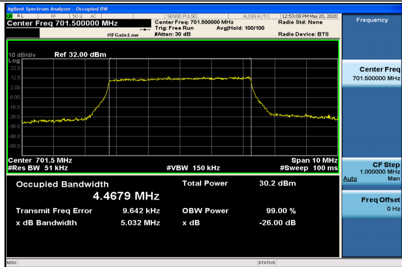
Band12-5MHz-QPSK-23035-25RB#0-4.4679
