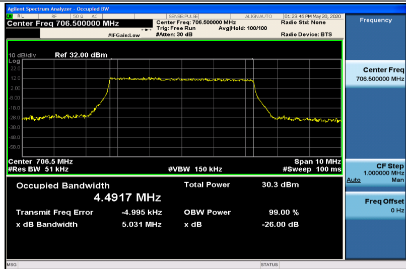
Band17-5MHz-QPSK-23755-25RB#0-4.4917
