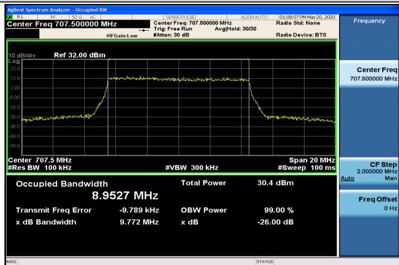
Band12-10MHz-QPSK-23095-50RB#0-8.9527
