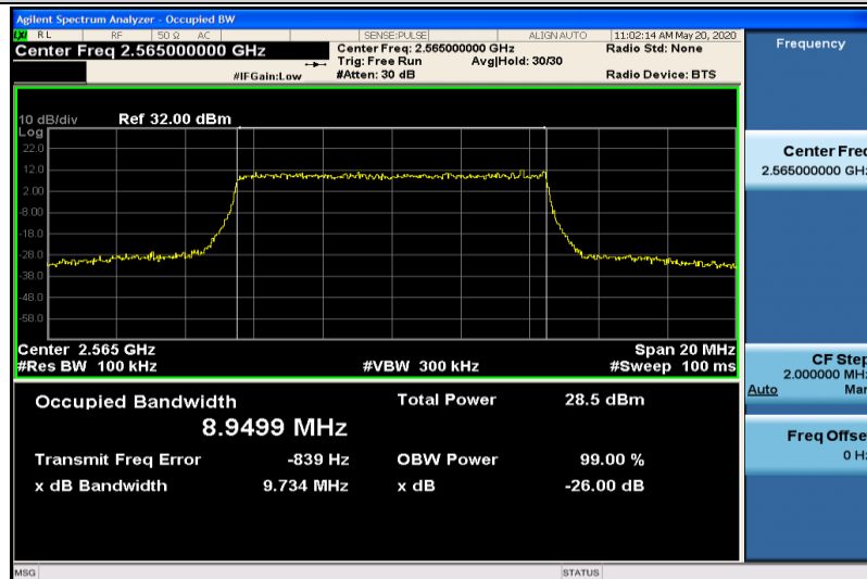
Band7-10MHz-16QAM-21400-50RB#0-8.9499
