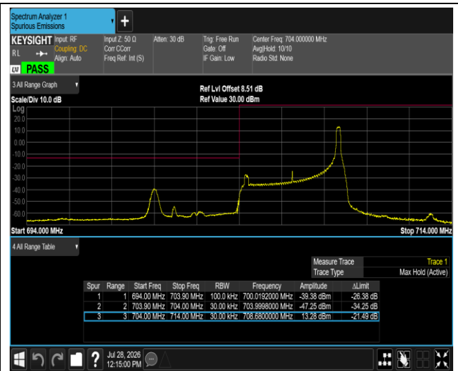
Band17-5MHz-16QAM-23825-1RB#0
