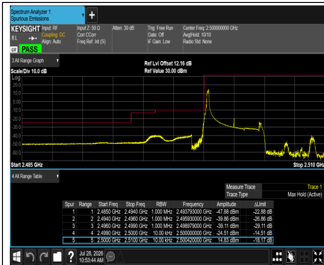
Band7-5MHz-16QAM-20775-25RB#0
