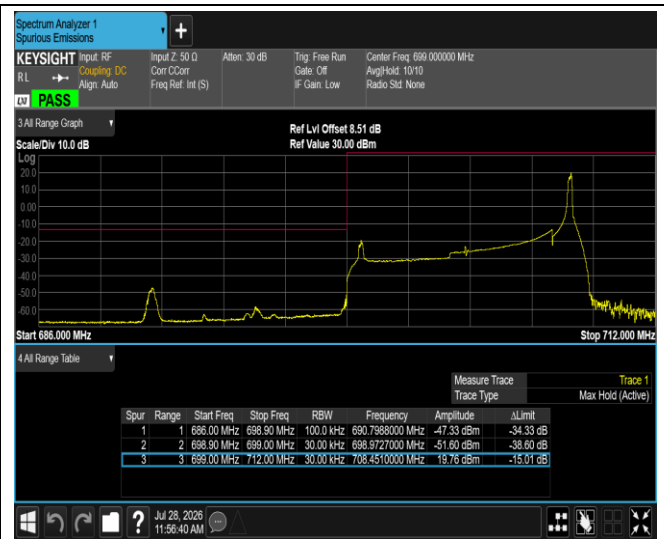
Band12-10MHz-QPSK-23130-1RB#0
