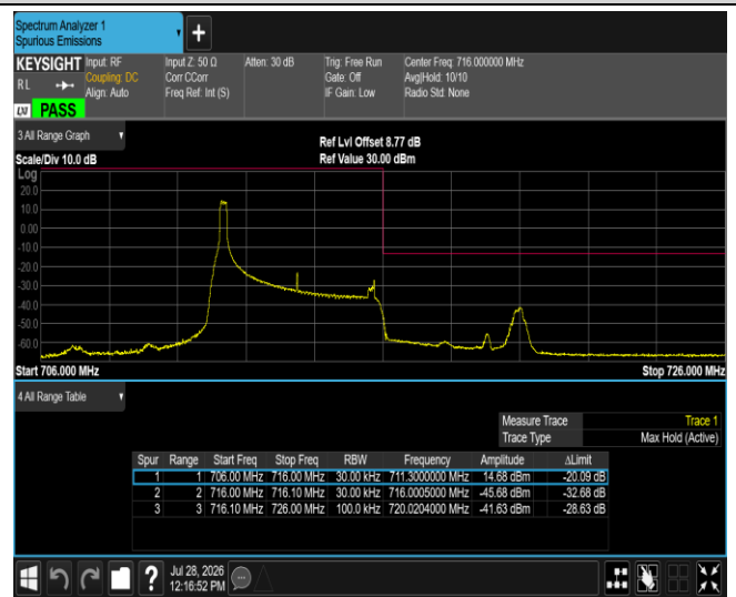
Band17-5MHz-QPSK-23825-25RB#0
