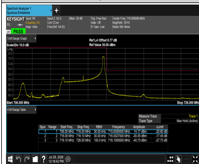
Band17-10MHz-QPSK-23780-1RB#0
