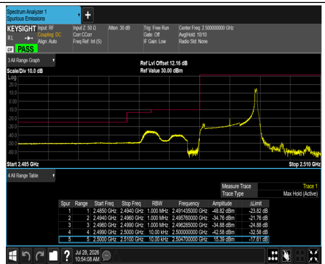
Band7-5MHz-16QAM-21425-1RB#0
