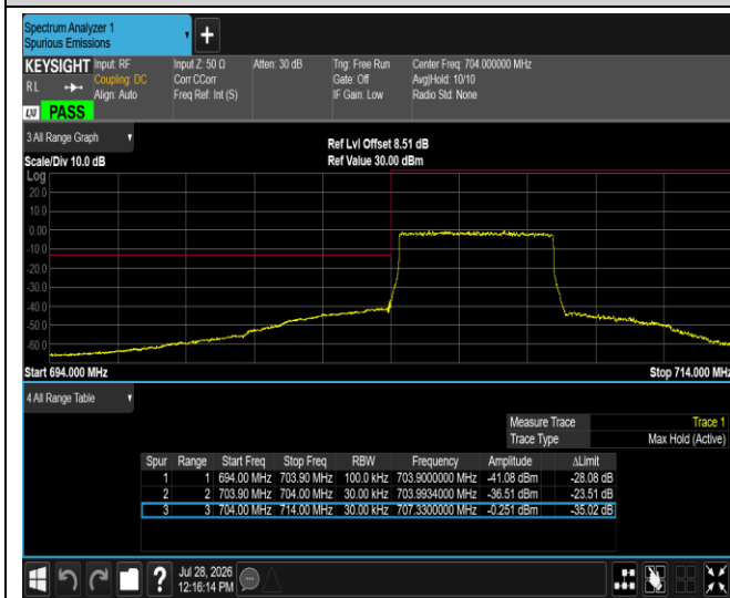
Band17-5MHz-16QAM-23825-1RB#24
