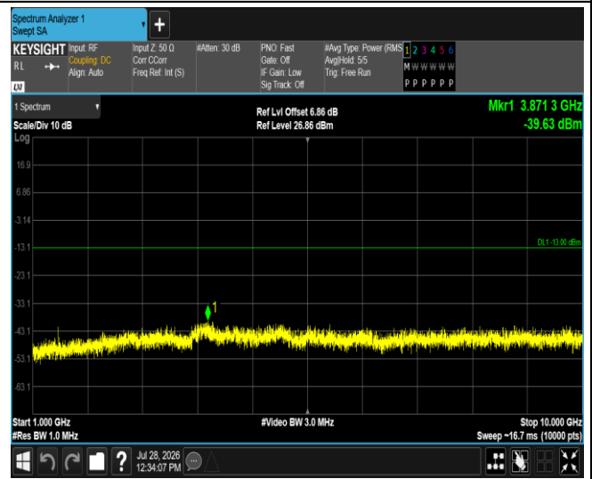
Band17-10MHz-16QAM-23780-1RB#0-Range2:1000~10000MHz
