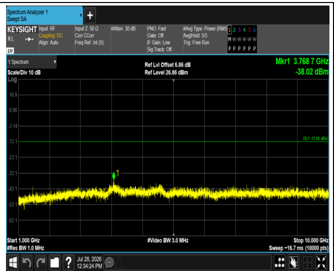
Band17-10MHz-QPSK-23800-1RB#0-Range2:1000~10000MHz
