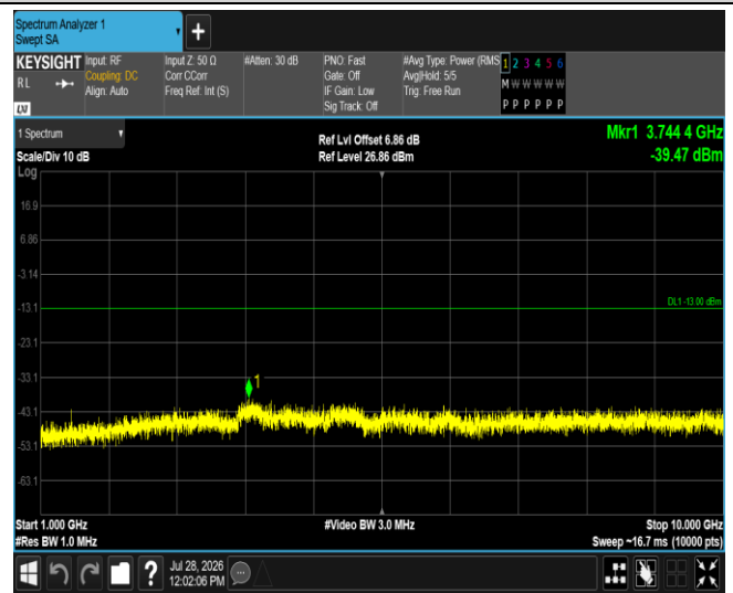
Band12-10MHz-16QAM-23130-1RB#0-Range2:1000~10000MHz
