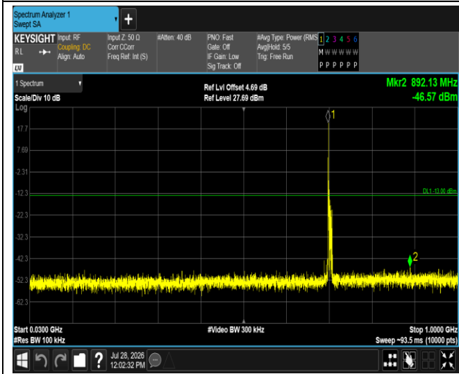
Band12-10MHz-16QAM-23130-1RB#0-Range1:30~1000MHz
