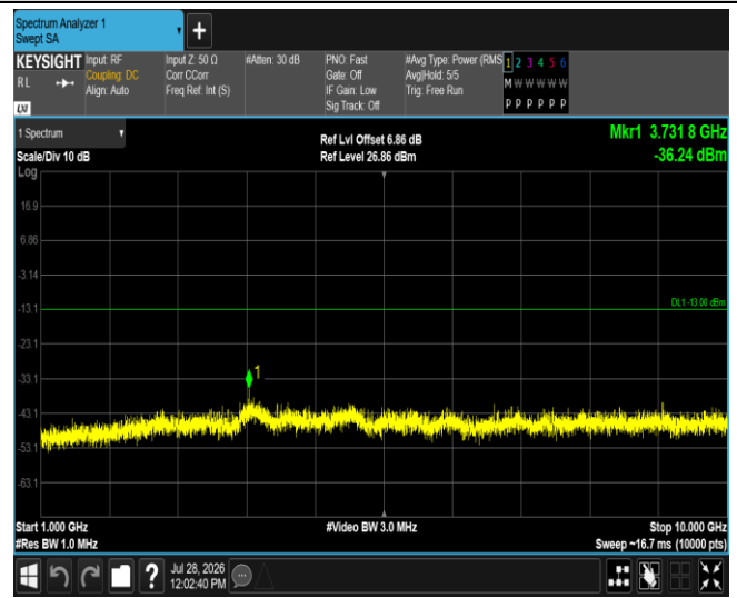
Band12-10MHz-16QAM-23130-1RB#0-Range2:1000~10000MHz
