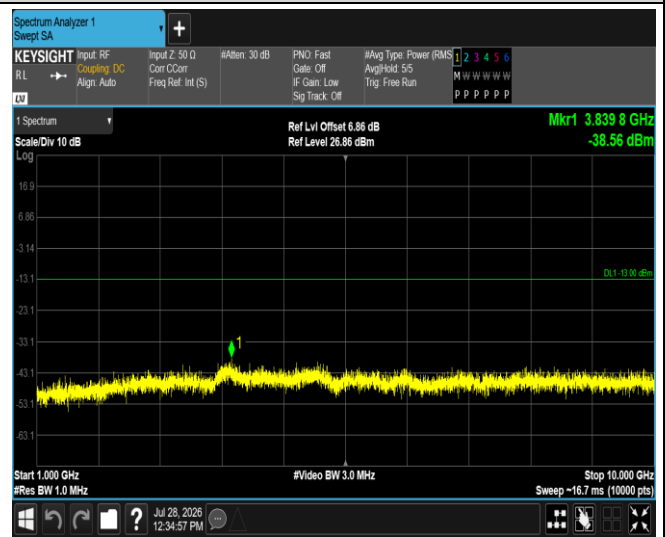
Band17-10MHz-16QAM-23780-1RB#0-Range2:1000~10000MHz
