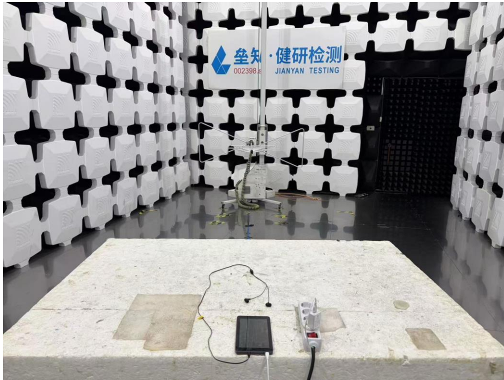
Star9 4G Radiated Spurious Emission Below 1GHz
