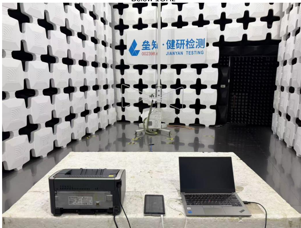
The Leader Tab9 4G Radiated Spurious Emission Below 1GHz
