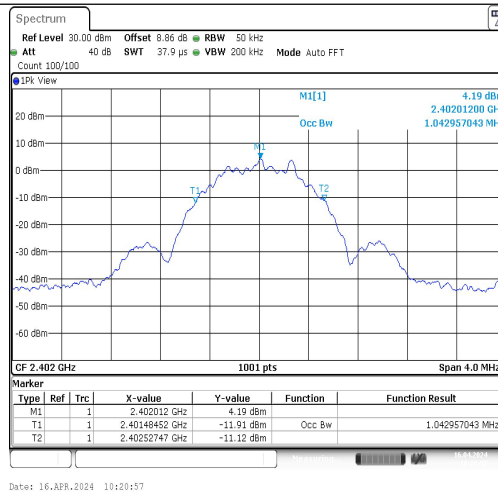
BLE_1M-Ant1-2402
