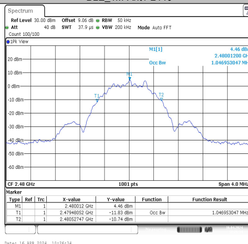
BLE_1M-Ant1-2480
