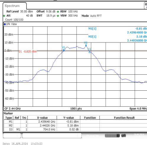
BLE_1M-Ant1-2440-PASS
