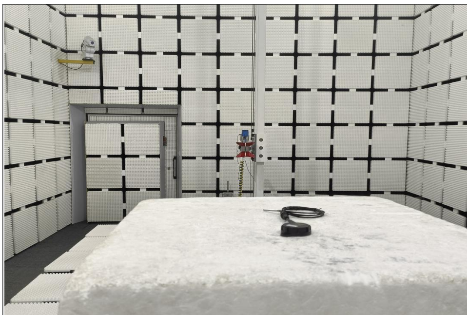
RADIATED EMISSION TEST (Above 1GHz)
