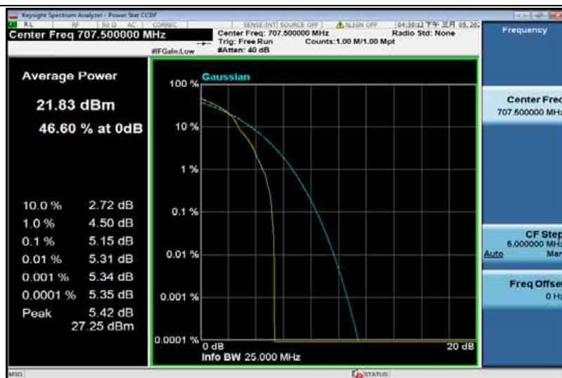
Band12-5MHz-16QAM-23095-25RB#0
