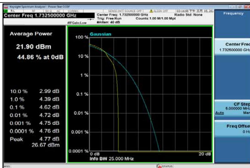
Band4-20MHz-16QAM-20175-100RB#0
