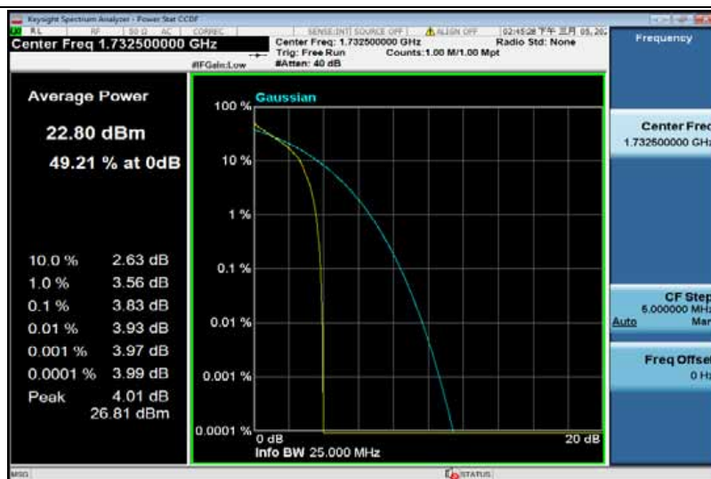
Band4-15MHz-QPSK-20175-75RB#0
