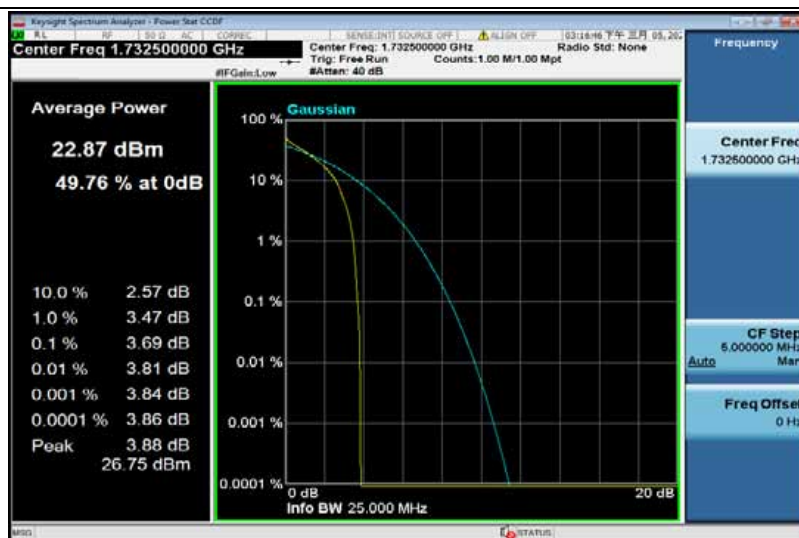
Band4-20MHz-QPSK-20175-100RB#0
