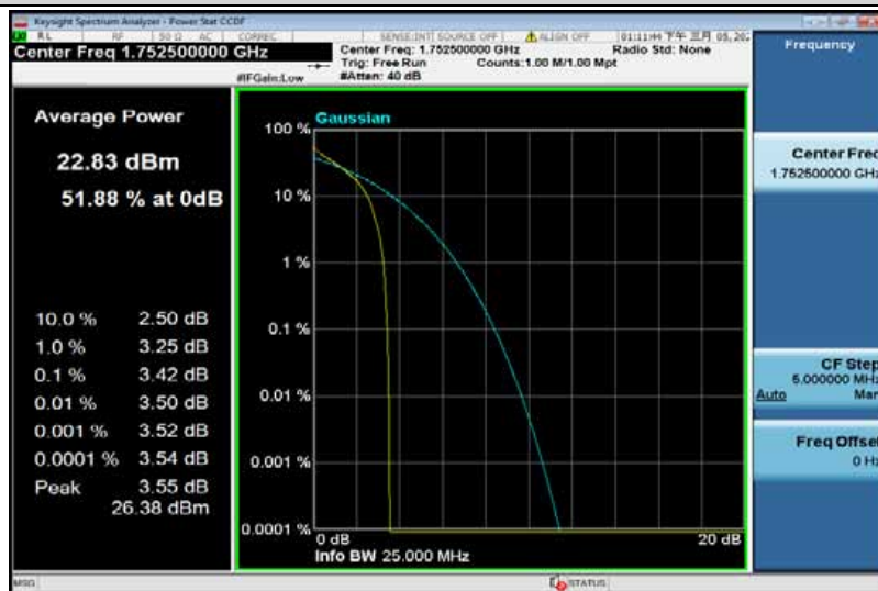
Band4-5MHz-QPSK-20375-25RB#0
