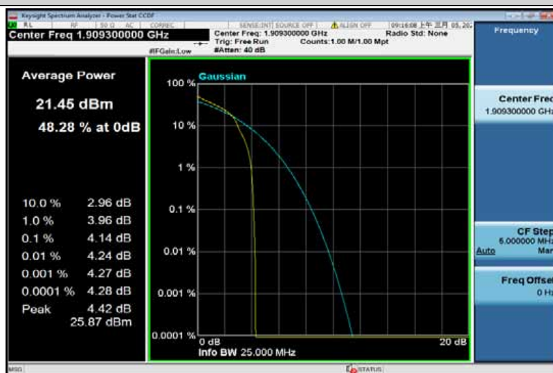
Band2-1.4MHz-16QAM-19193-6RB#0
