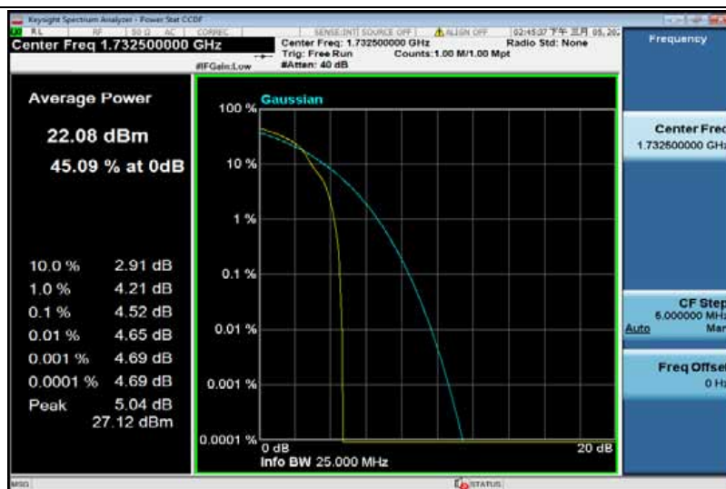
Band4-15MHz-16QAM-20175-75RB#0
