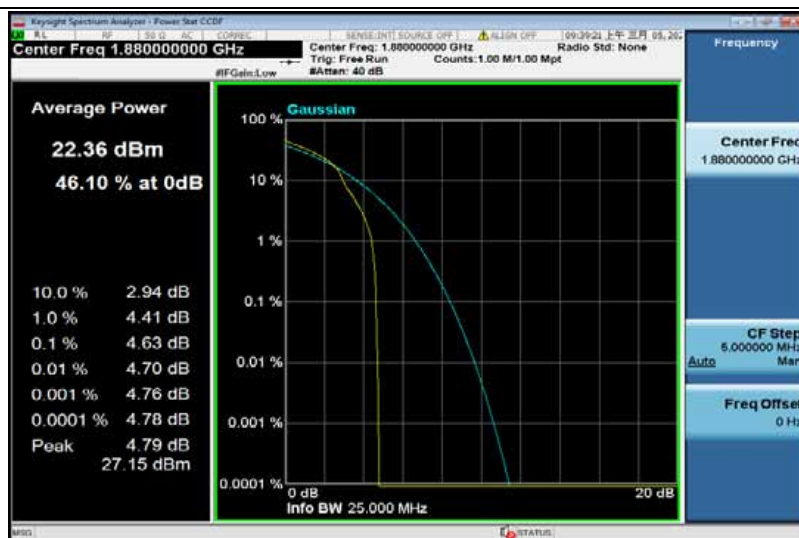
Band2-3MHz-16QAM-18900-15RB#0
