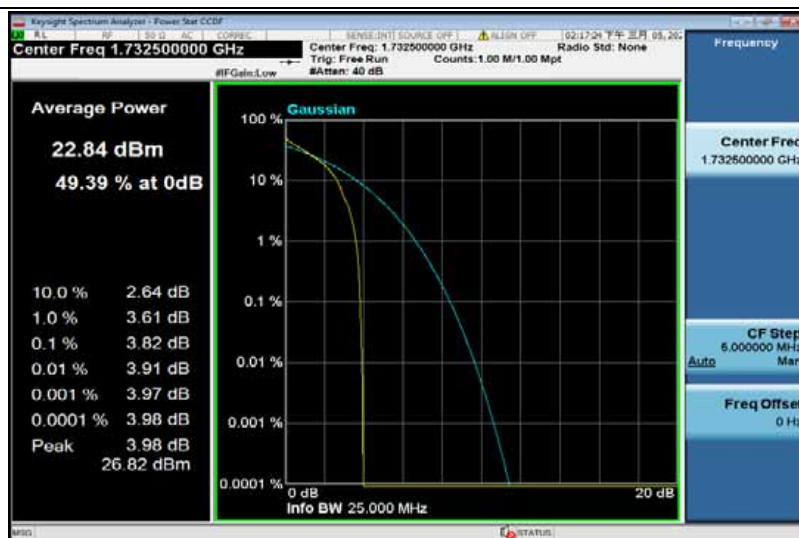
Band4-10MHz-QPSK-20175-50RB#0
