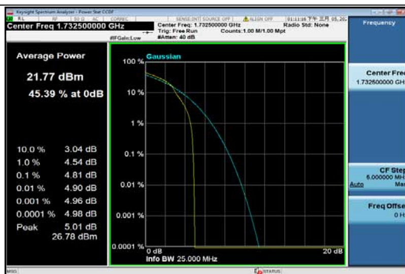
Band4-5MHz-16QAM-20175-25RB#0
