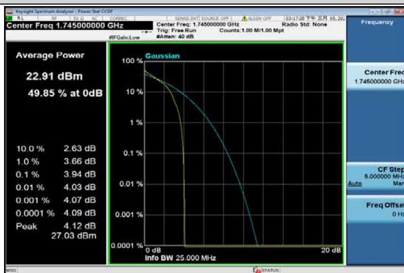
Band4-20MHz-QPSK-20300-100RB#0
