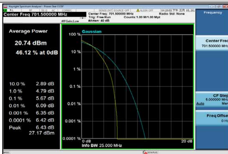
Band12-5MHz-16QAM-23095-1RB#0
