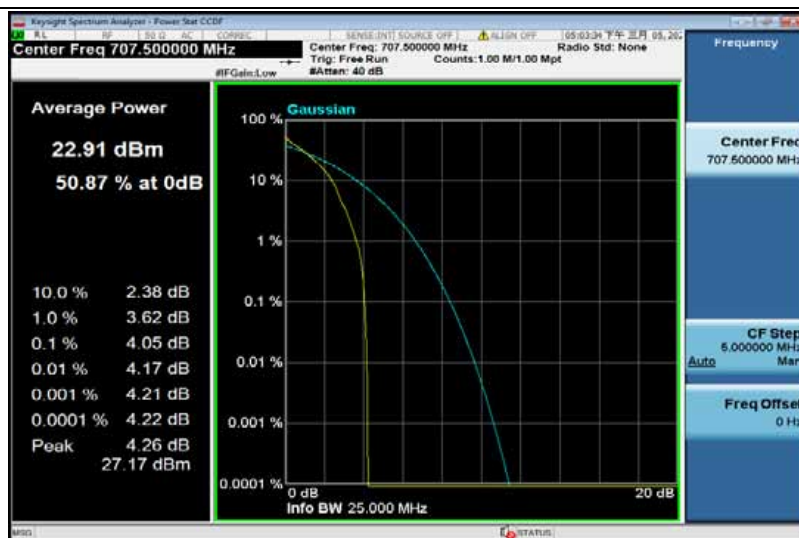
Band12-10MHz-QPSK-23095-50RB#0
