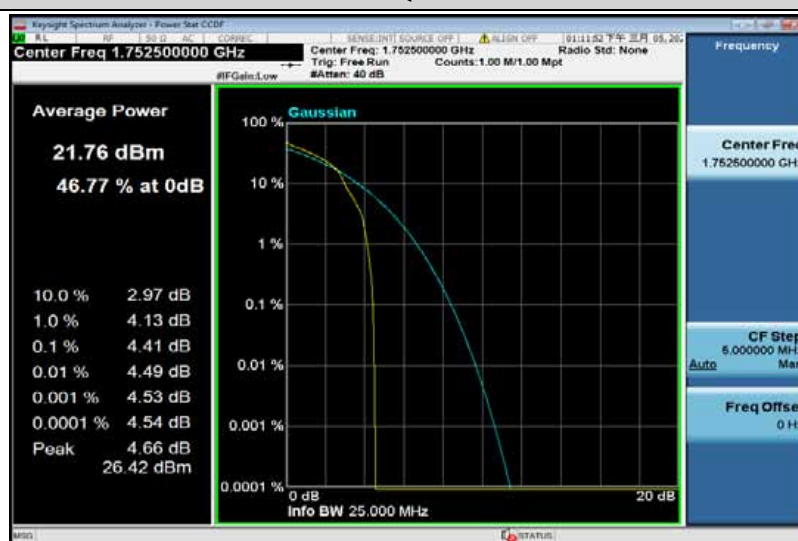
Band4-5MHz-16QAM-20375-25RB#0
