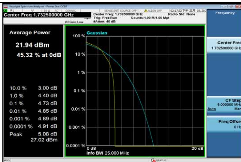
Band4-10MHz-16QAM-20175-50RB#0
