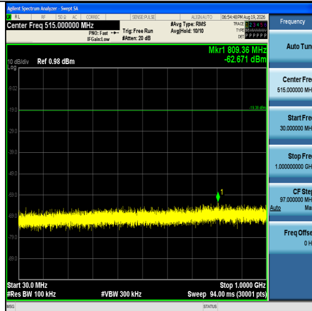
SRD-Ant1-2402-30~1000-PASS
