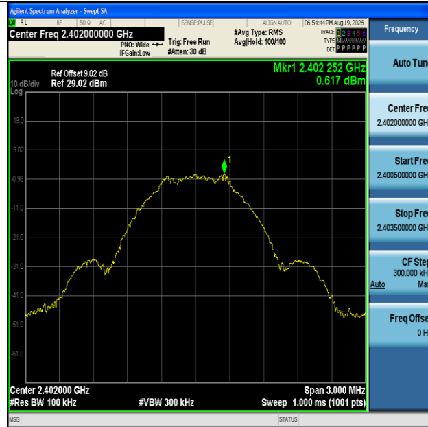
SRD-Ant1-2402-0~Reference-PASS
