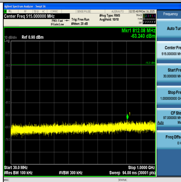
SRD-Ant1-2403-30~1000-PASS
